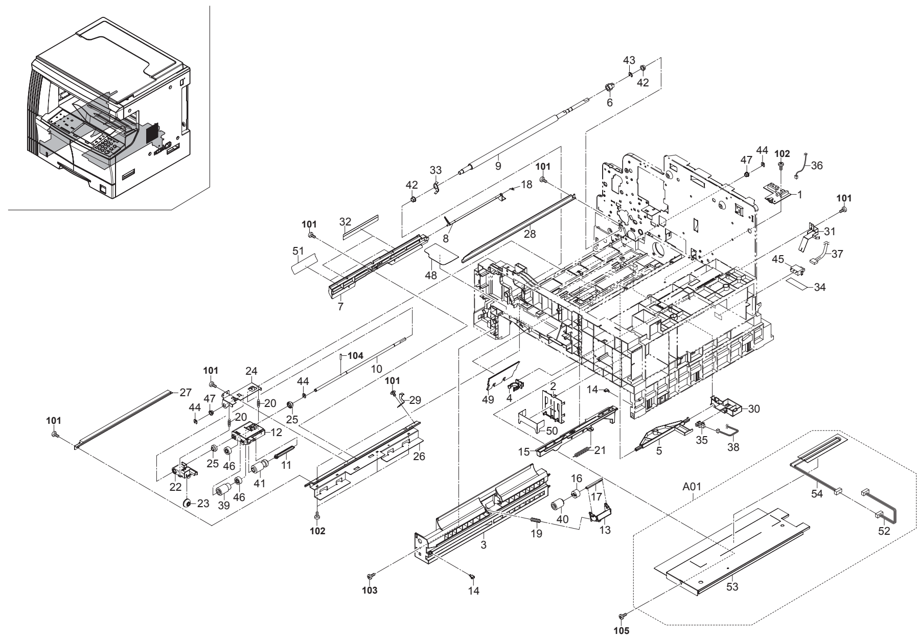
FIG. 5 Paper Feed-in
