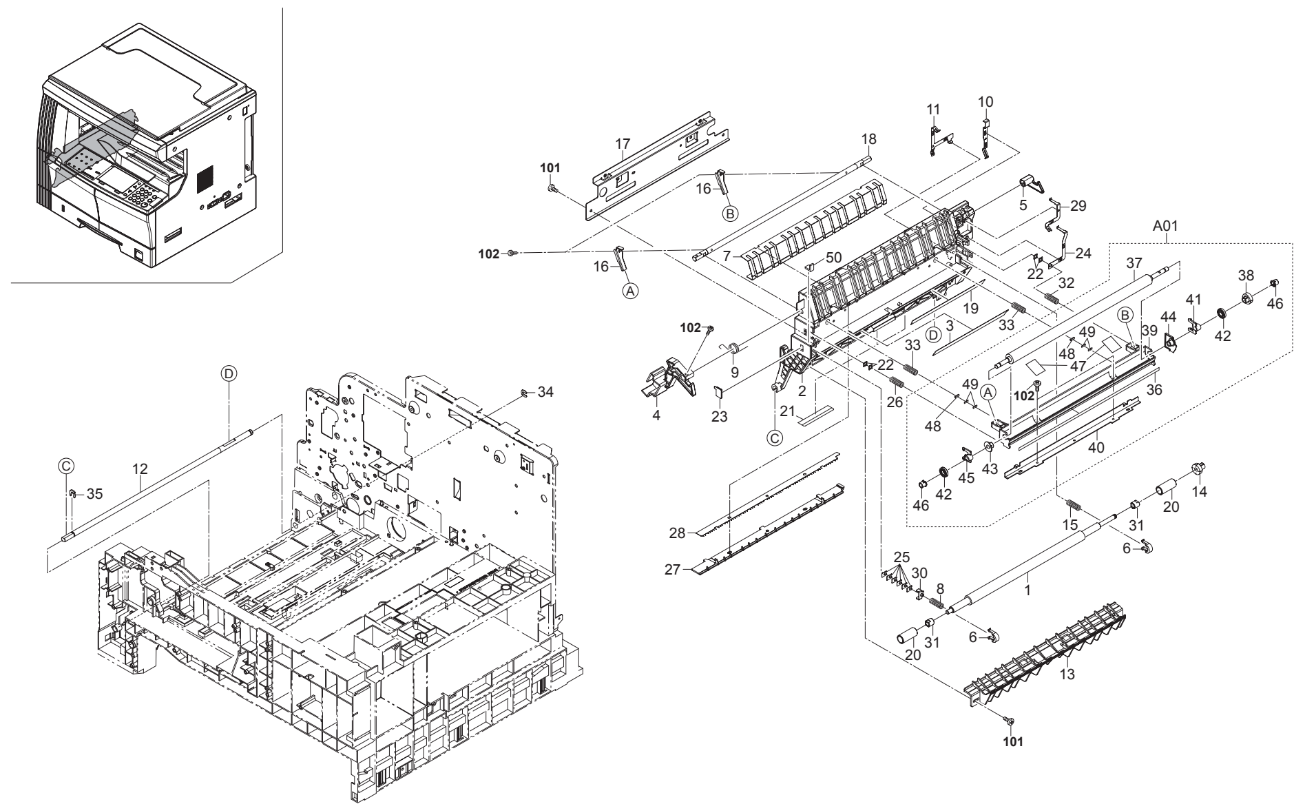
FIG. 4 Conveying
