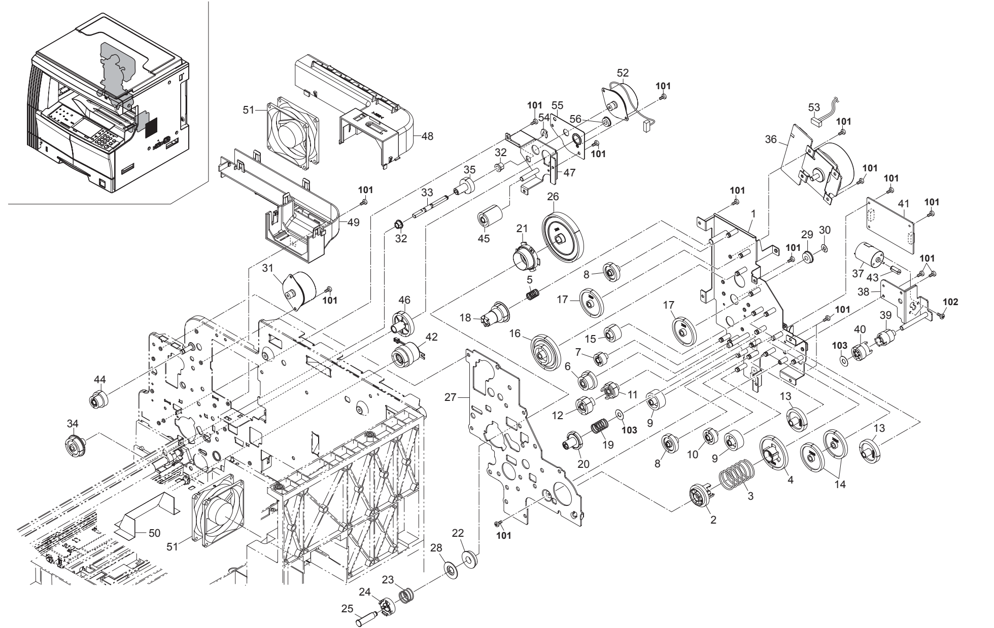
FIG. 11 Driving & Cooling
