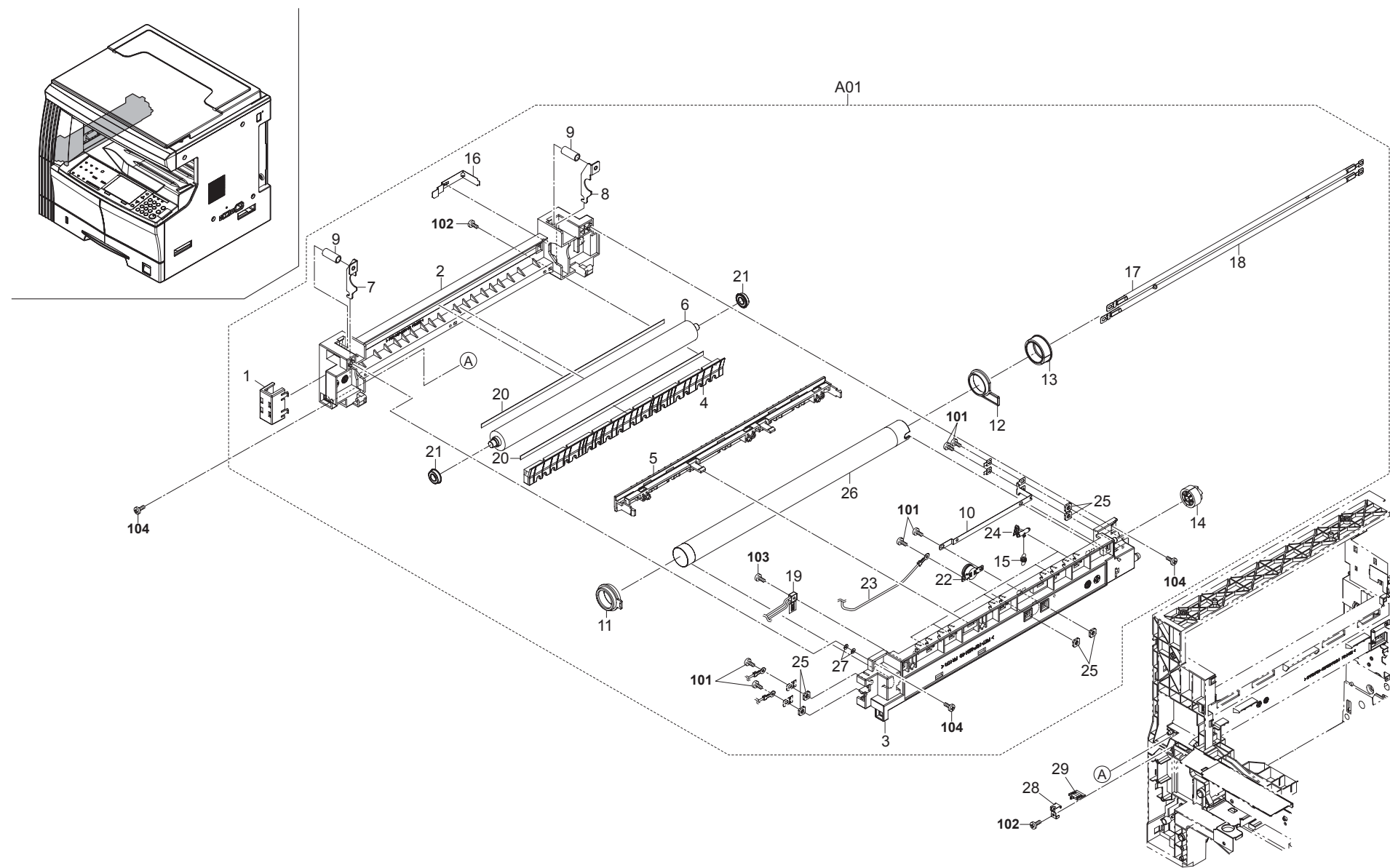
FIG. 10 Fuser Unit
