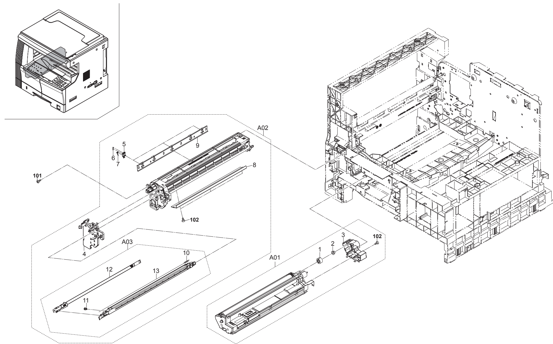
FIG. 9 Imaging Unit
