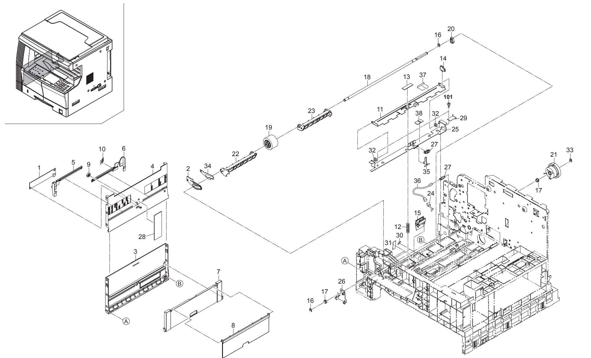
FIG. 6 Bypass
