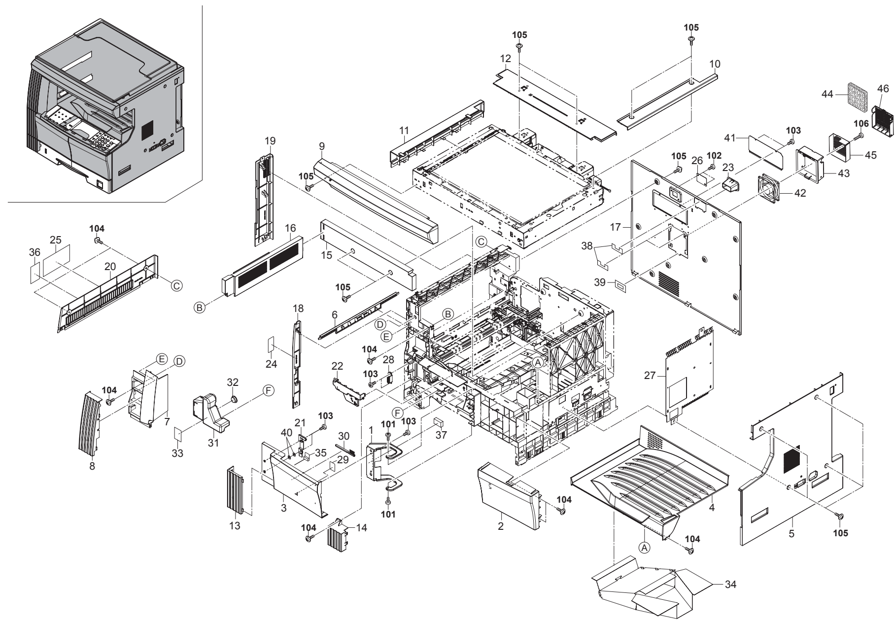
FIG. 1 Covers
