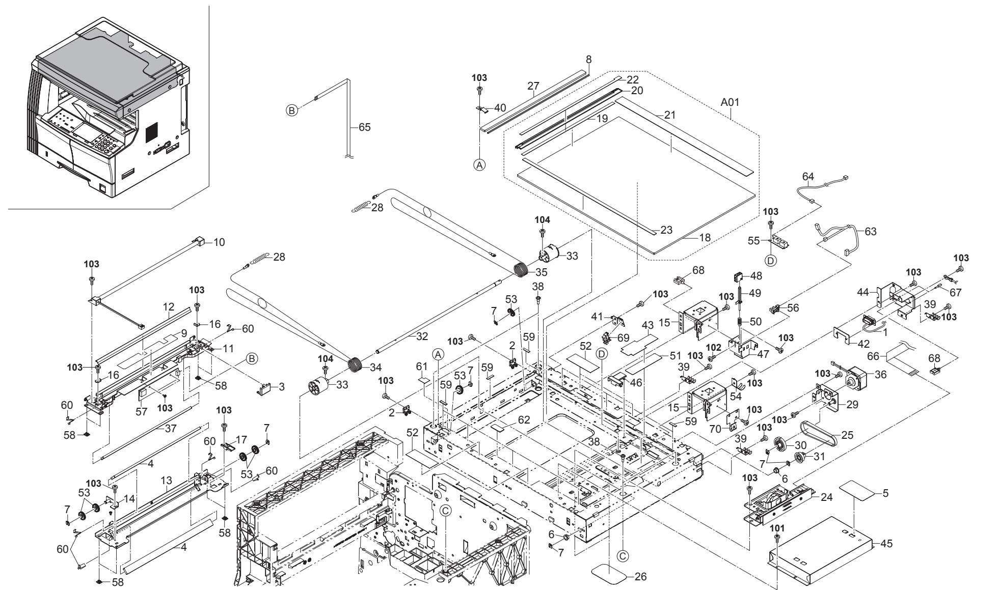
FIG. 8 Scanner
