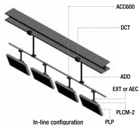
In-line configuration
