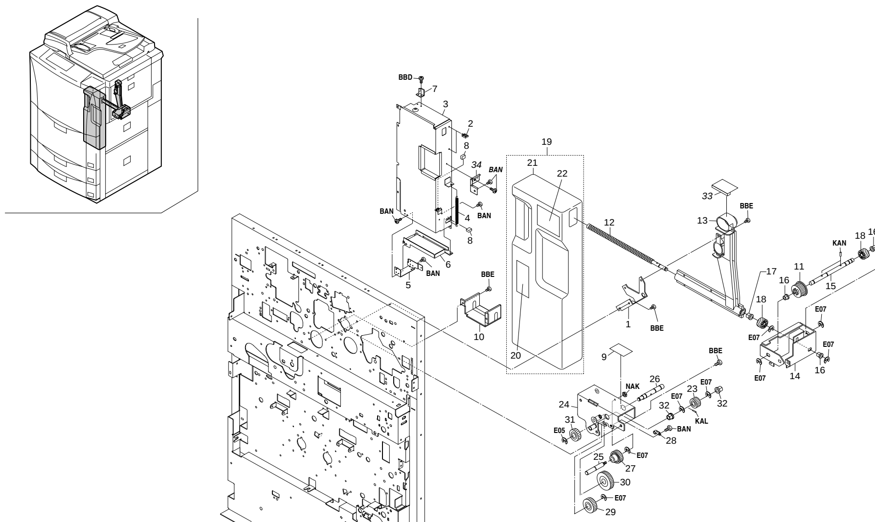
FIG.22 CLEANING SECTION II
