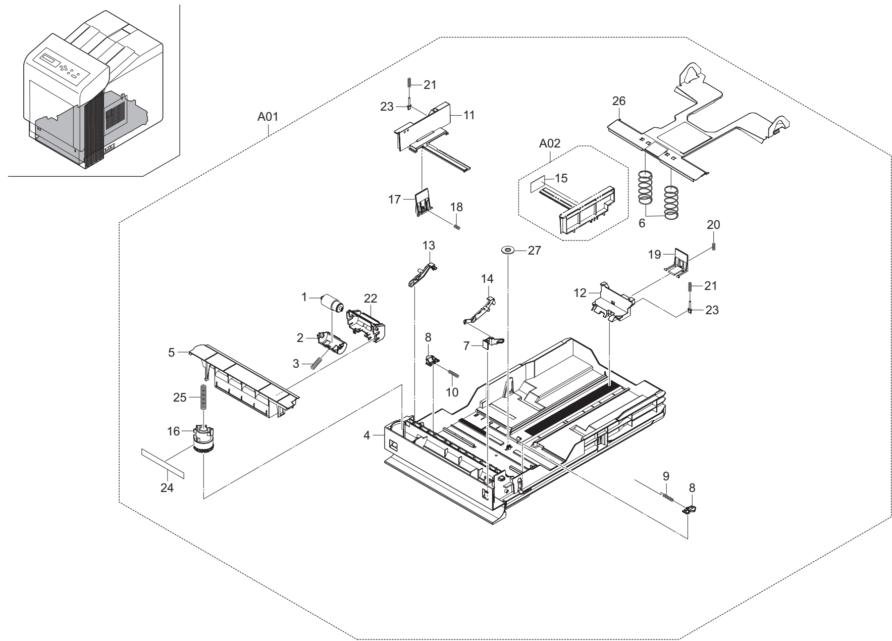
FIG. 5 Paper Cassettes (21/23ppm 250sheet)
