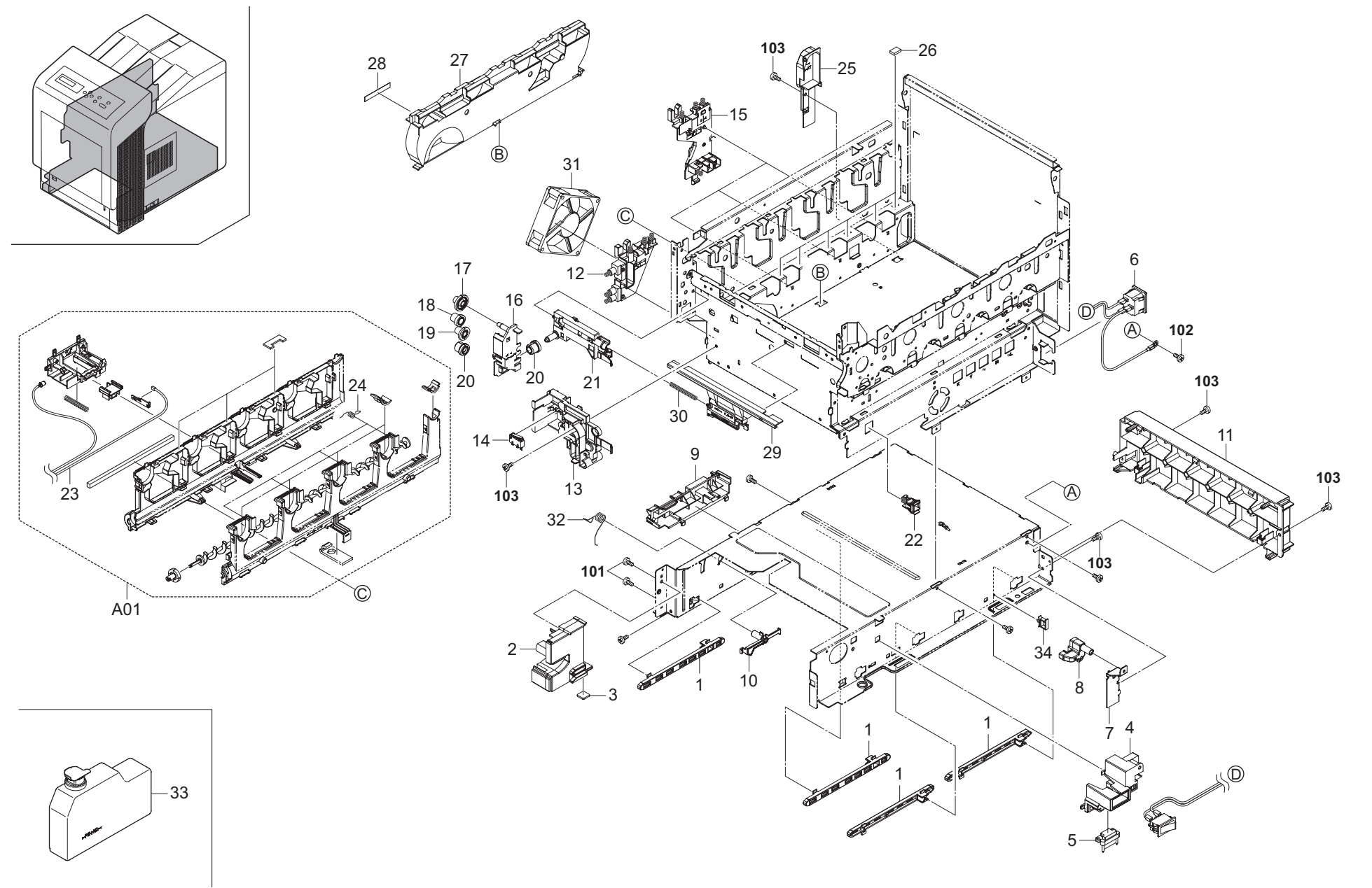
FIG. 4 Frames 2 (21/23ppm 500sheet, 26/28ppm 500sheet)
