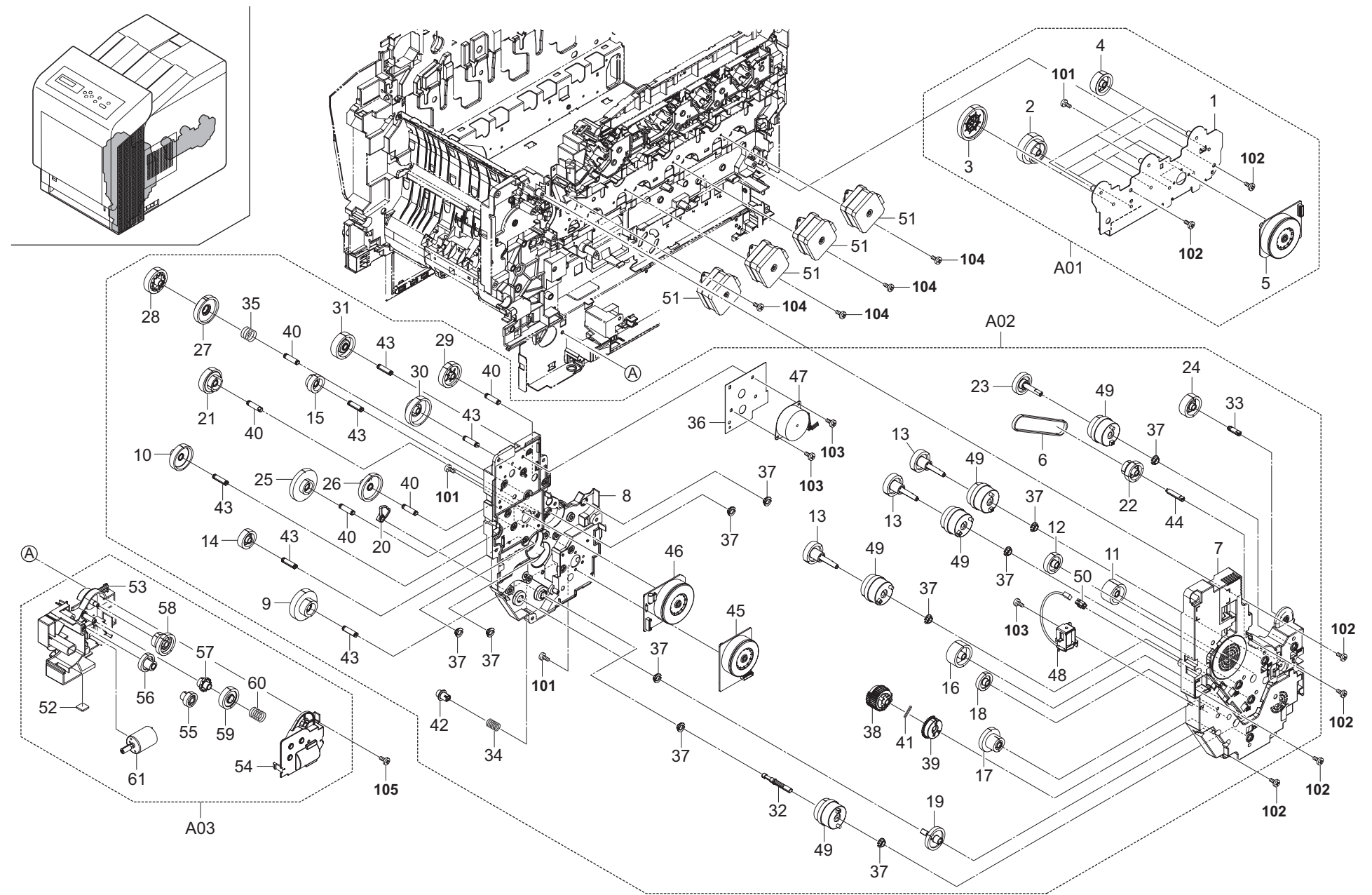
FIG. 12 Drive Section (26/28ppm 500sheet)
