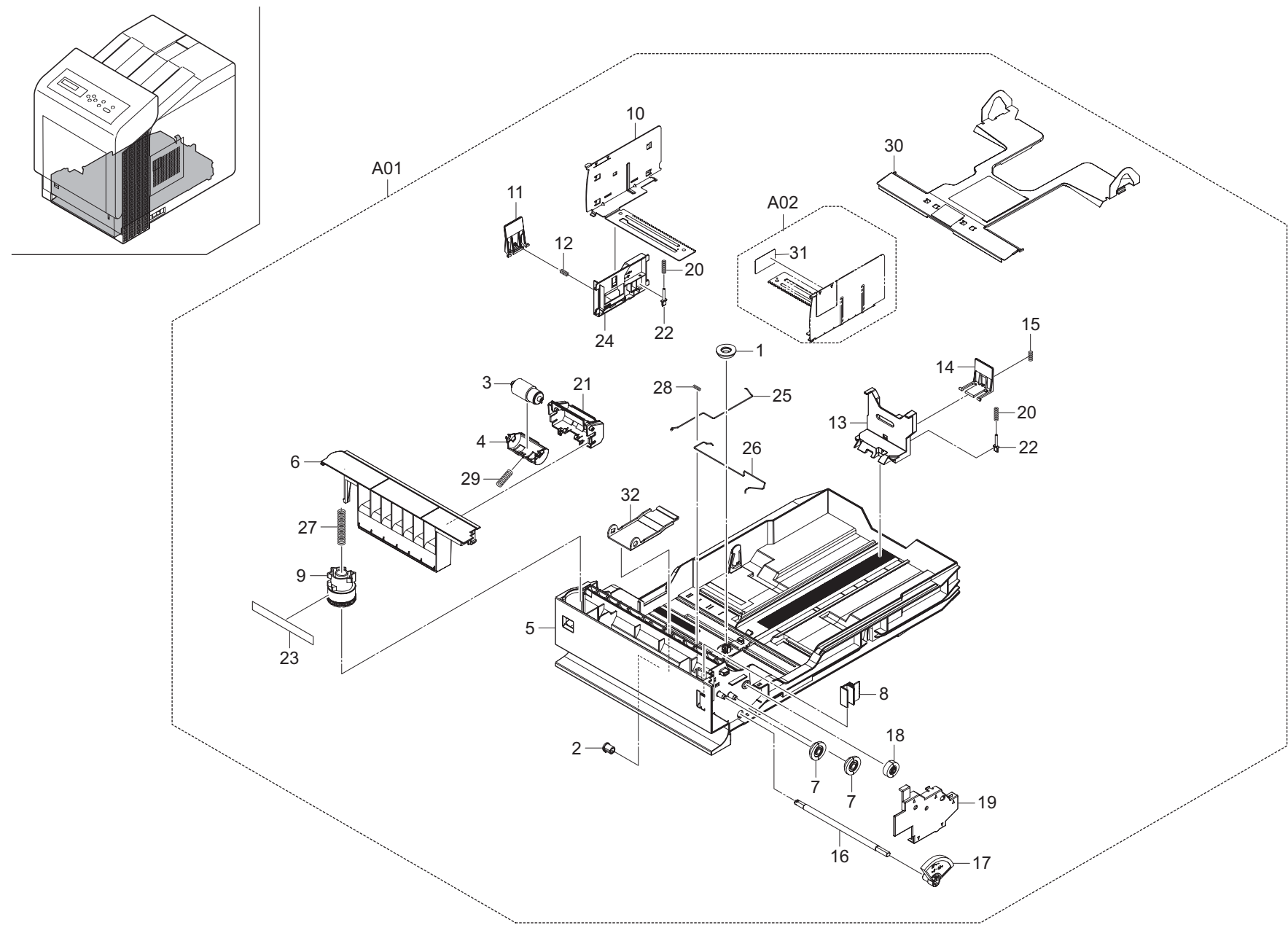
FIG. 5 Paper Cassettes (21/23ppm 500sheet, 26/28ppm 500sheet)
