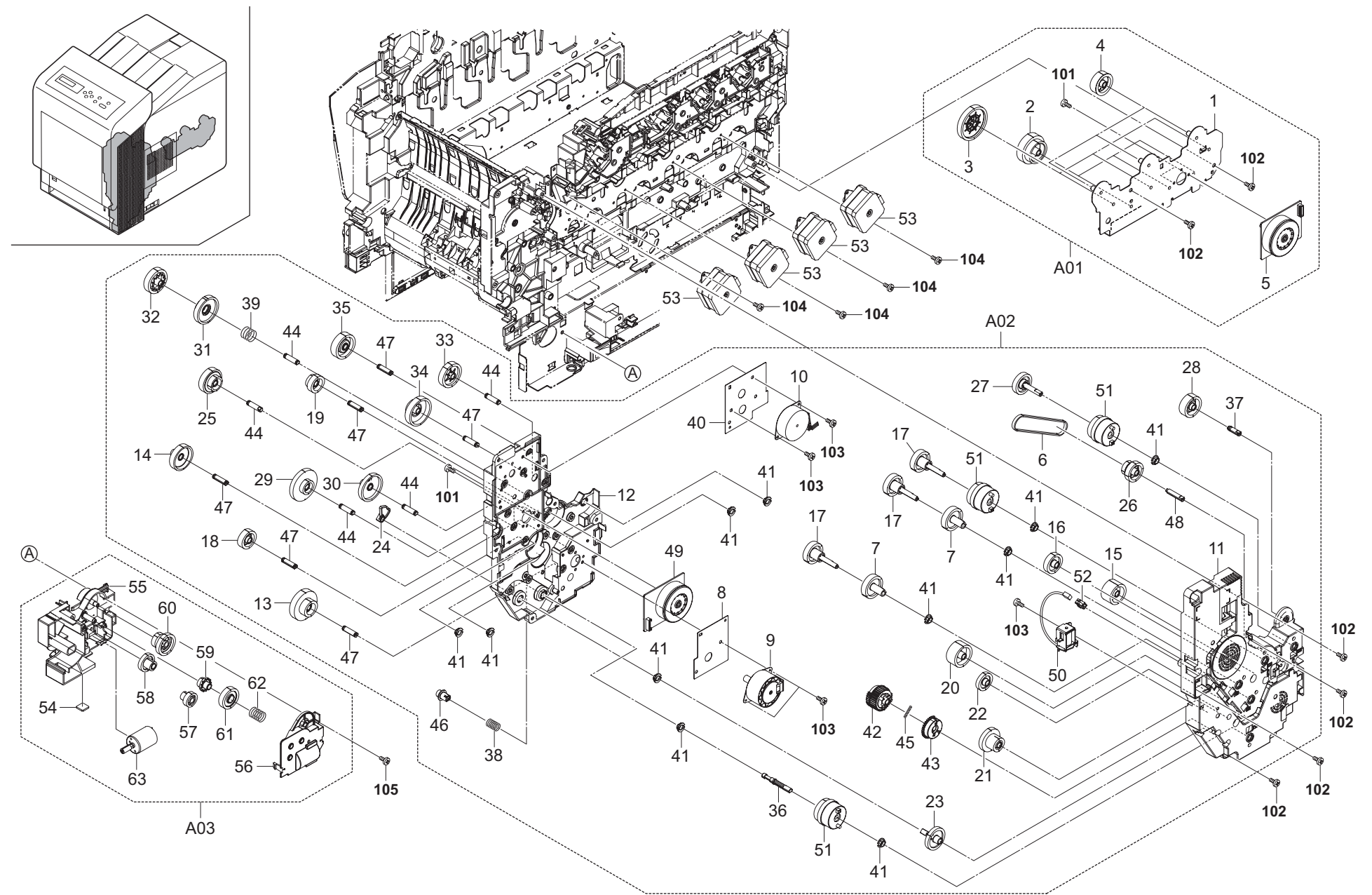
FIG. 12 Drive Section (21/23ppm 250sheet, 21/23ppm 500sheet)
