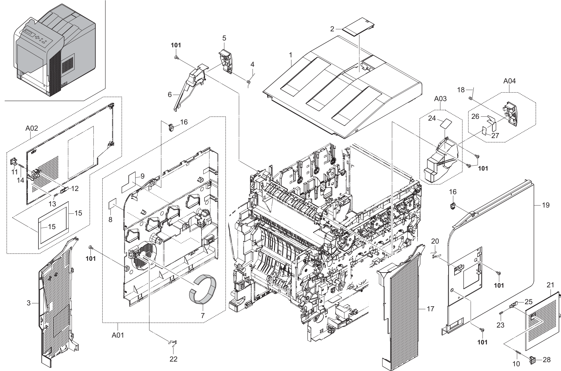
FIG. 1 Covers 1 (21/23ppm 500sheet, 26/28ppm 500sheet)
