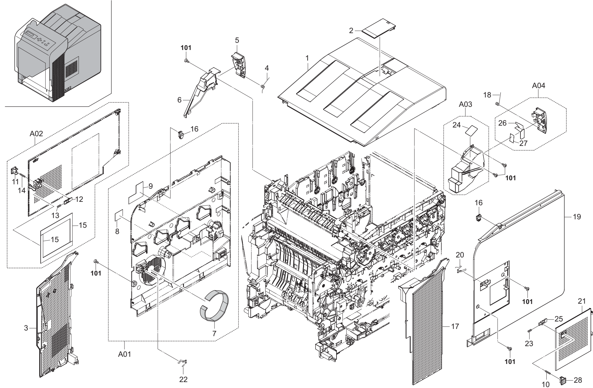
FIG. 1 Covers 1 (21/23ppm 250sheet)
