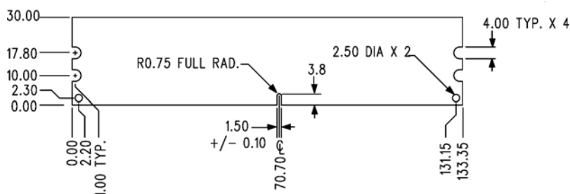
Figure 1: KVR800D2D4P6K2/4G 240-Pin DIMM
