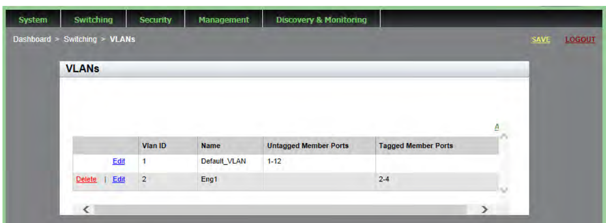
Figure 47. VLANs Page
