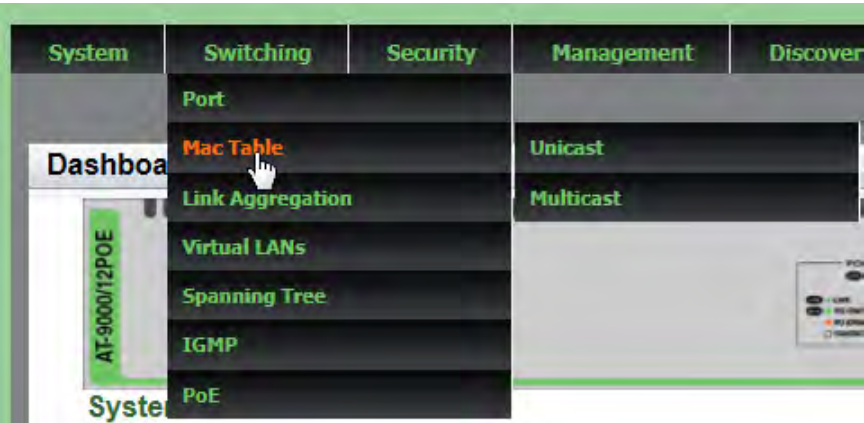
Figure 33. Switching Tab
