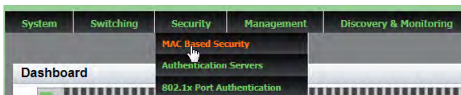
Figure 57. Security Tab
