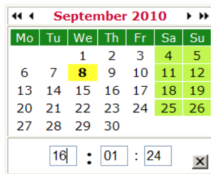
Figure 8. Calendar Page
