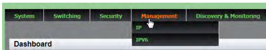
Figure 69. Management Tab
