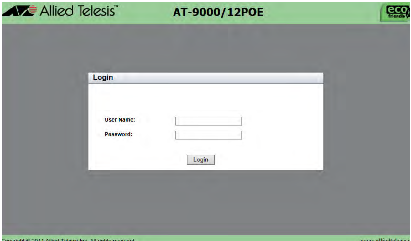
Figure 3. Login Page
