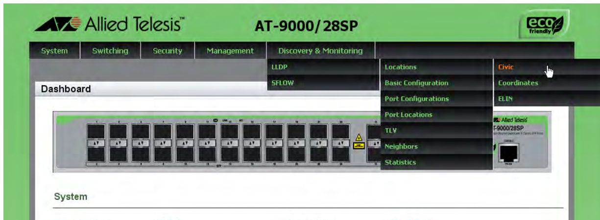
Figure 74. Locations Tab
