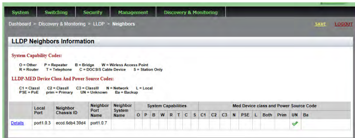
Figure 91. LLDP Neighbors Information Page
