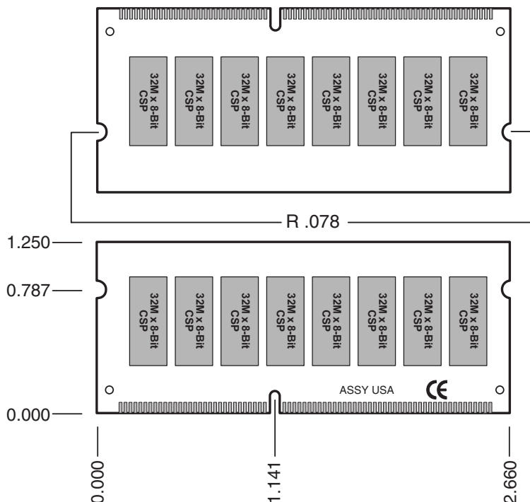
Figure 1: KVR133X64SC3/512 144-Pin SDRAM Module
