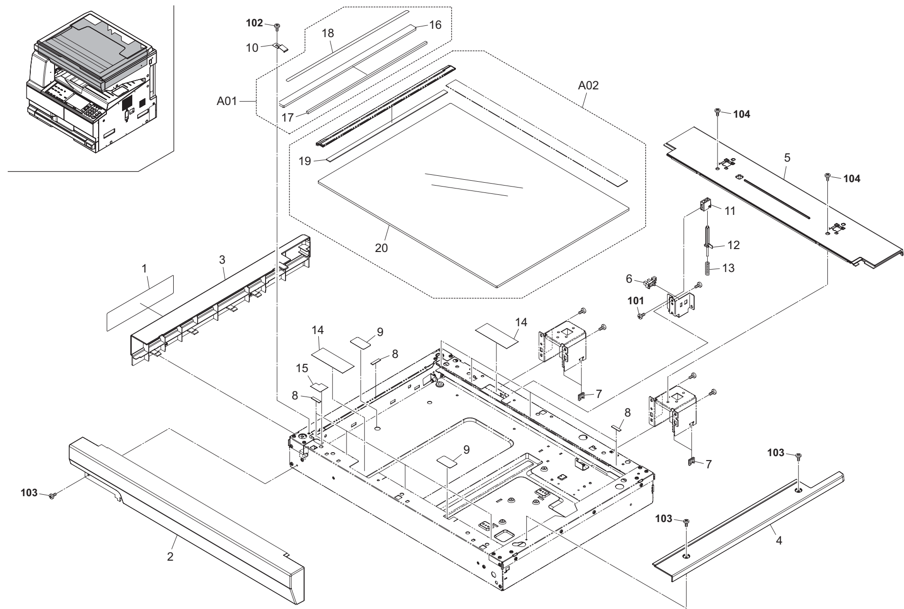
FIG. 8 Scanner Section 2
