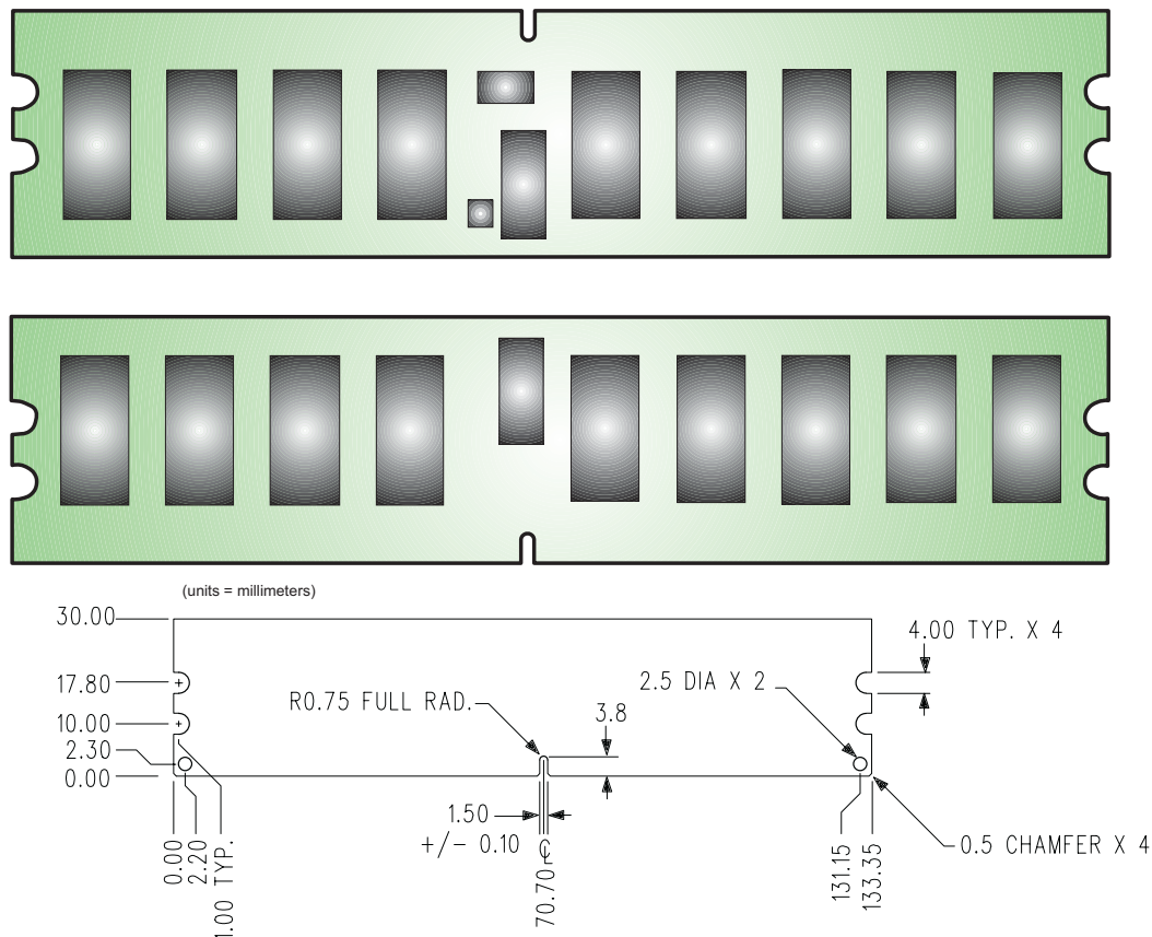
Figure 1: KVR800D2S4P6K2/2G 240-Pin DIMM
