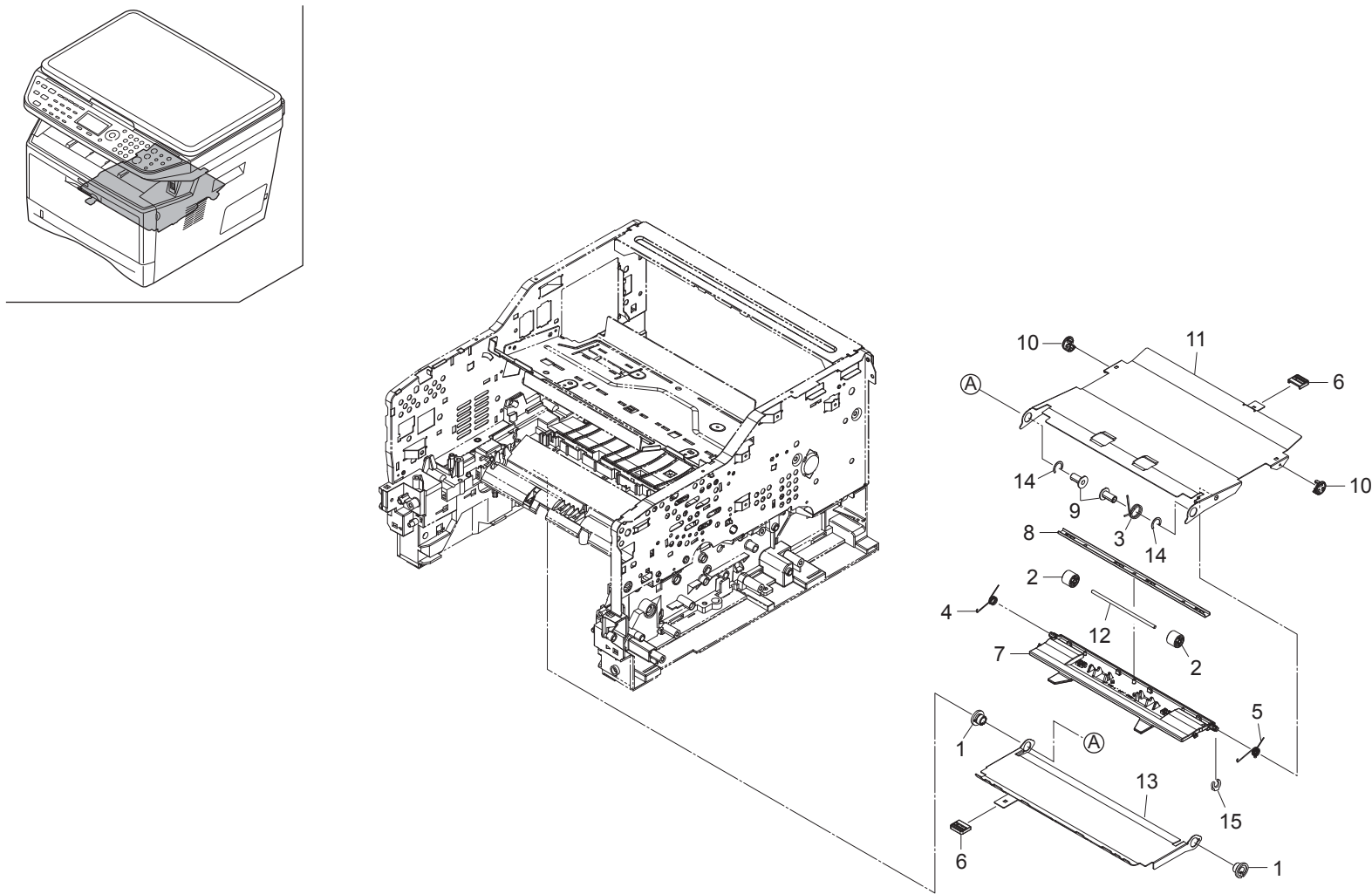
FIG. 11 Paper Conveying Section
