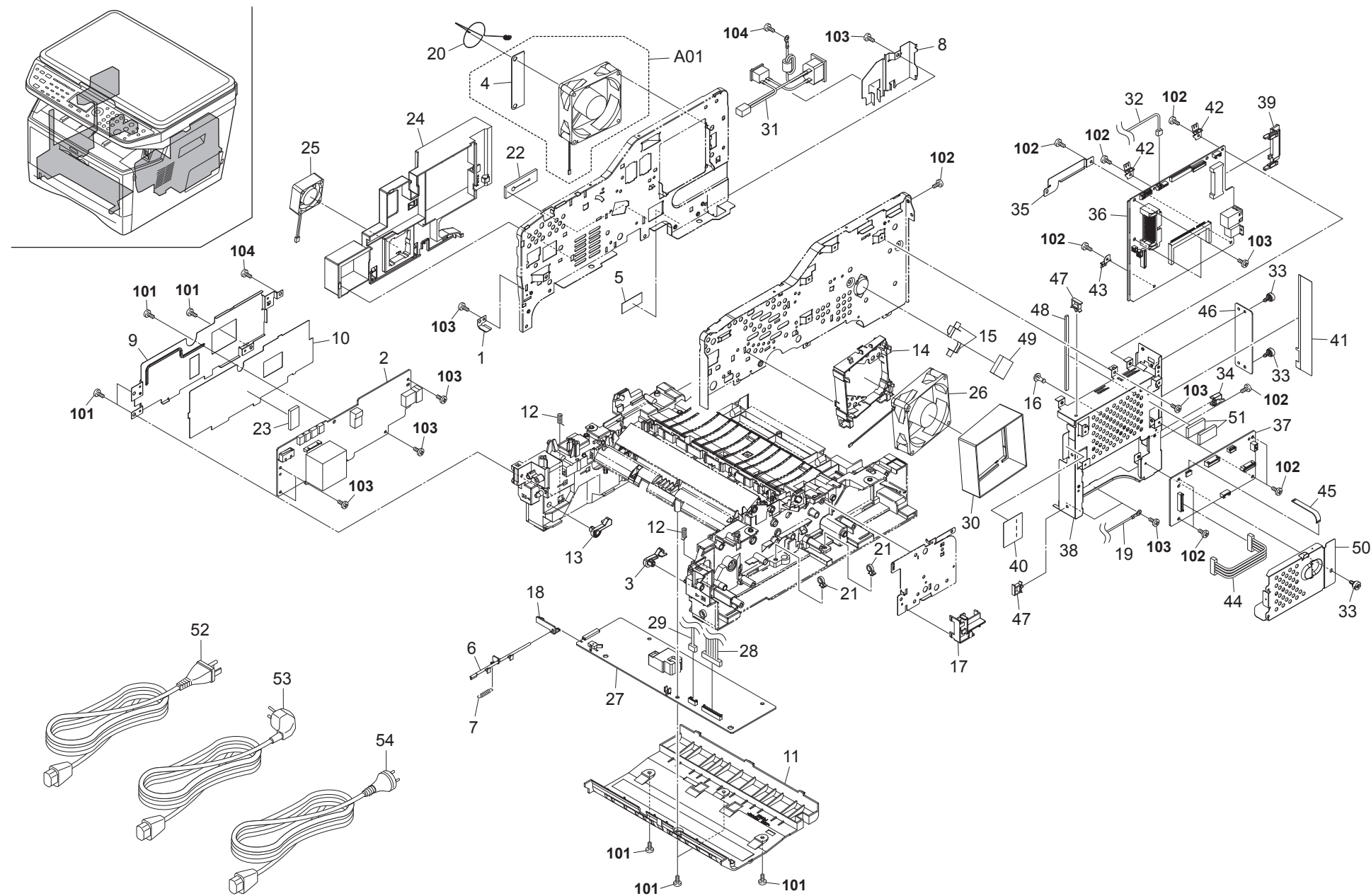
FIG. 12 Electrical Components
