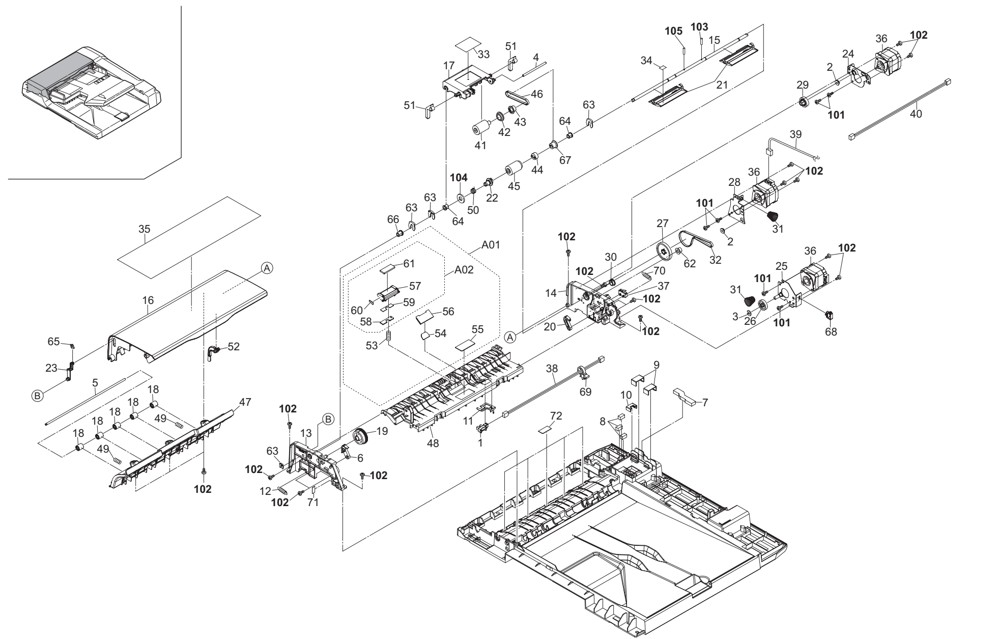
FIG. 3 Paper Feed Section
