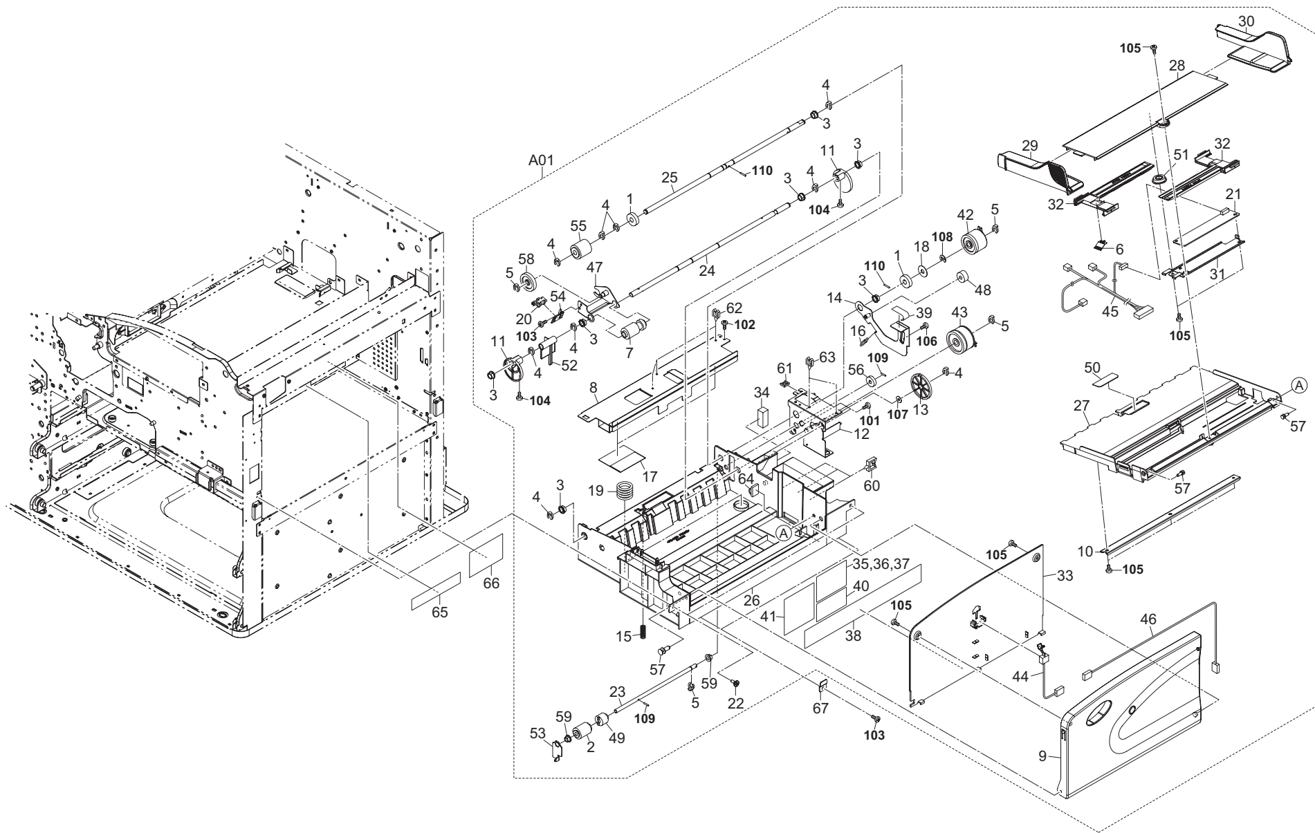
FIG. 9 Bypass Unit
