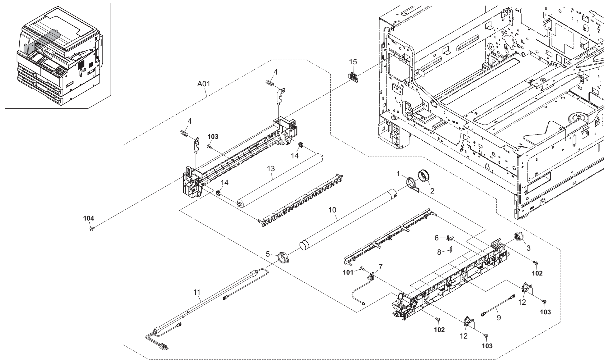
FIG. 15 Fuser Section
