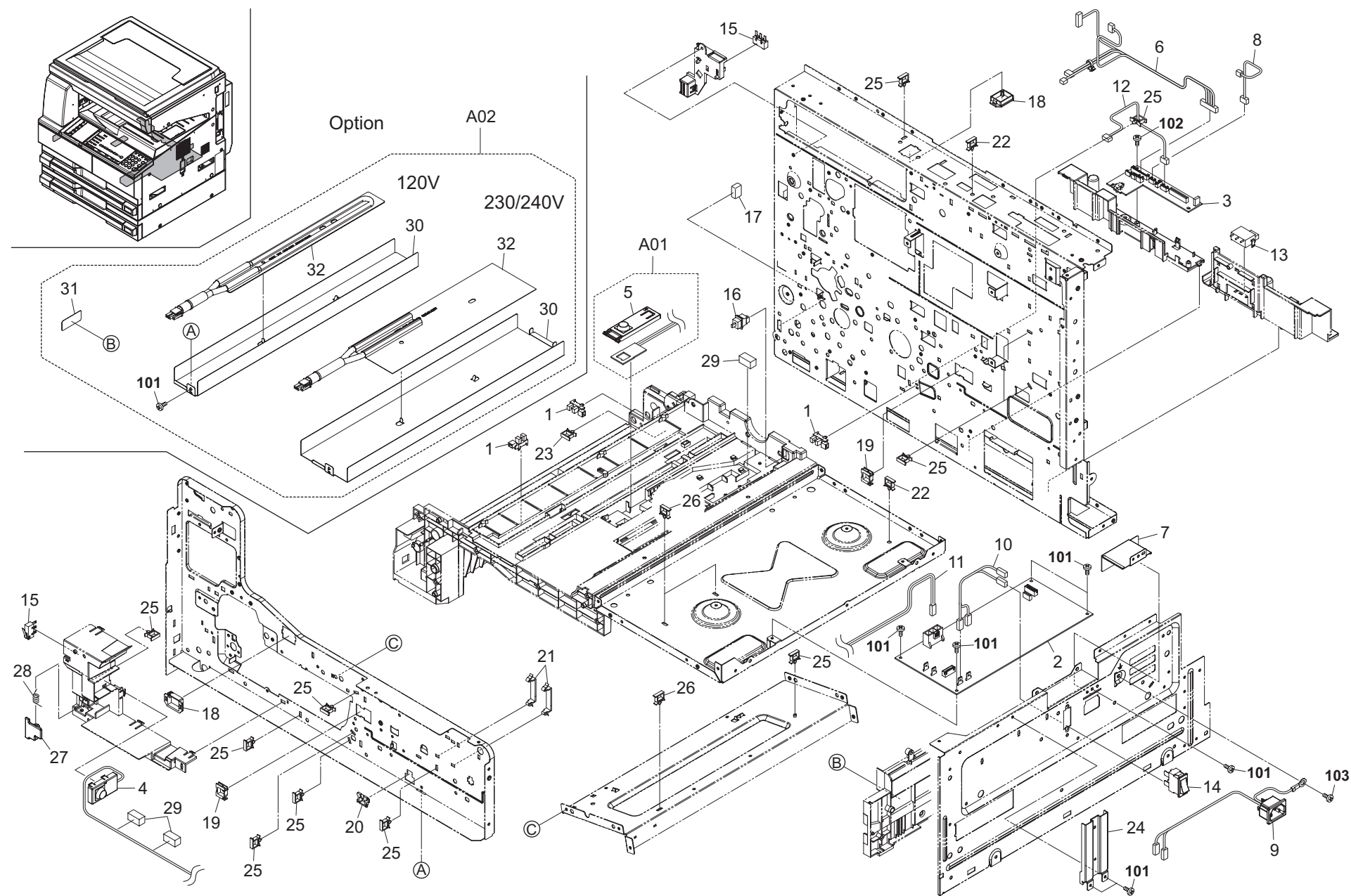
FIG. 19 Electrical Components 1
