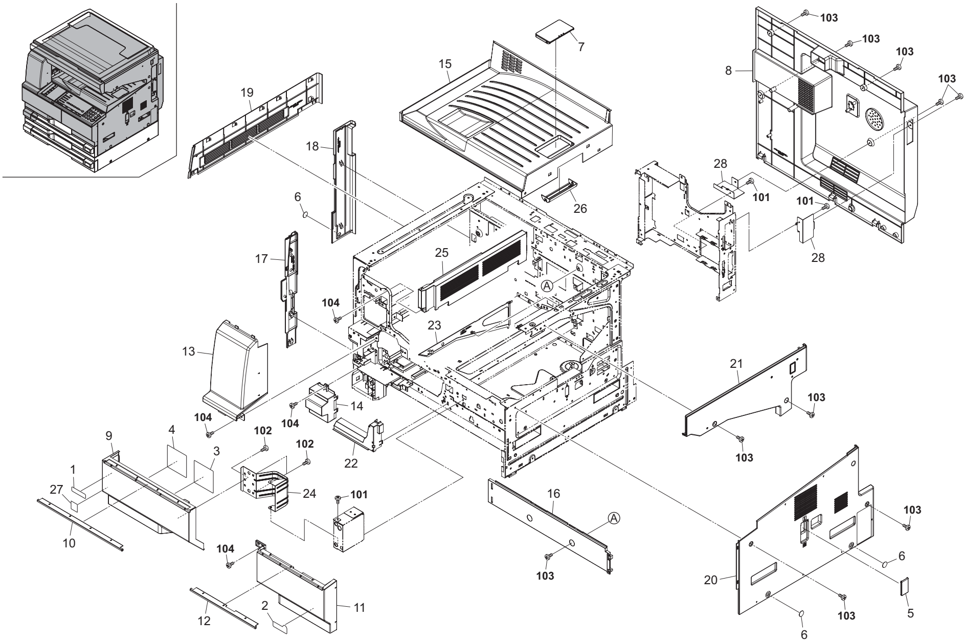
FIG. 1 Covers
