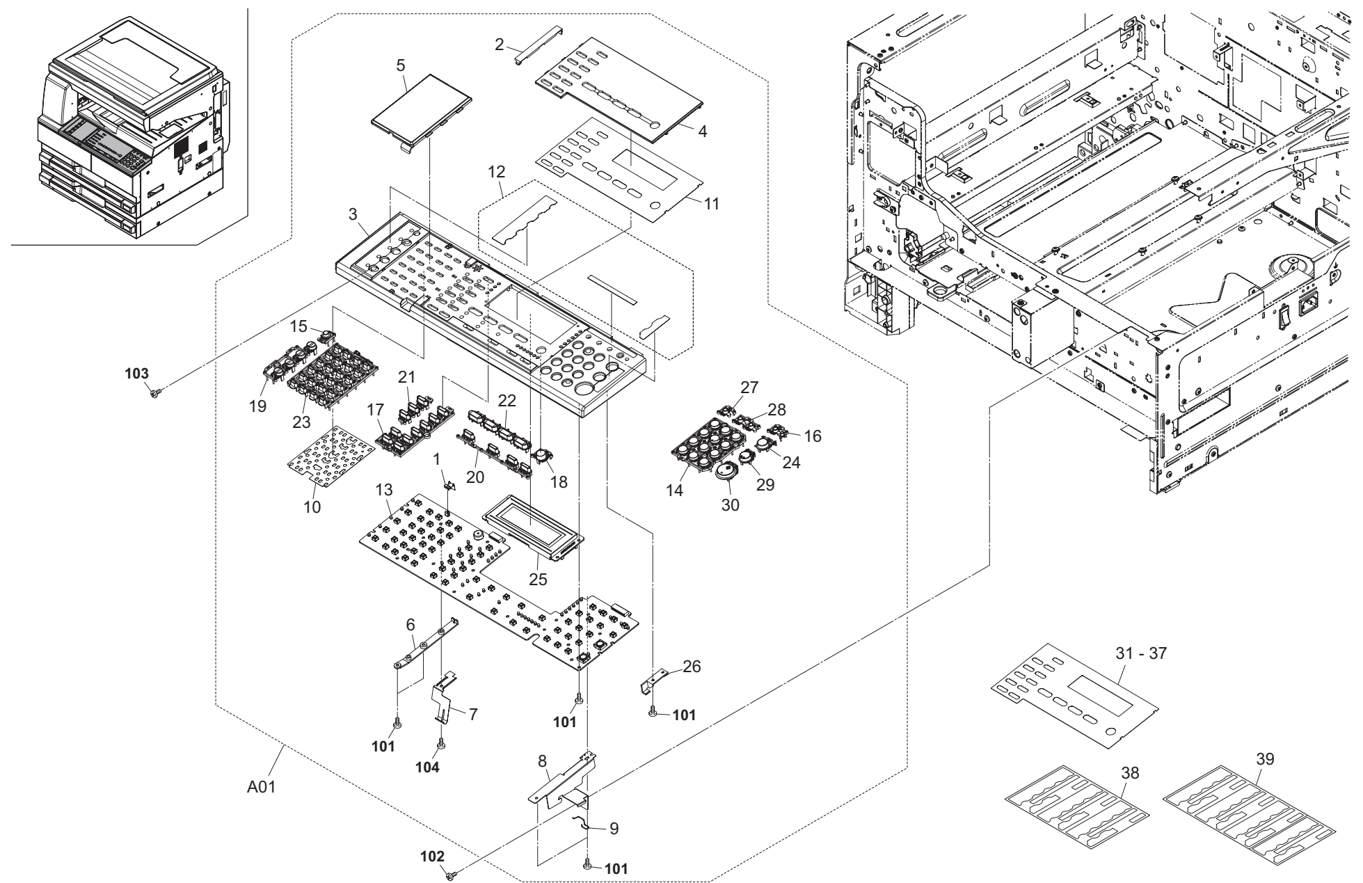
FIG. 22 Operation Section
