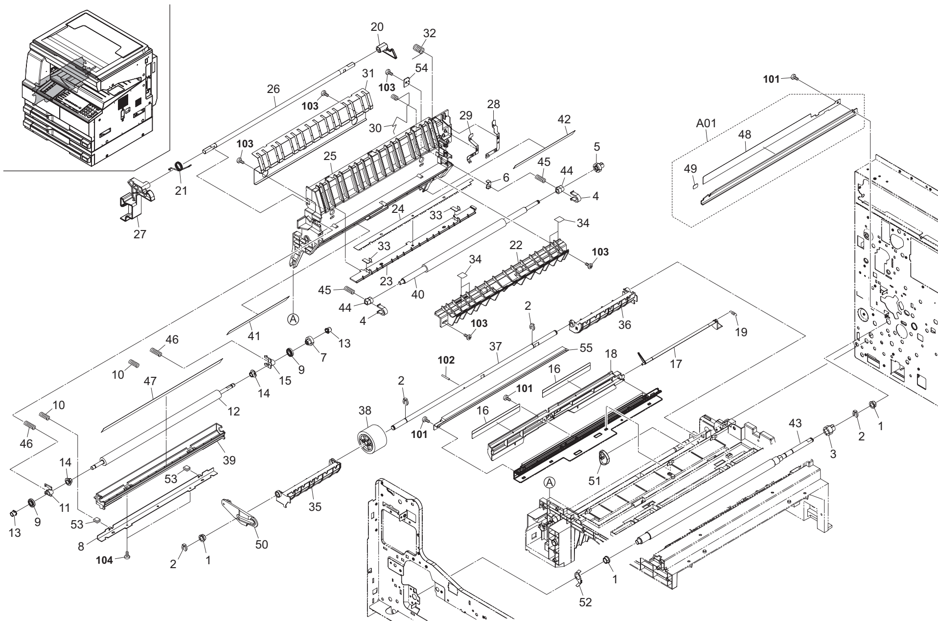
FIG. 5 Paper Feed Section 2
