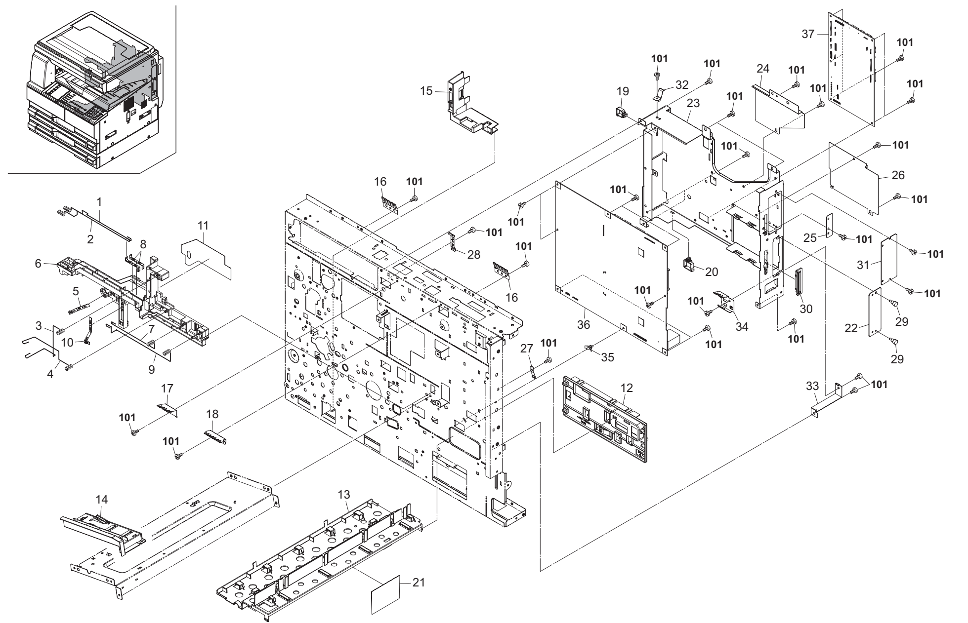
FIG. 21 Electrical Components 3
