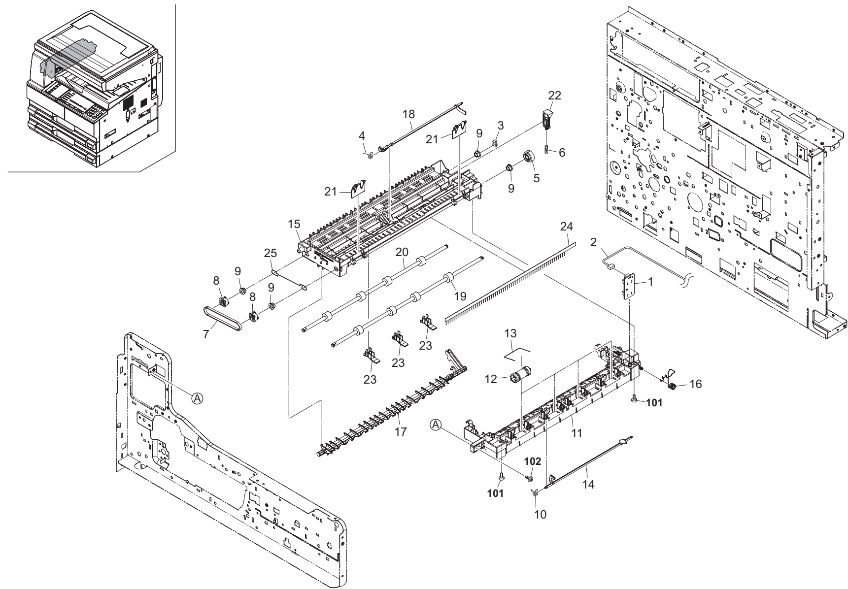
FIG. 18 Exit Section
