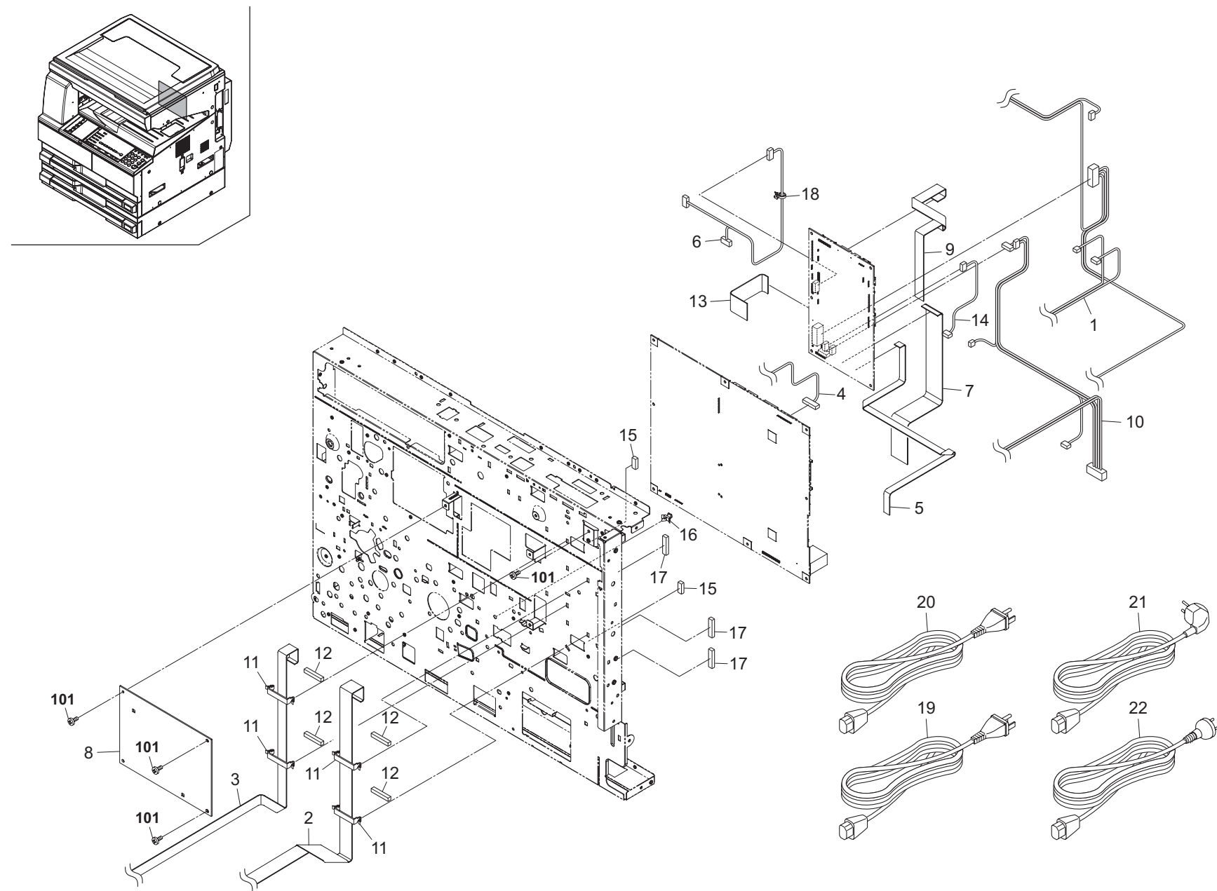
FIG. 20 Electrical Components 2
