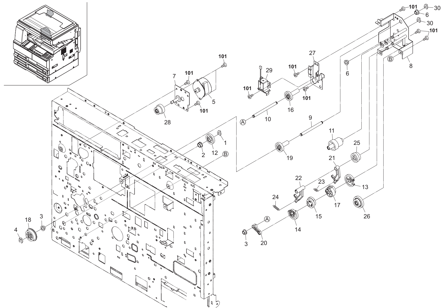
FIG. 16 Drive Section 1
