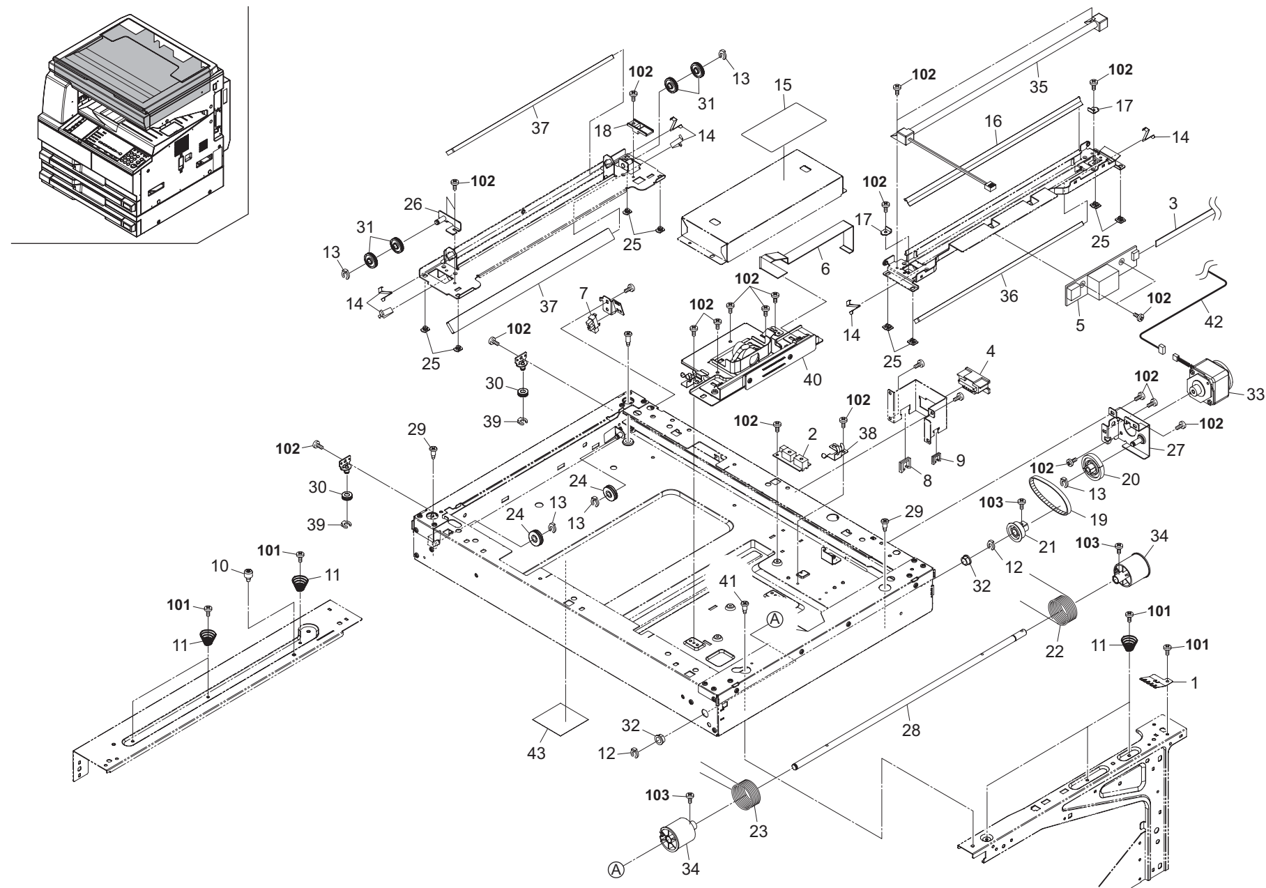
FIG. 10 Scanner Section 1
