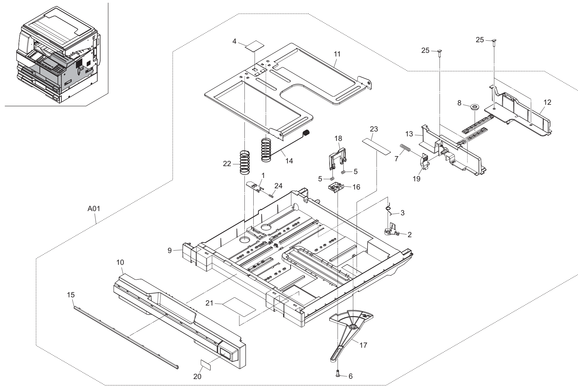
FIG. 6 Paper Cassette 1
