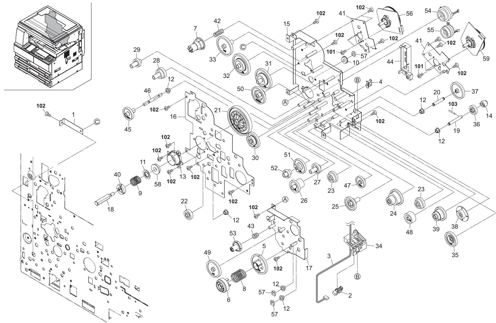
FIG. 17 Drive Section 2
