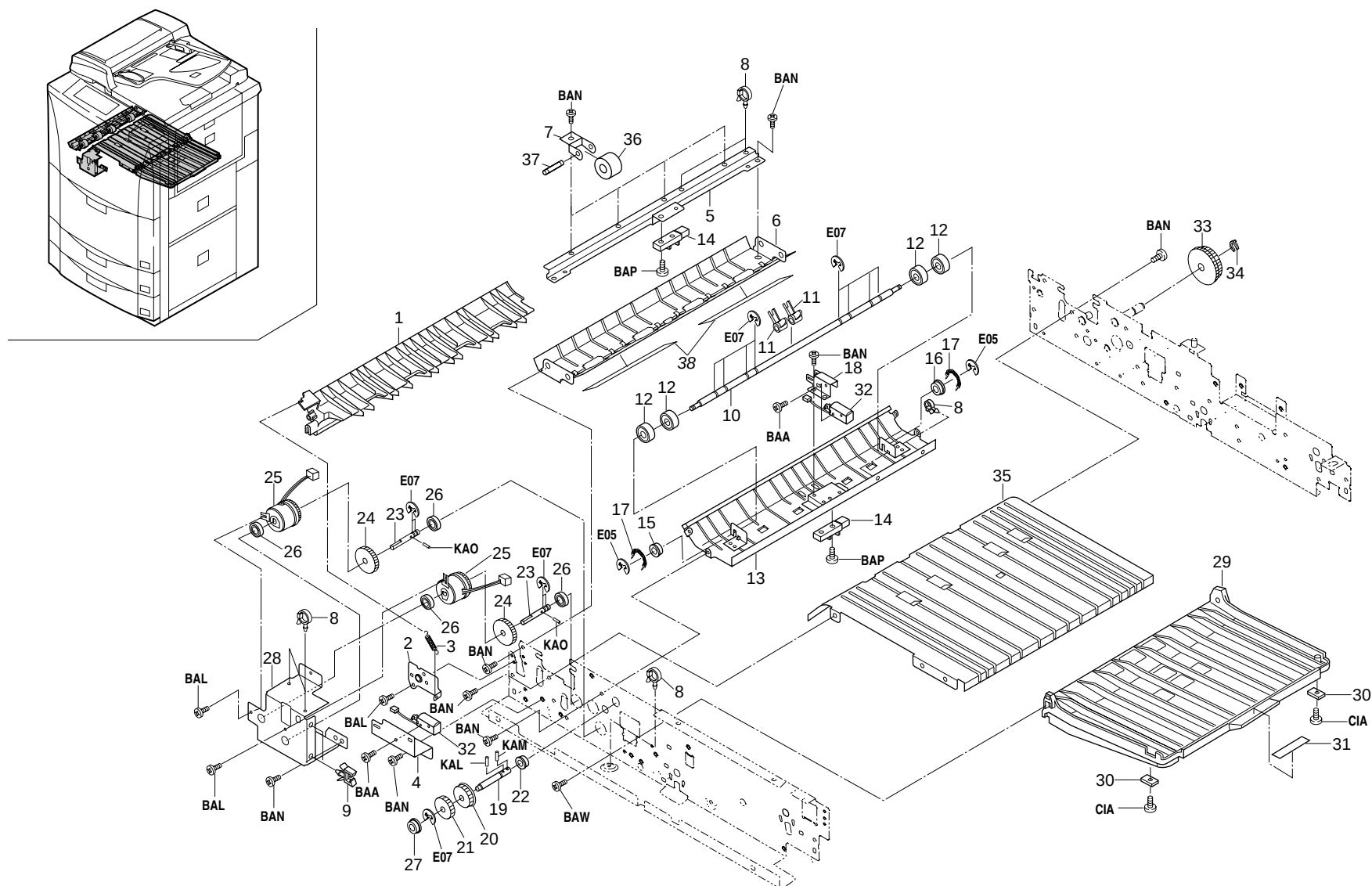
FIG.30 DUPLEX UNIT II
