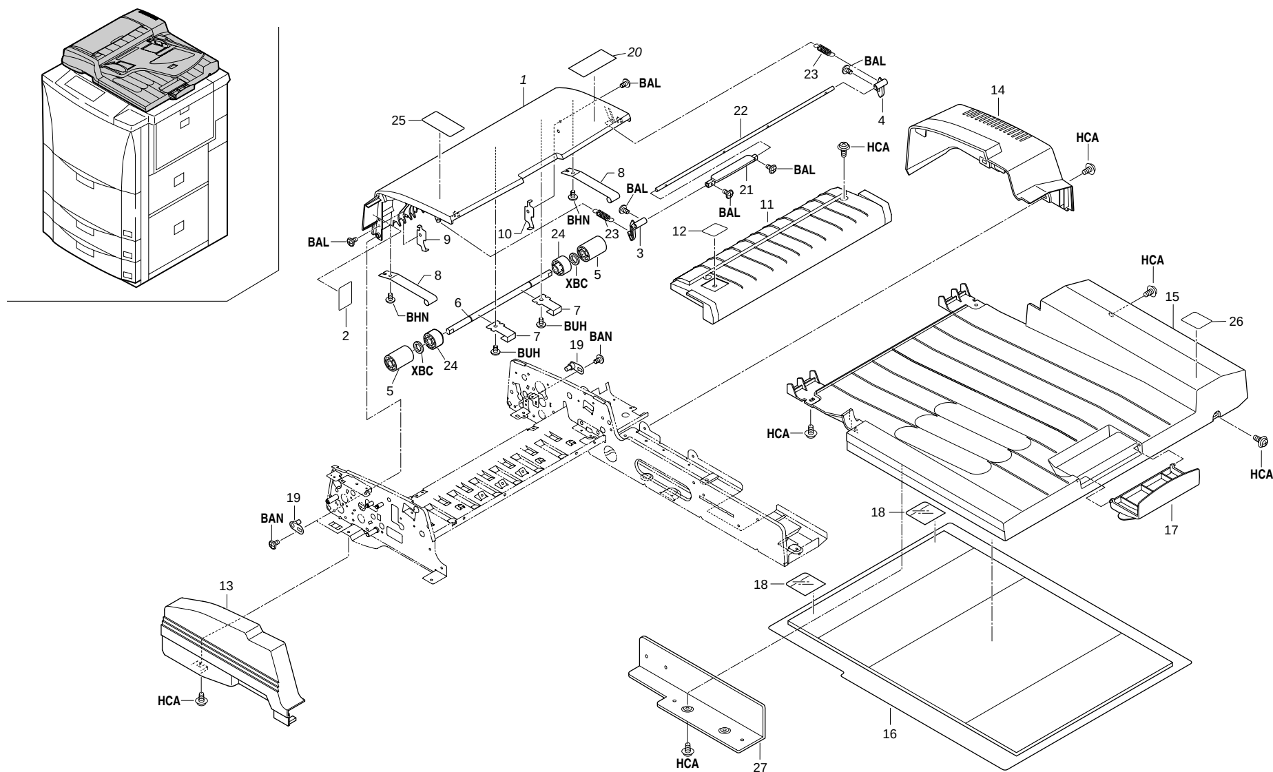
FIG.41 EXTERIOR COVERS (DP)
