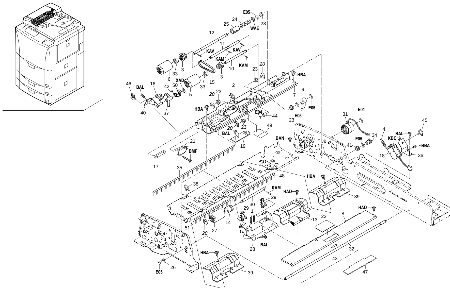
FIG.44 PAPER CONVEYING SECTION (DP)
