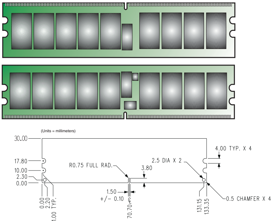
Figure 1: KVR533D2D4R4K2/8G 240-Pin DIMM
