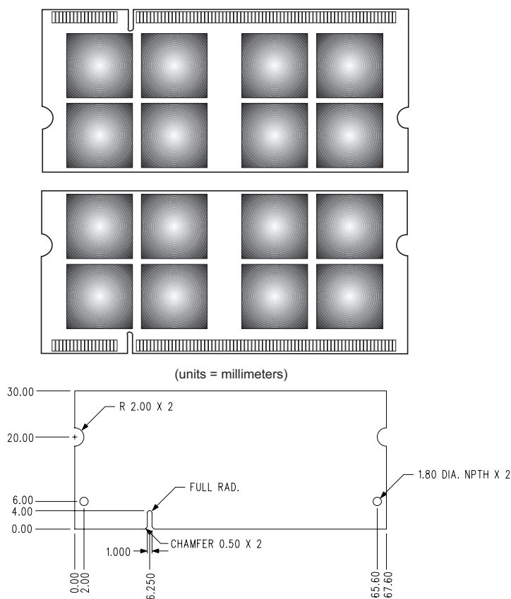
Figure 1: KVR667D2SO/2GR 200-Pin SODIMM
