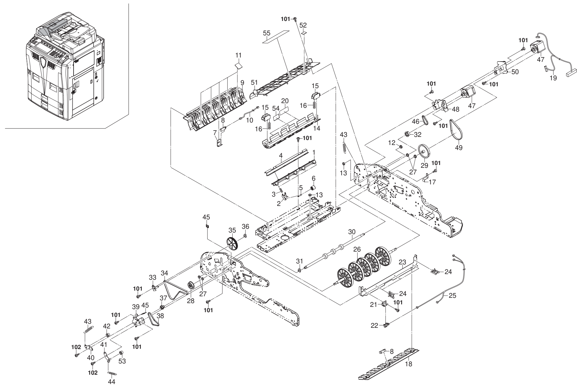
FIG. 37 Paper Conveying (DP)
