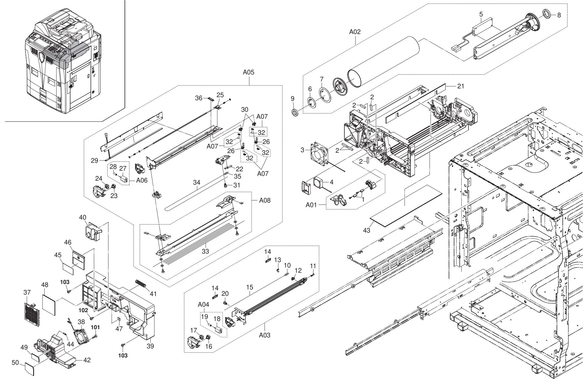
FIG. 17 Imaging Unit
