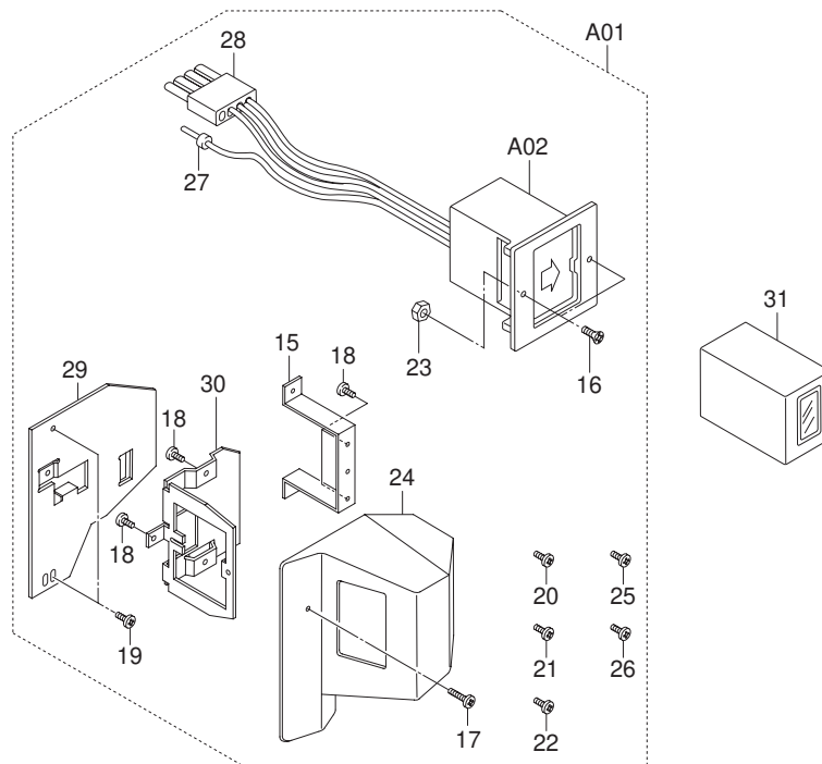
Key Counter
