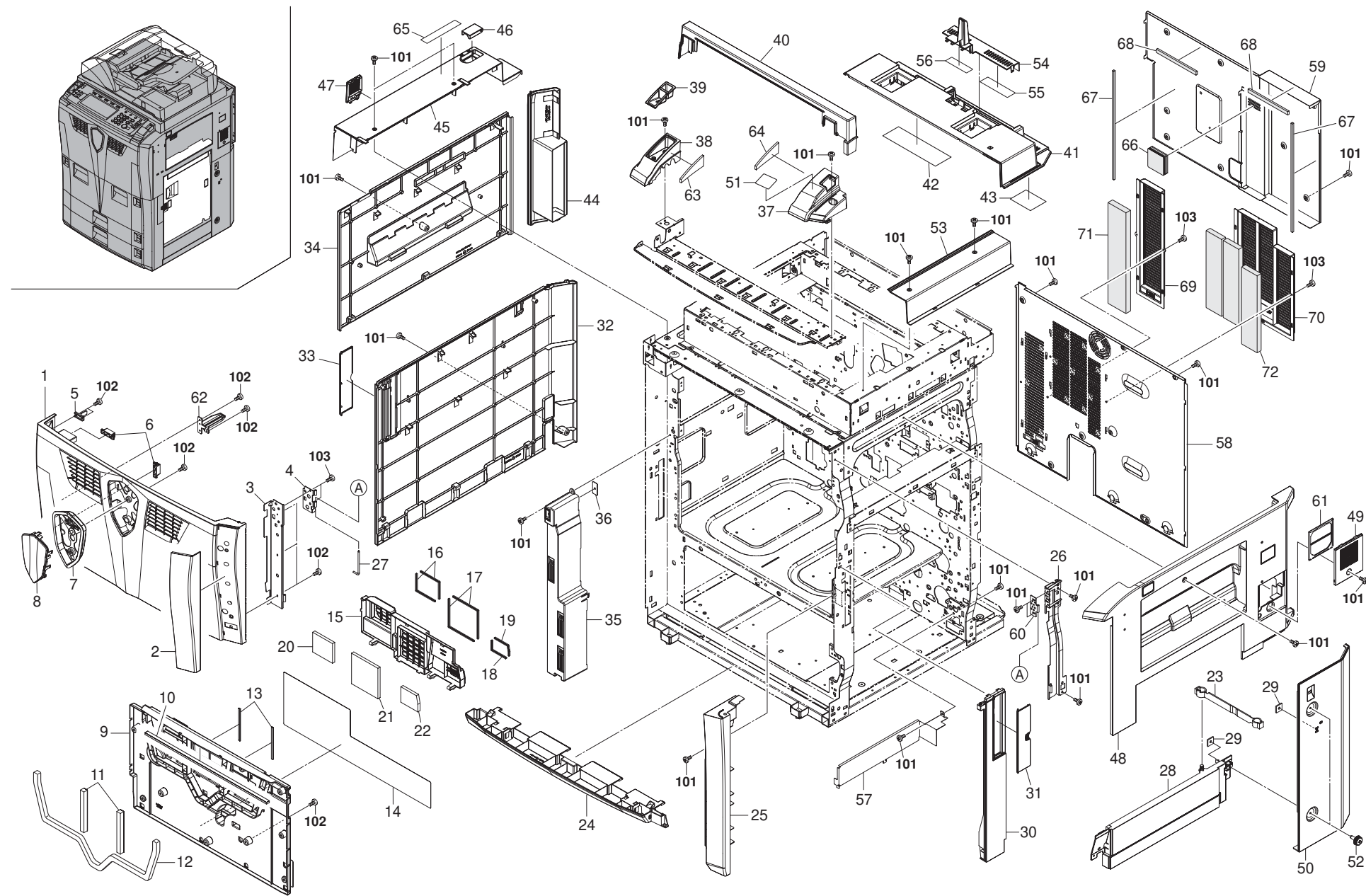
FIG. 1 Covers
