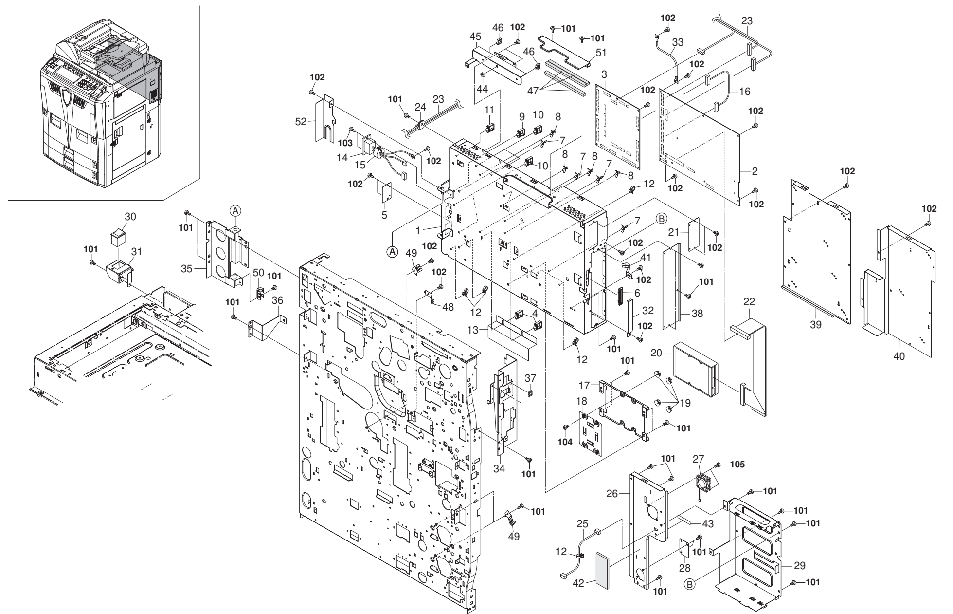
FIG. 31 Electrical Components II
