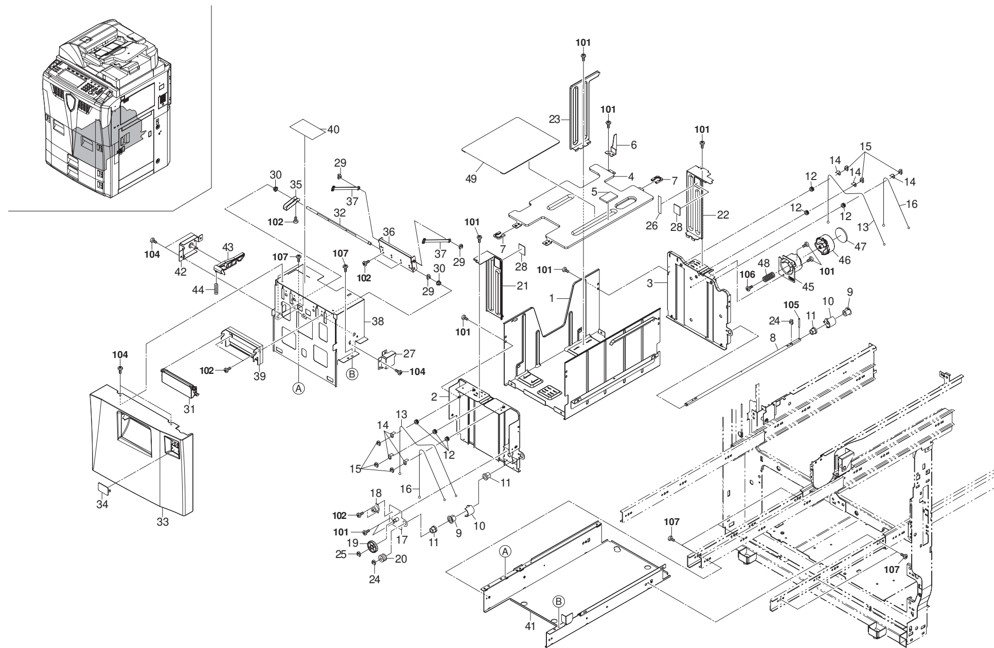
FIG. 5 Paper Deck Unit I
