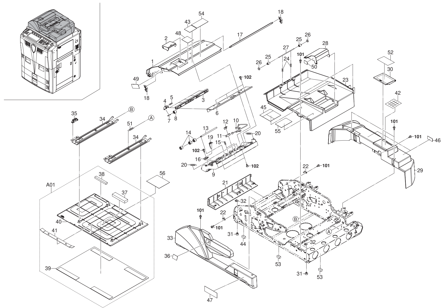
FIG. 34 Covers (DP)
