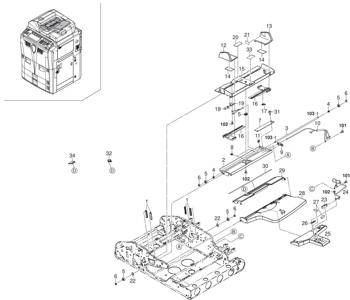
FIG. 36 Paper Feed-in (DP)
