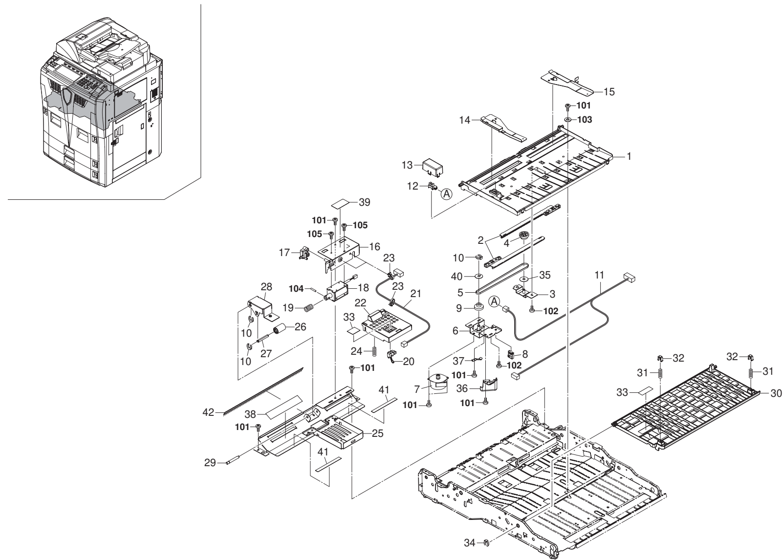
FIG. 28 Duplex Unit III
