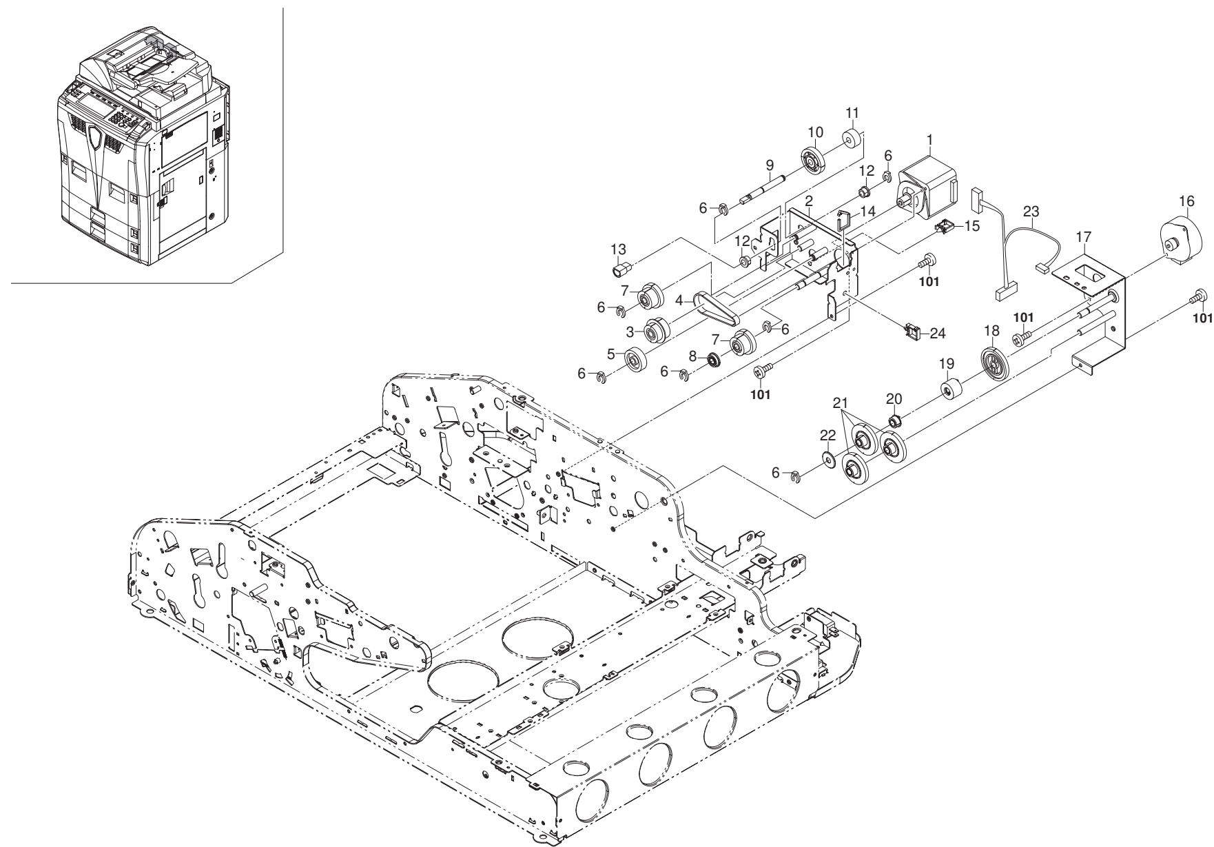
FIG. 40 Driving Unit (DP)
