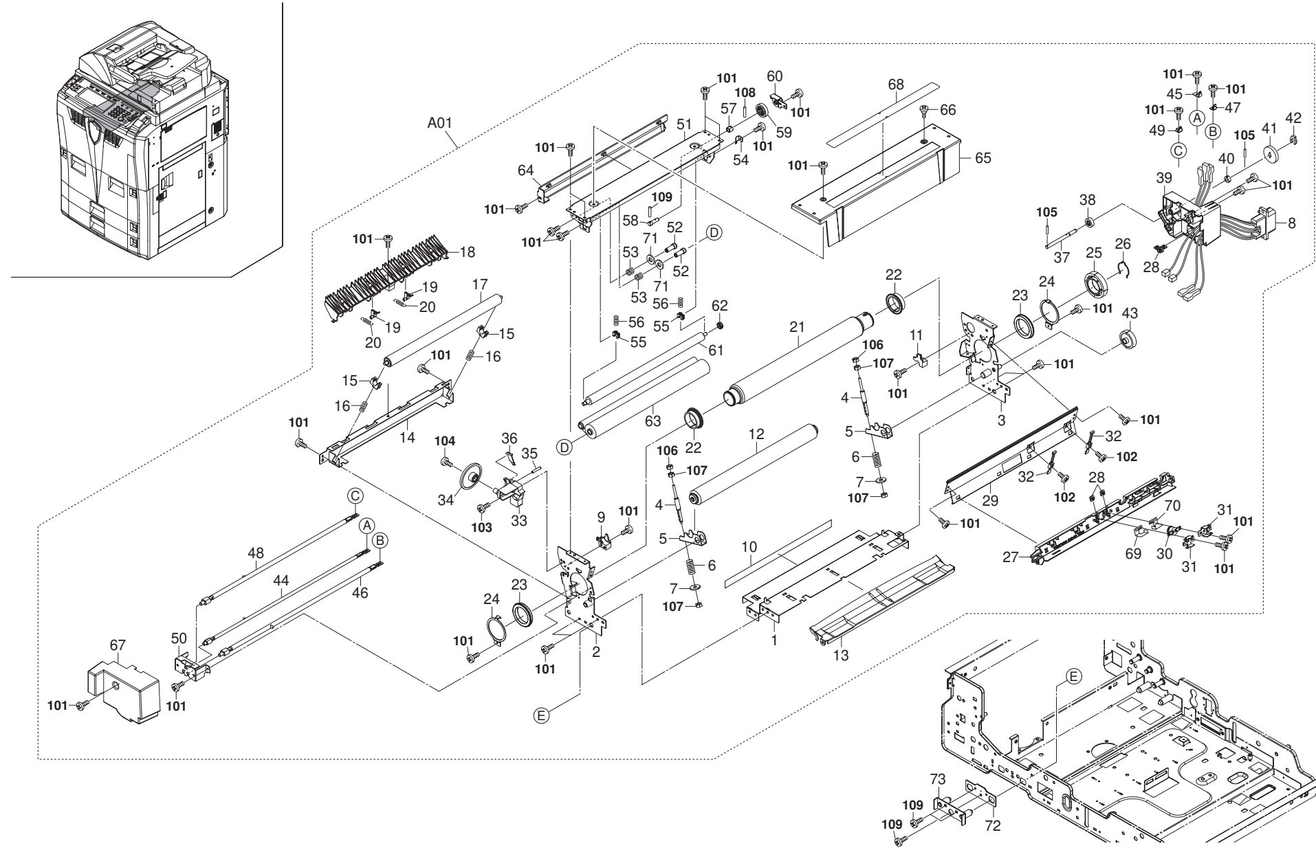
FIG. 21 Fuser Section I
