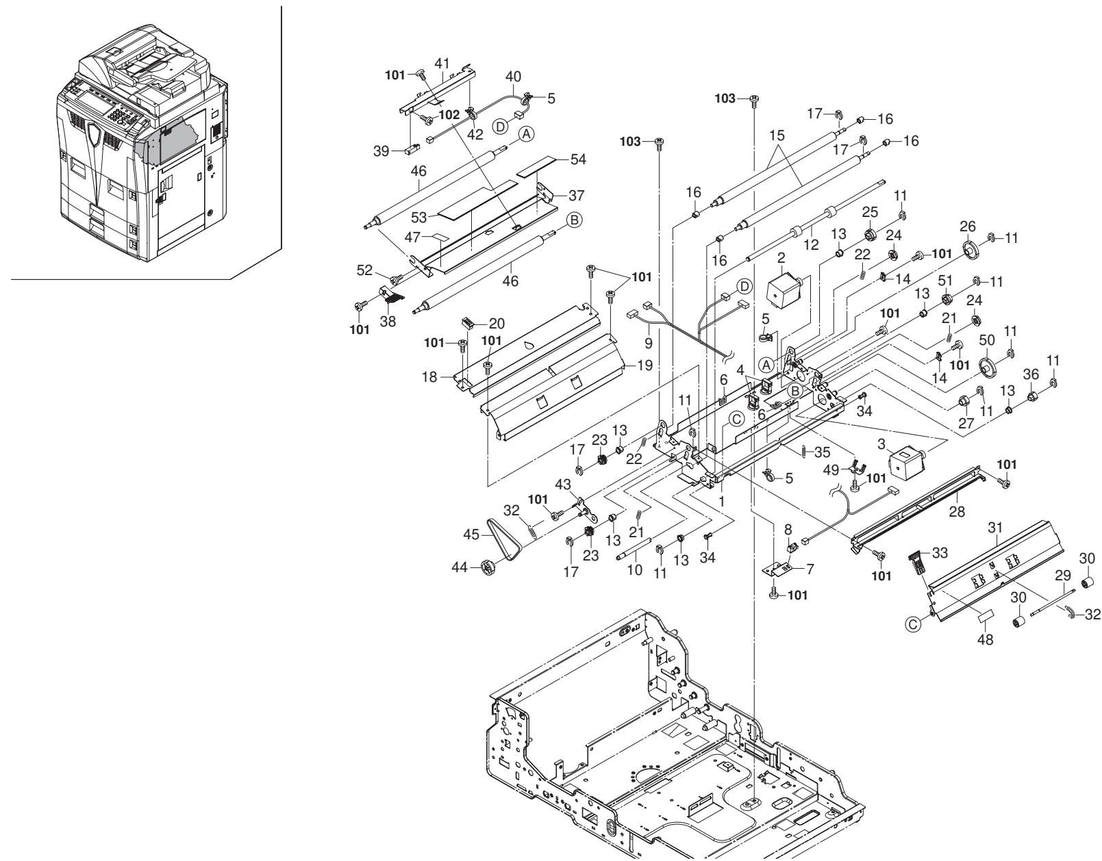
FIG. 13 Paper Conveying II
