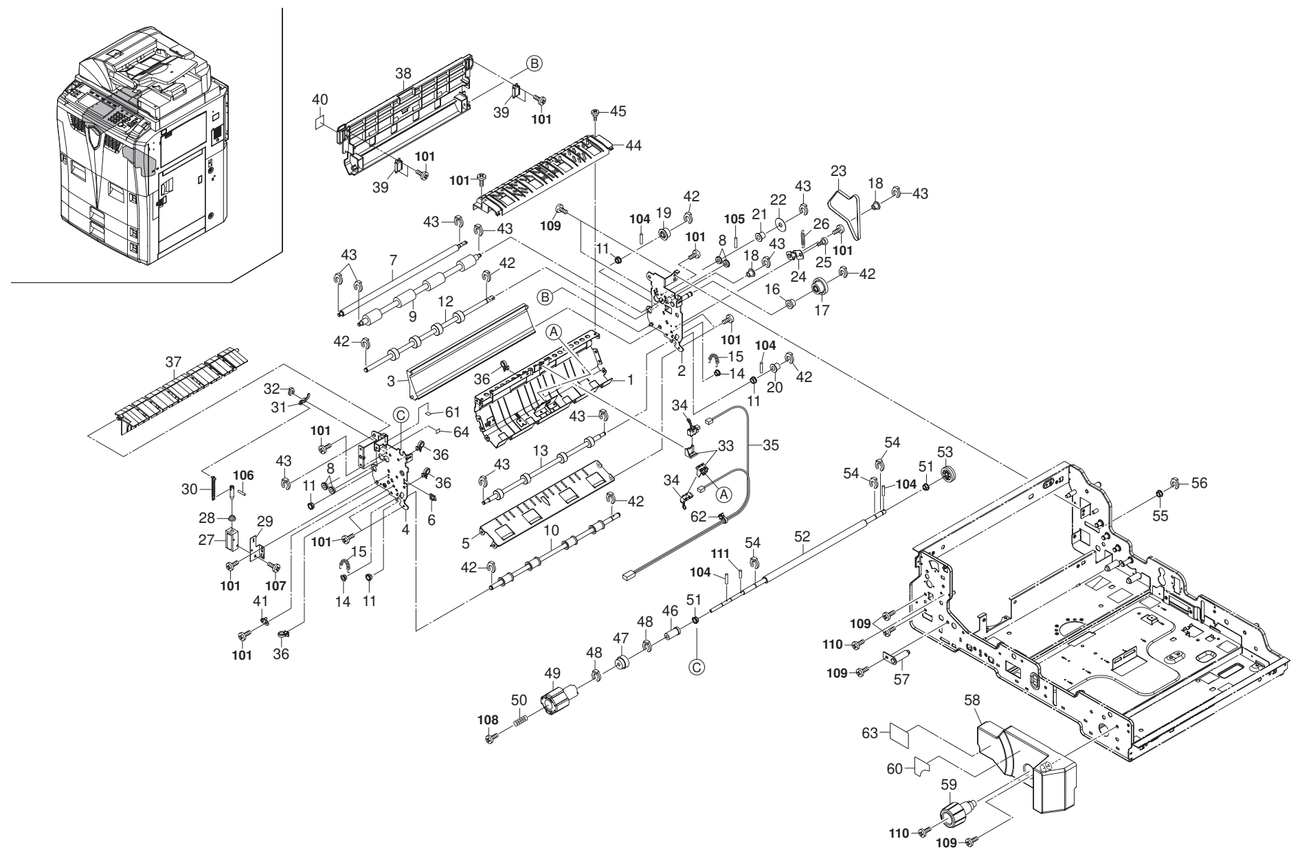
FIG. 14 Paper Conveying III
