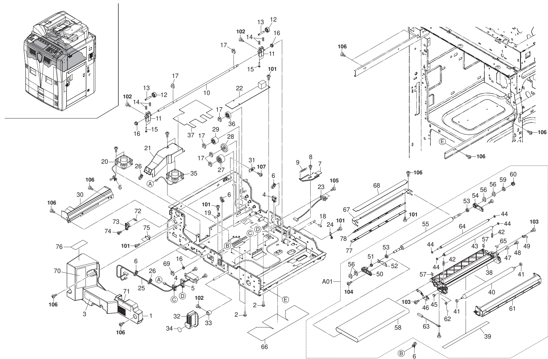
FIG. 12 Paper Conveying I
