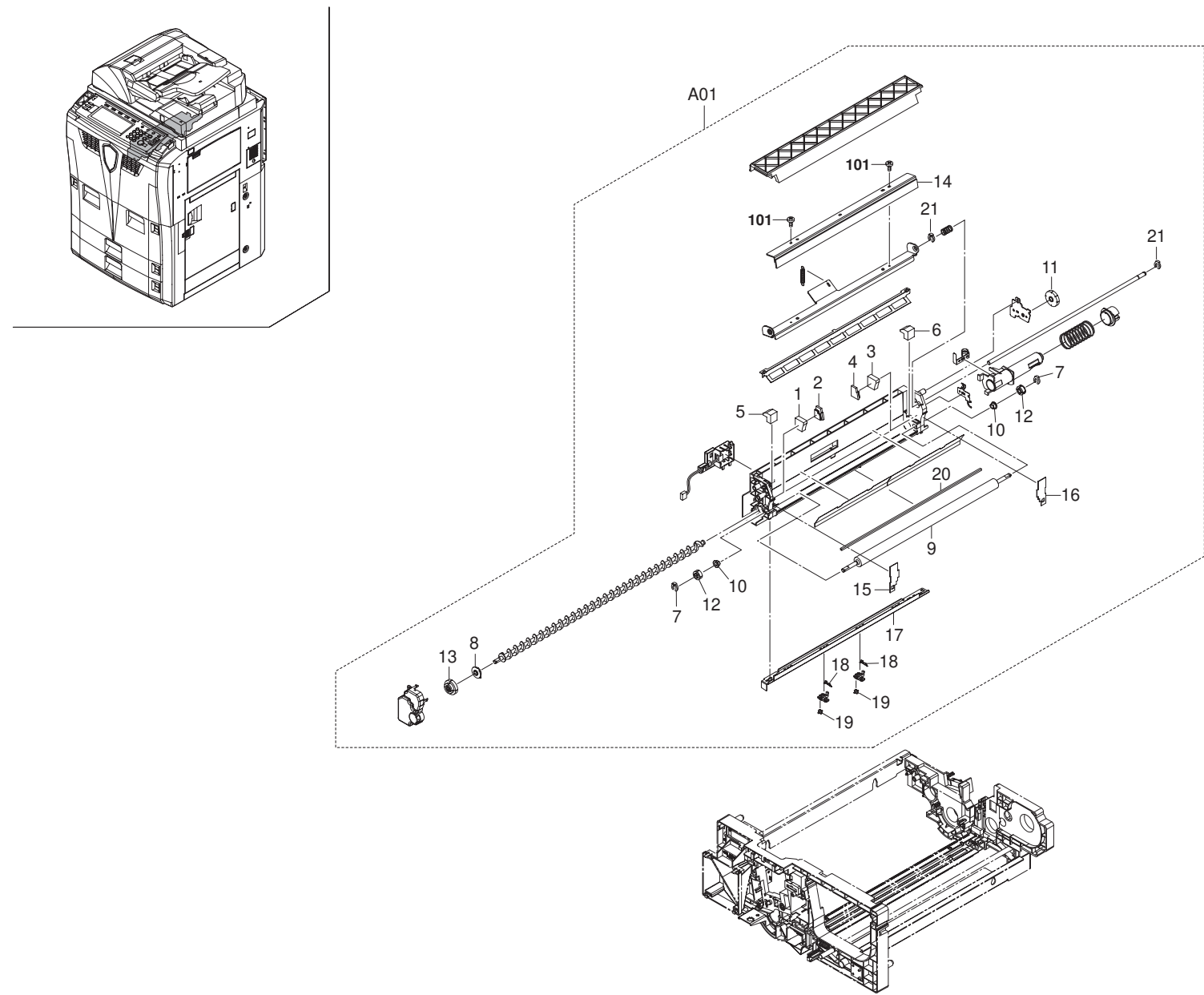
FIG. 19 Cleaning Unit I
