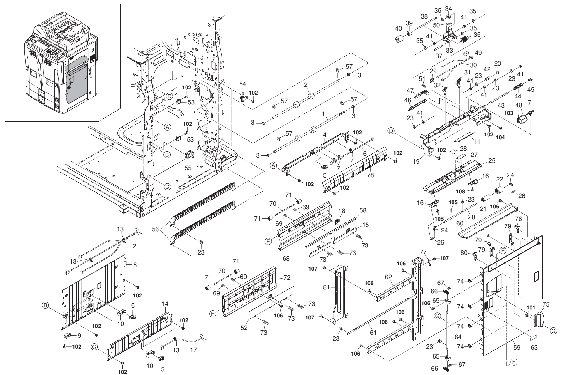
FIG. 9 Paper Feed-in I
