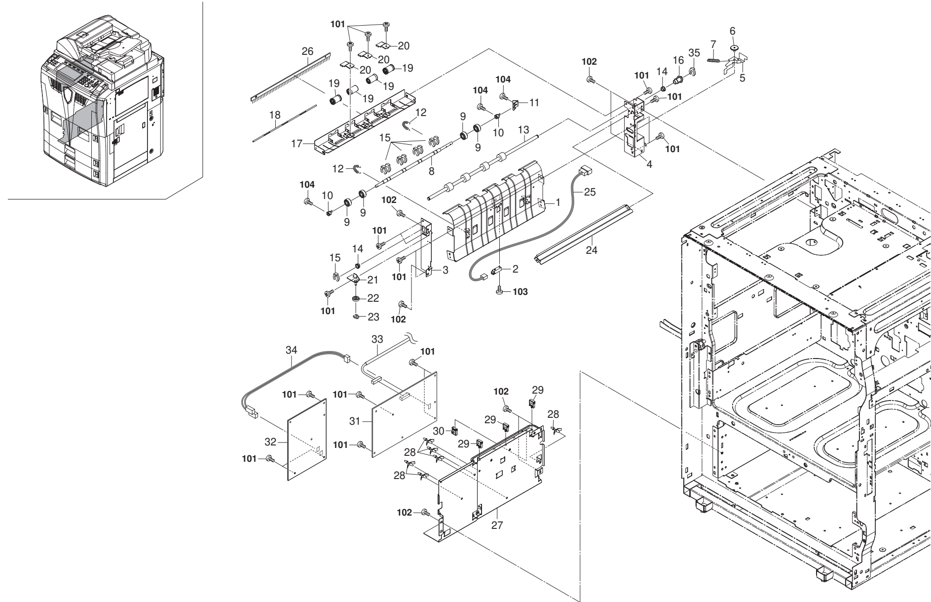
FIG. 29 Paper Eject
