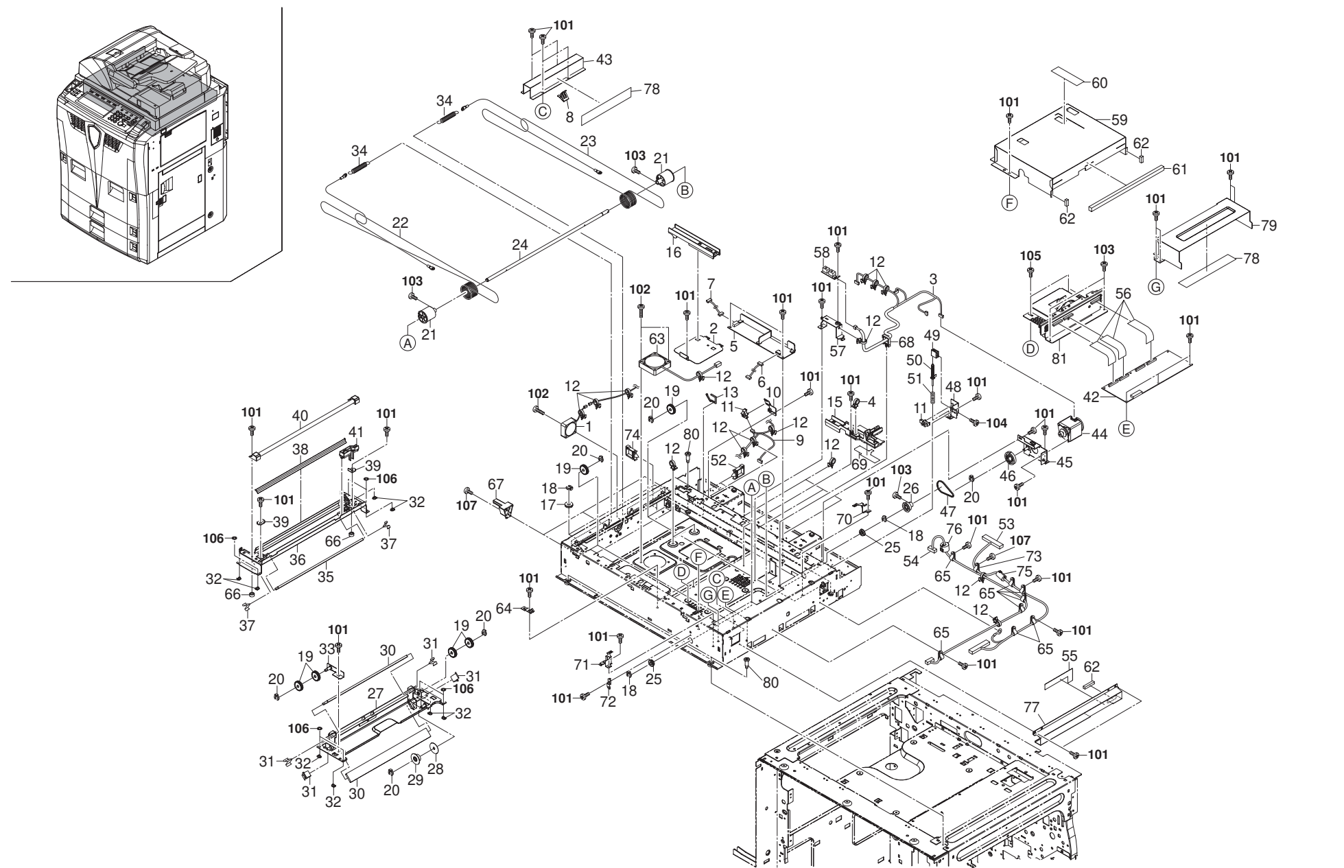
FIG. 15 Optical Section I
