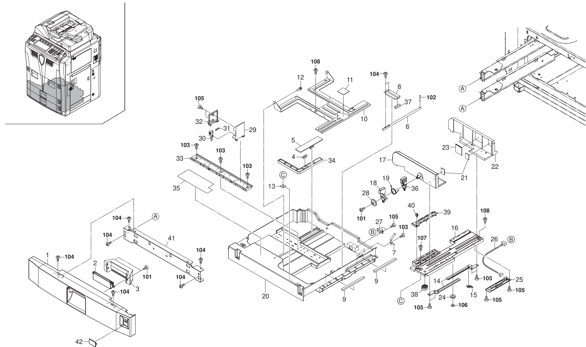
FIG. 4 Paper Cassette
