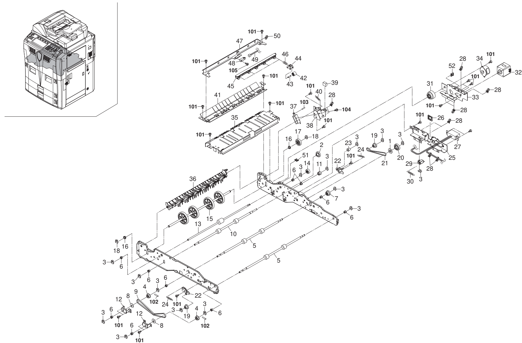
FIG. 27 Duplex Unit II
