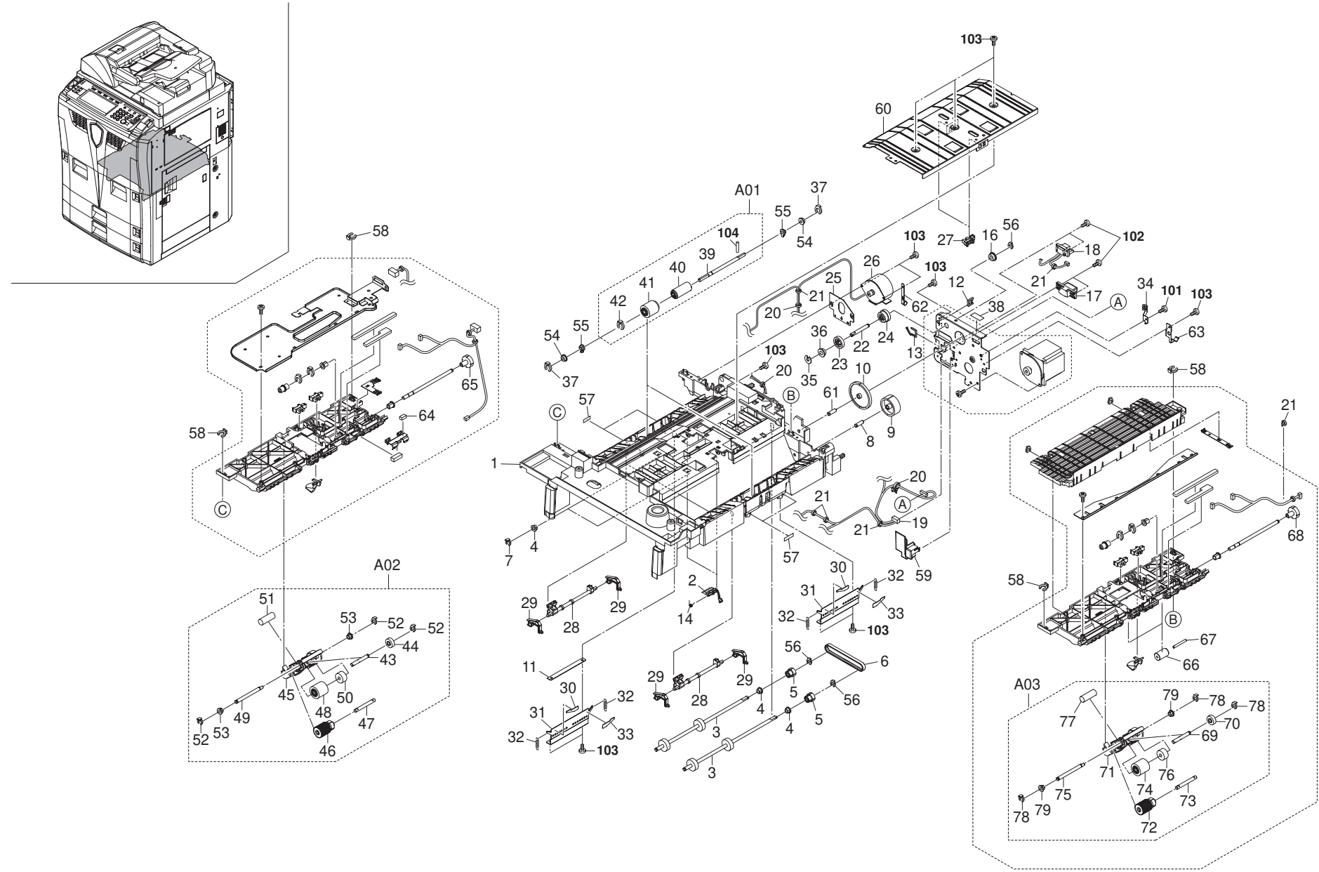
FIG. 7 Deck Feed Section I
