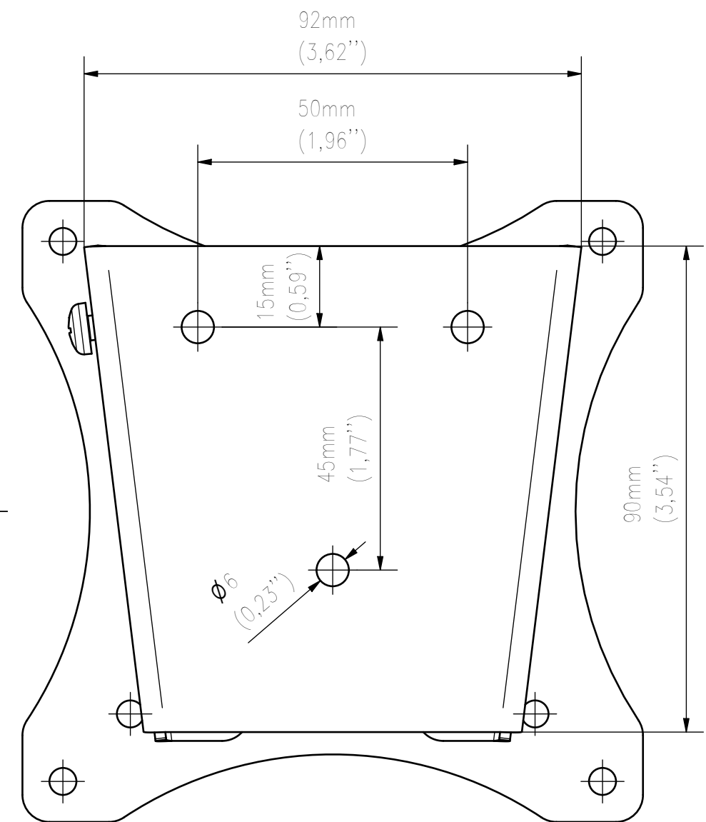
BACK VIEW
