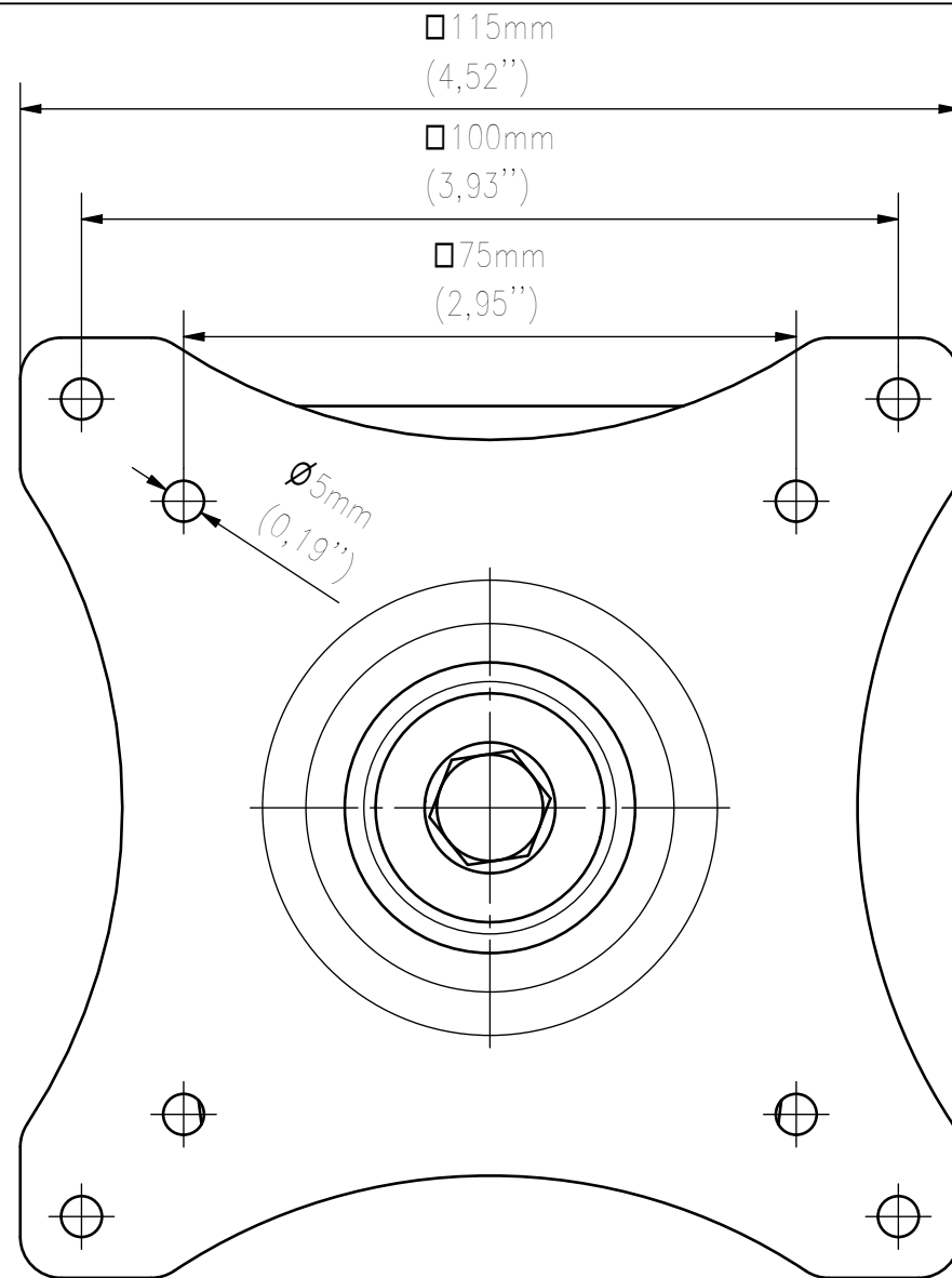
FRONT VIEW
