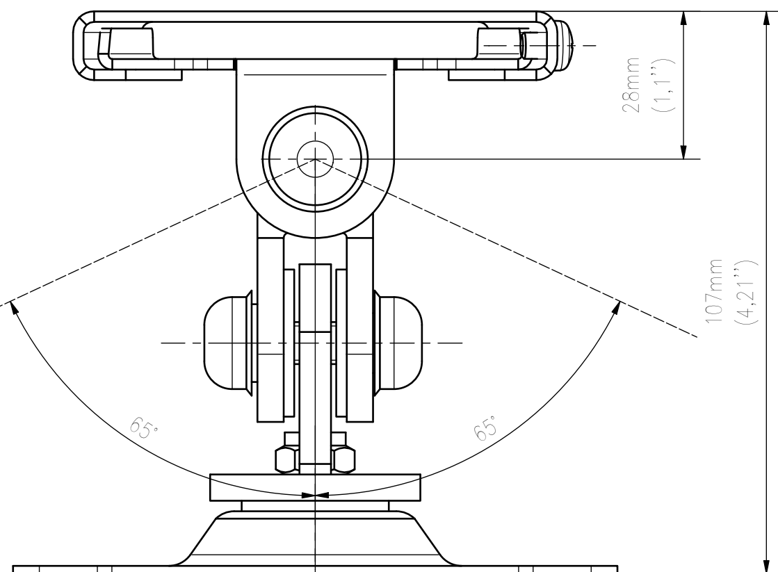
TOP VIEW
