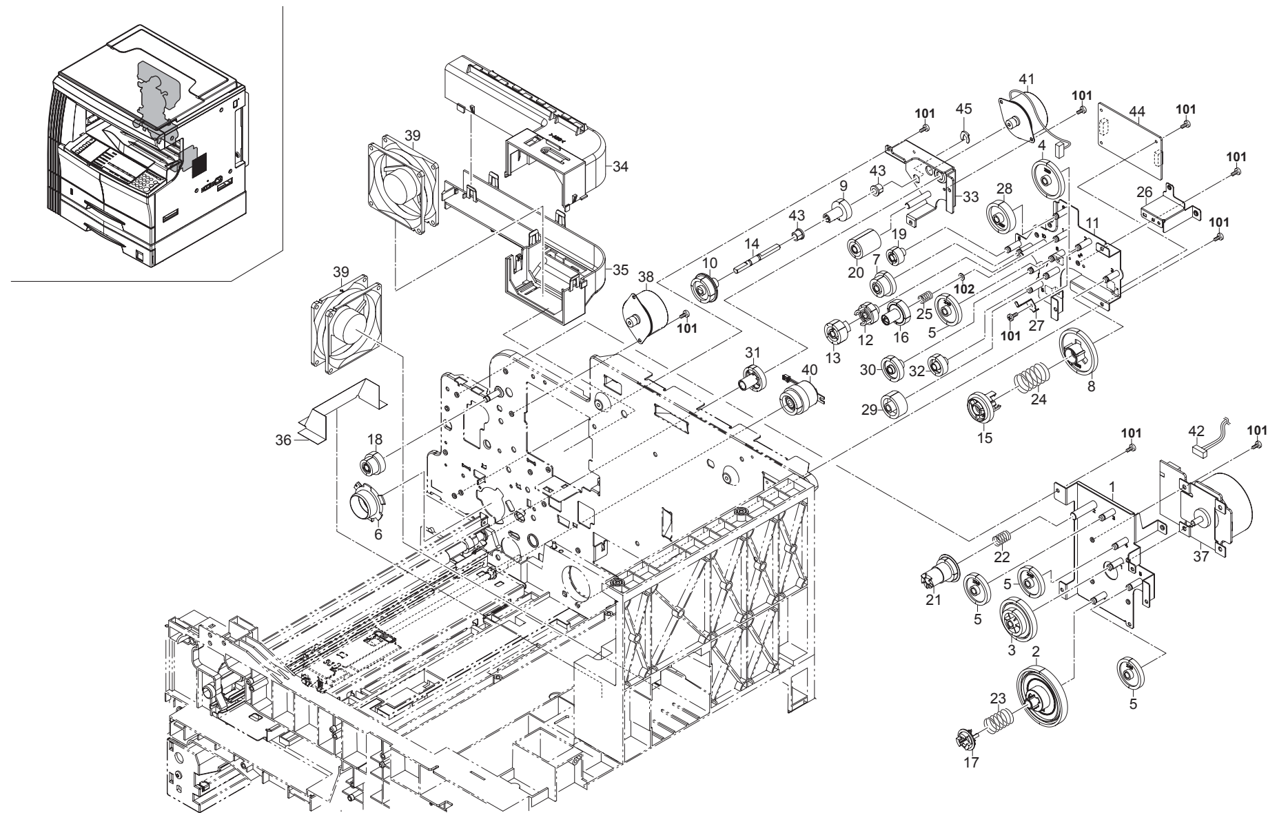
FIG. 13 Driving & Cooling Section
