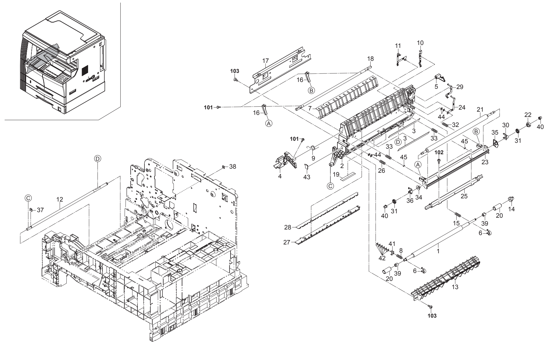
FIG. 6 Conveying Section
