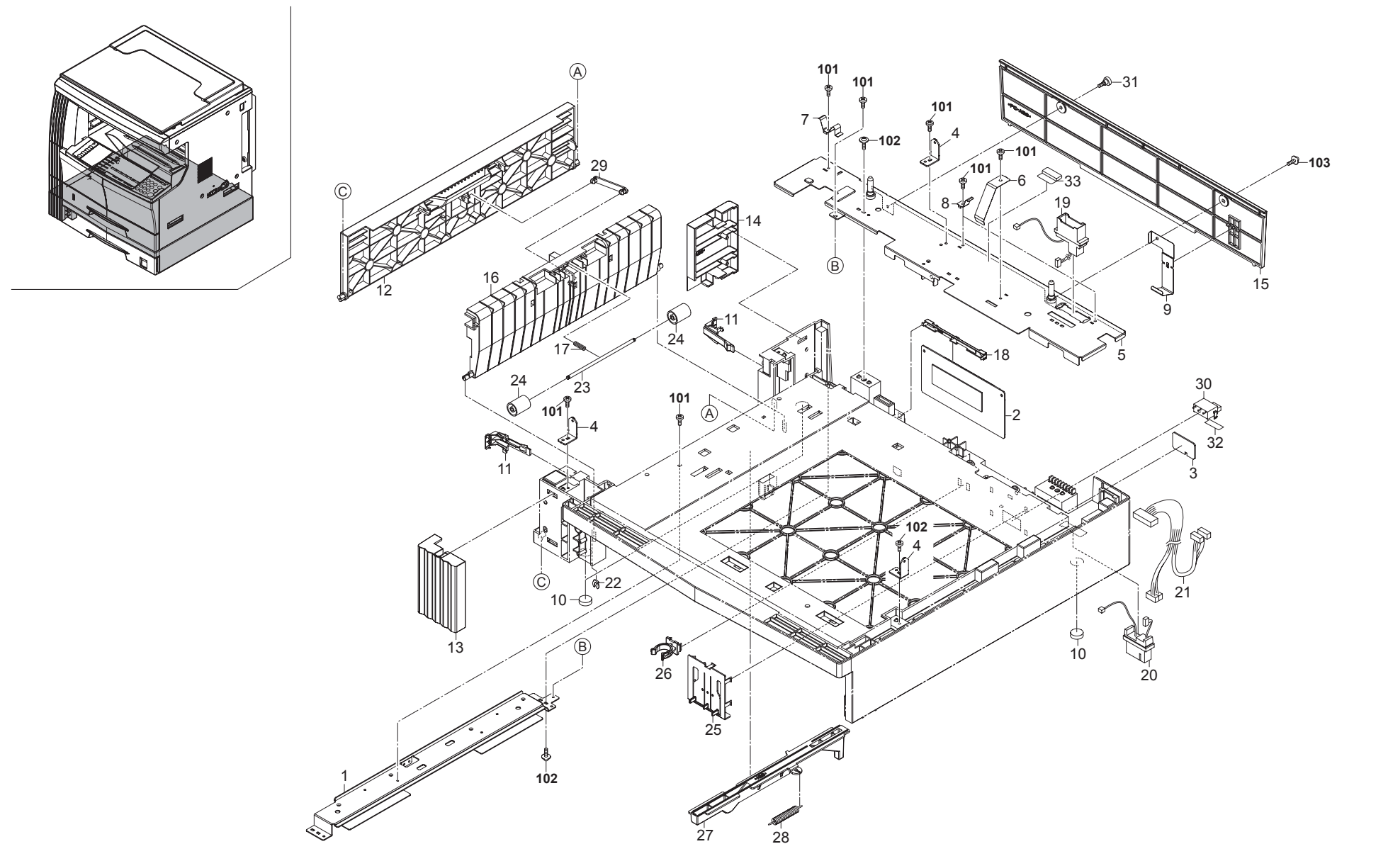
FIG. 3 Exterior Covers (20ppm)
