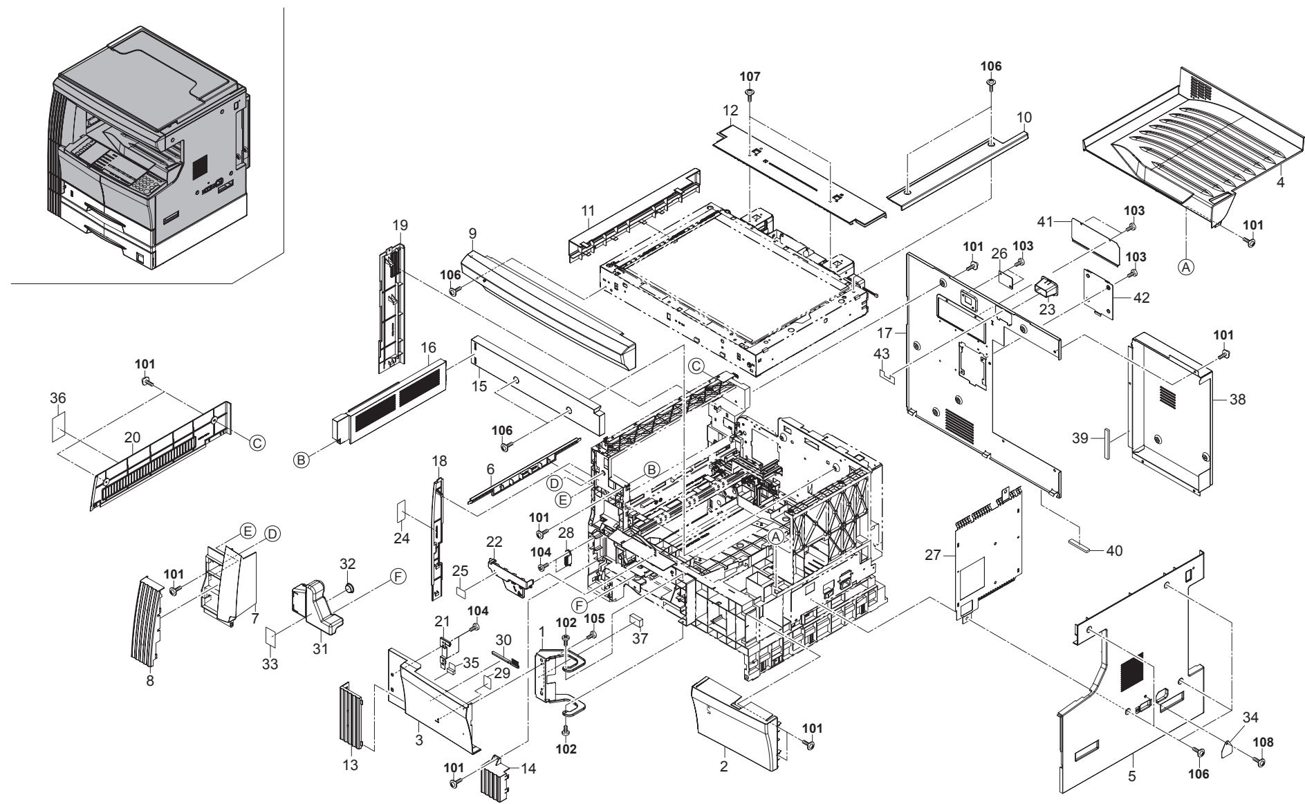
FIG. 1 Exterior Covers
