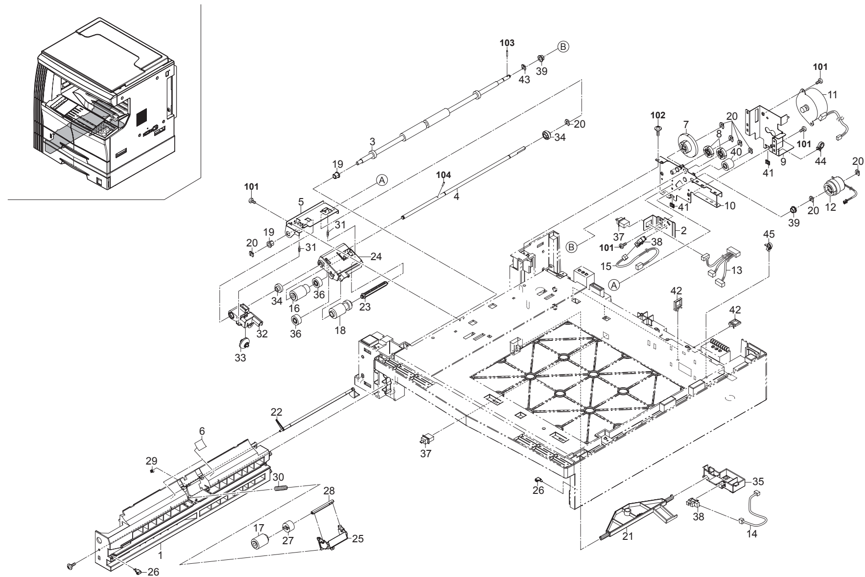
FIG. 4 Paper Feed Section (20ppm)
