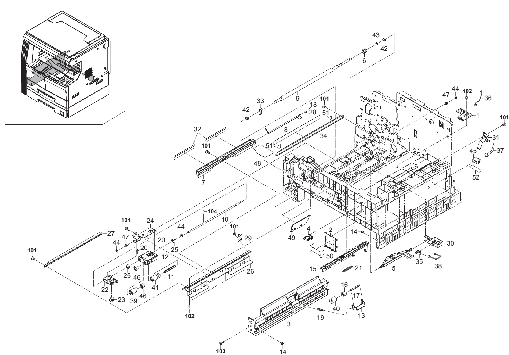
FIG. 7 Paper Feed Section
