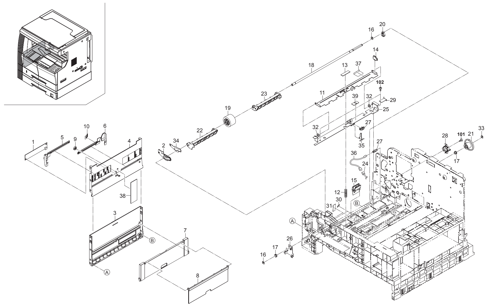
FIG. 8 Bypass Section
