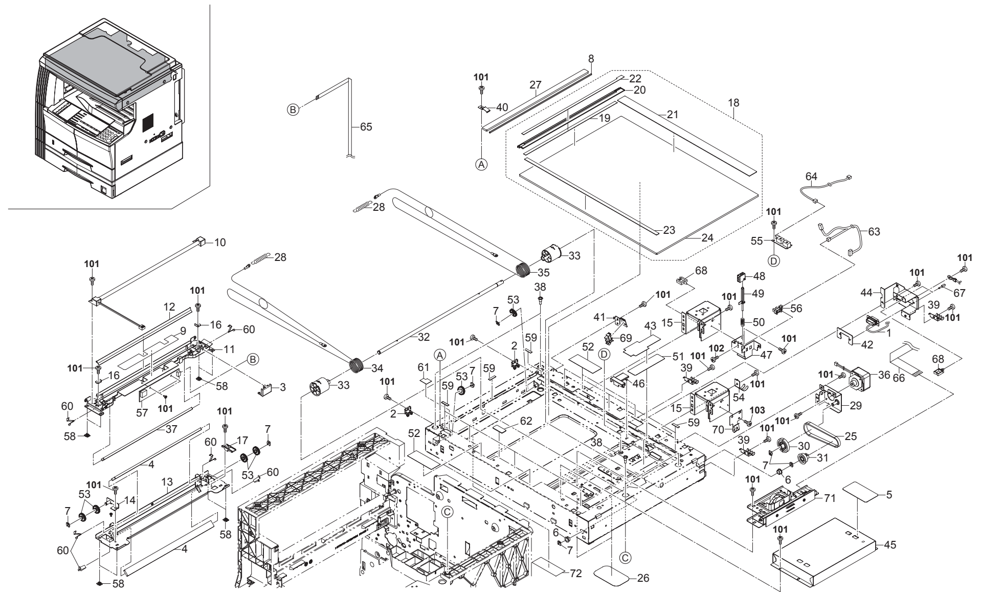
FIG. 10 Scanner Section
