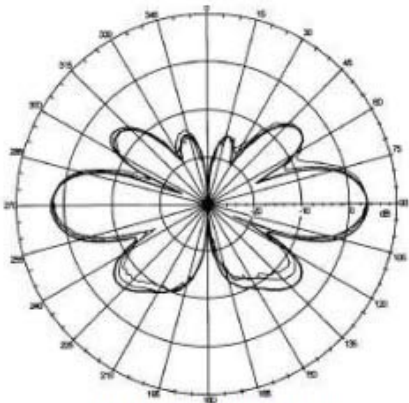
V-Plane Co-polarization
