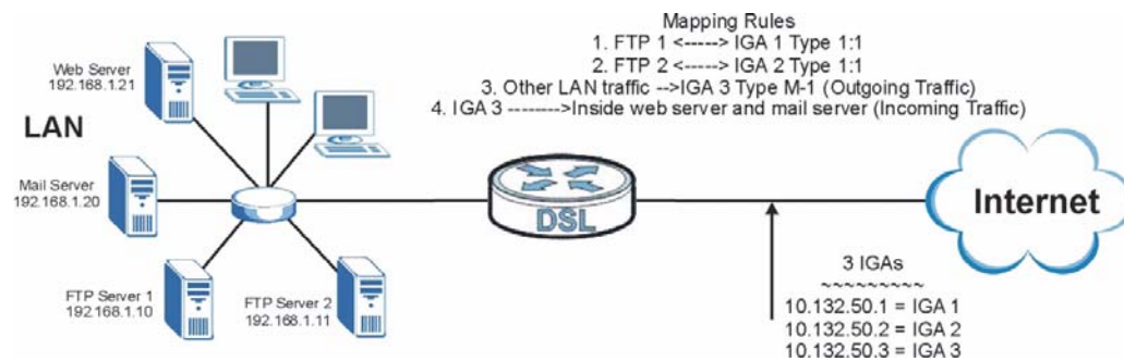
Figure 171 NAT Example 3
