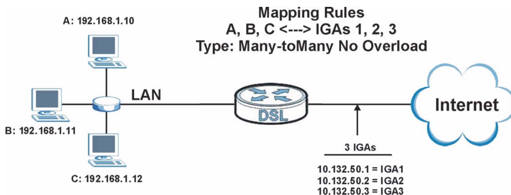
Figure 176 NAT Example 4
