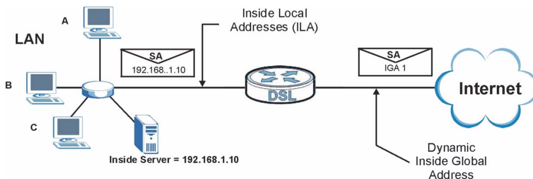
Figure 169 NAT Example 2
