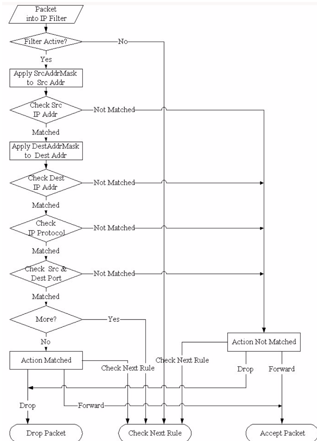
Figure 186 Executing an IP Filter
