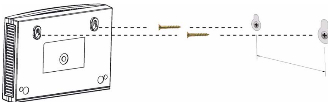
Figure 233 Wall-mounting Example
