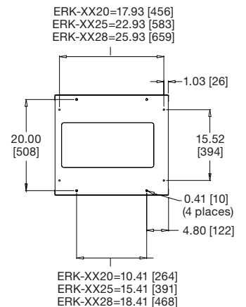
bottom view mounting holes
