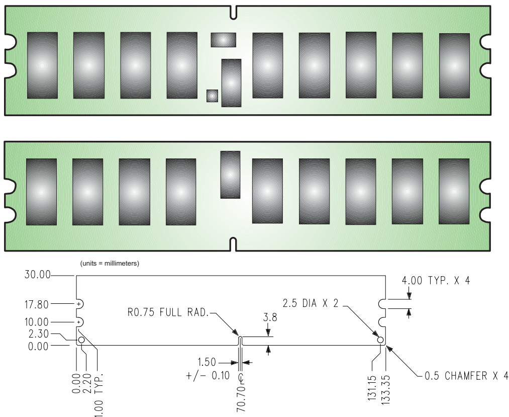
Figure 1: KVR667D2S4P5K2/2G 240-Pin DIMM
