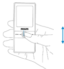
Through list
