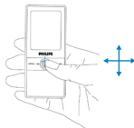
Through menu
