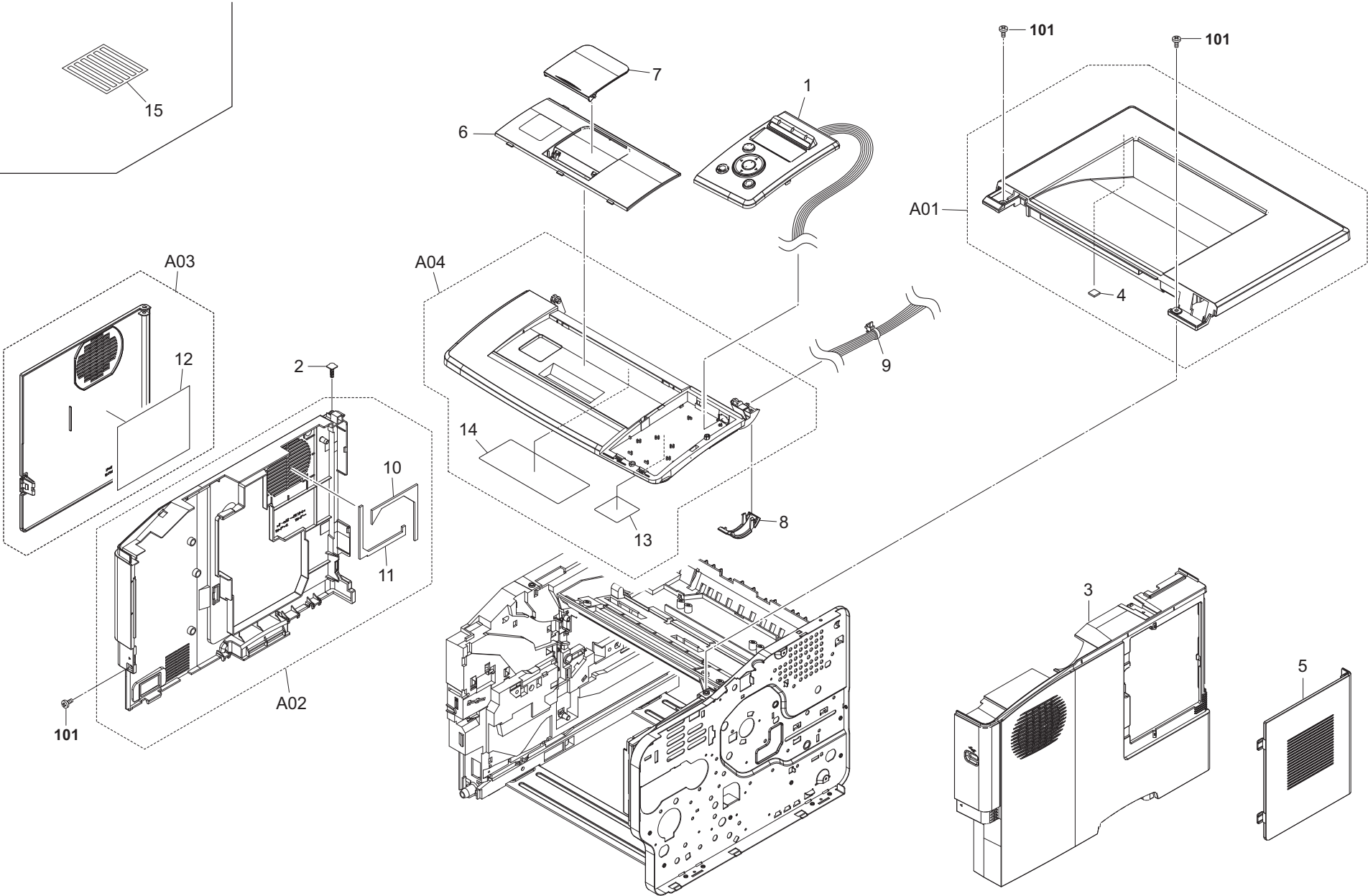
FIG. 1 Covers (FS-2020D)
