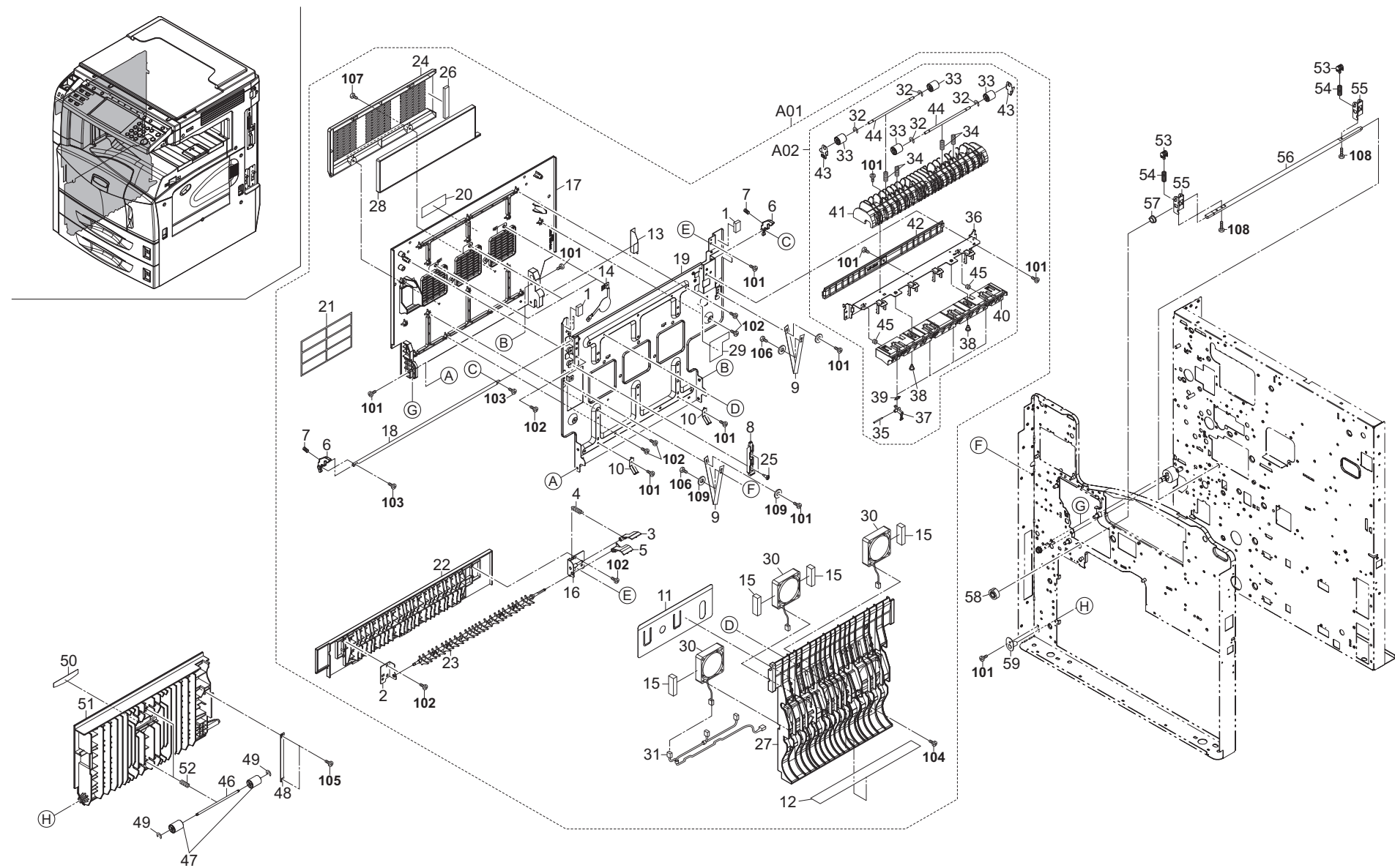
FIG. 6 Paper Feed-In III
