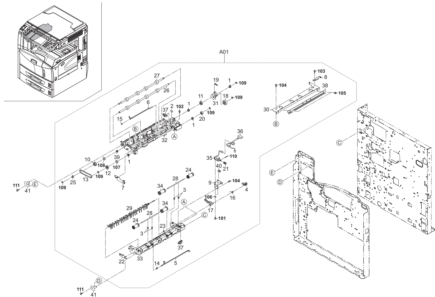
FIG. 8 Paper Exit (120/230/240V)
