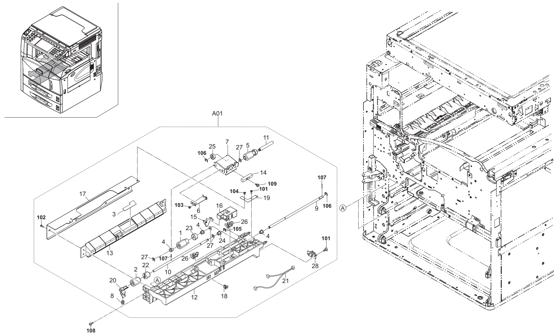
FIG. 4 Paper Feed-In I
