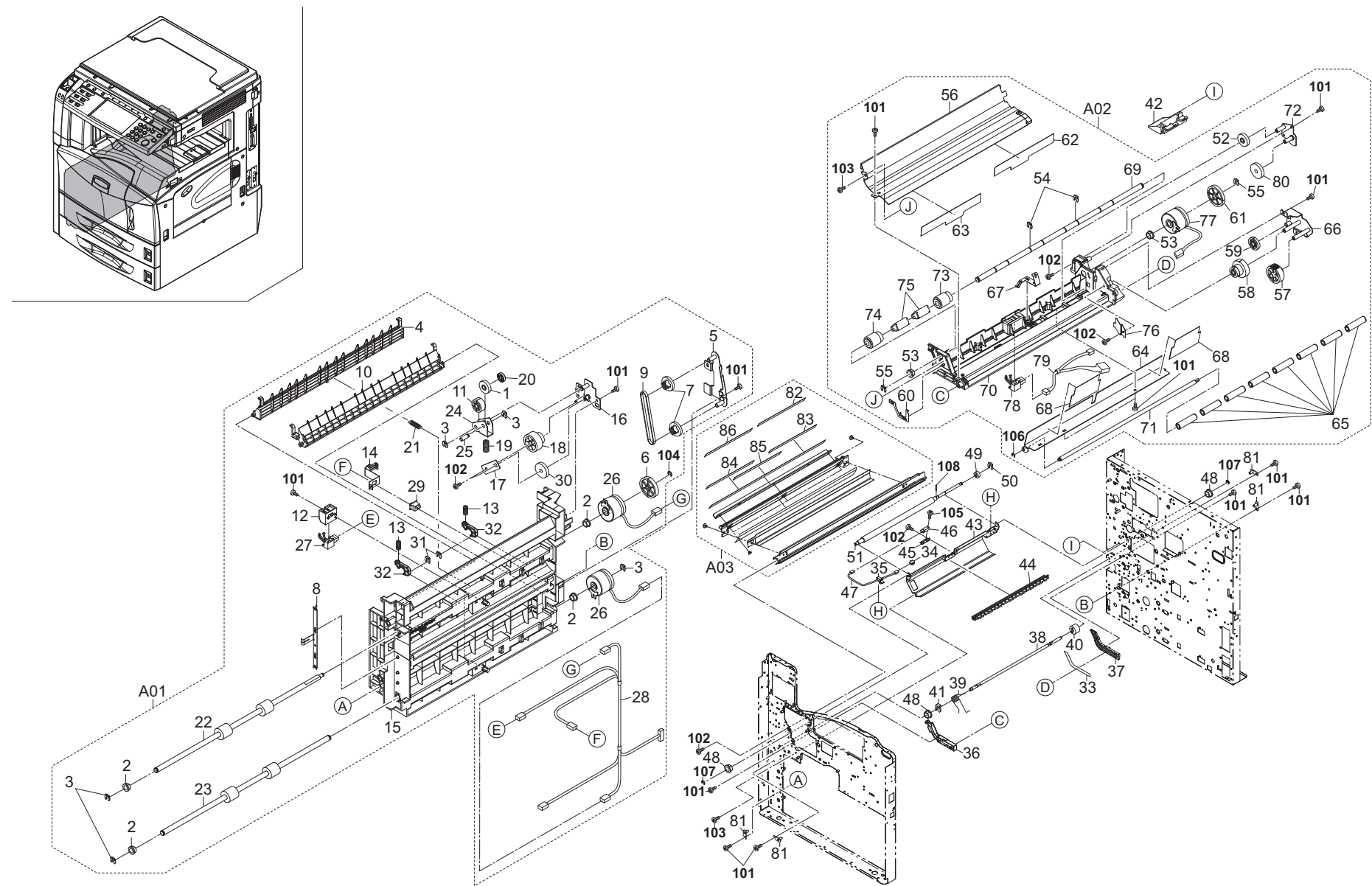
FIG. 5 Paper Feed-In II
