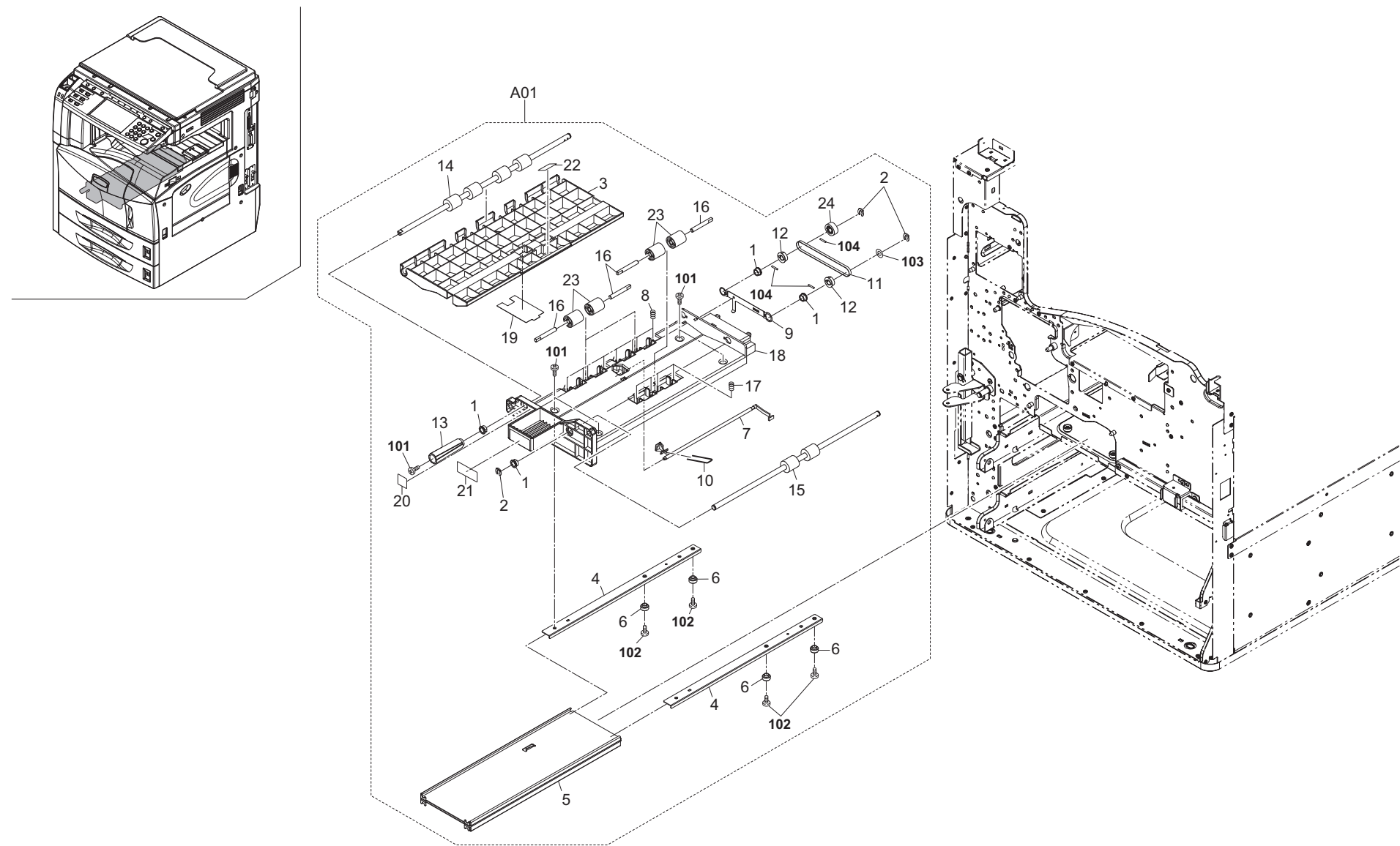
FIG. 12 Bypass Feed Unit
