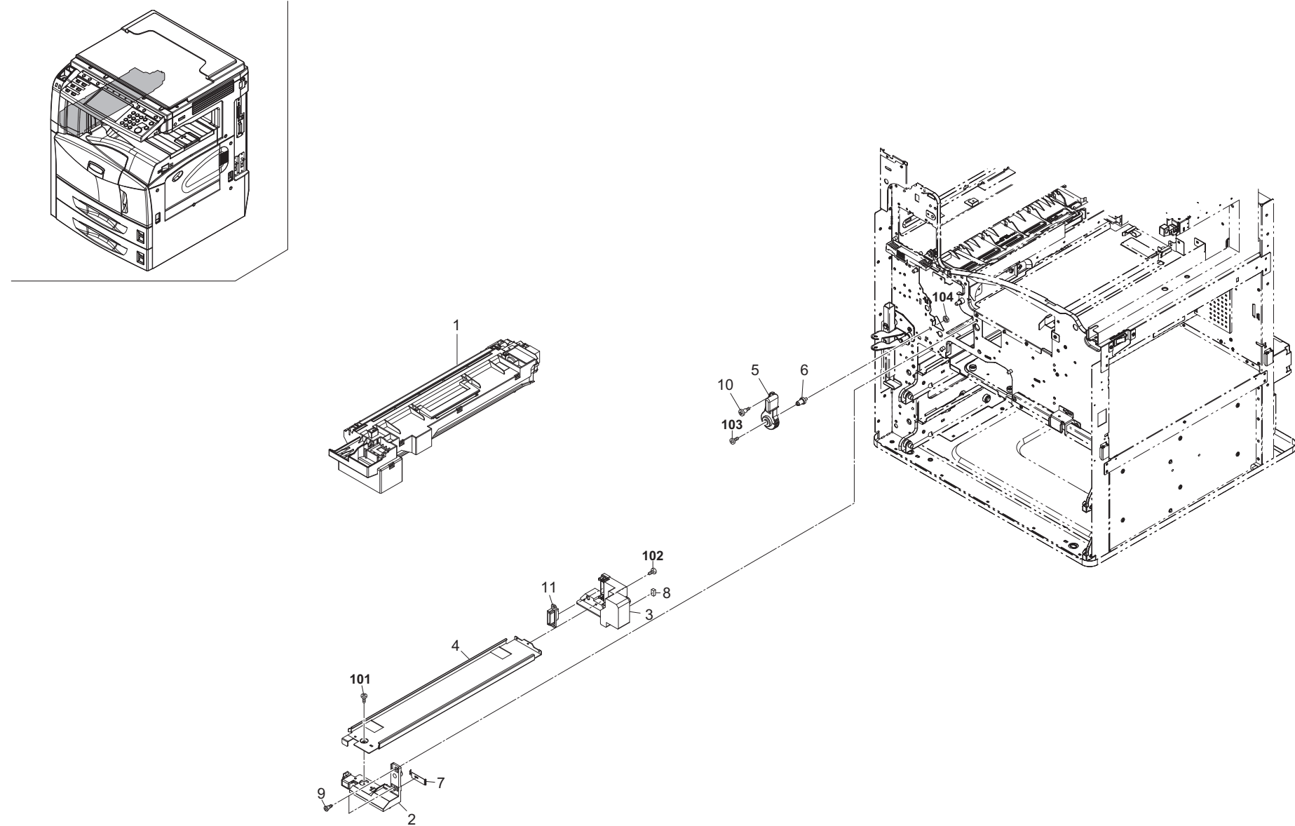
FIG. 14 Developer Unit
