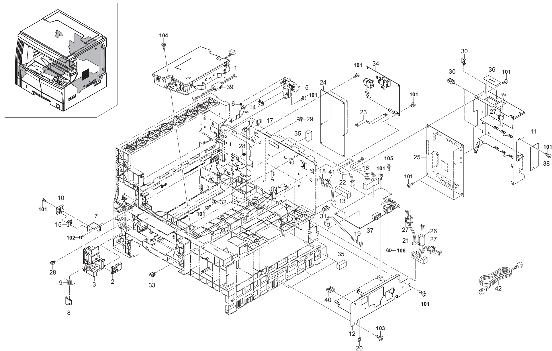
FIG. 12 Electrical Components
