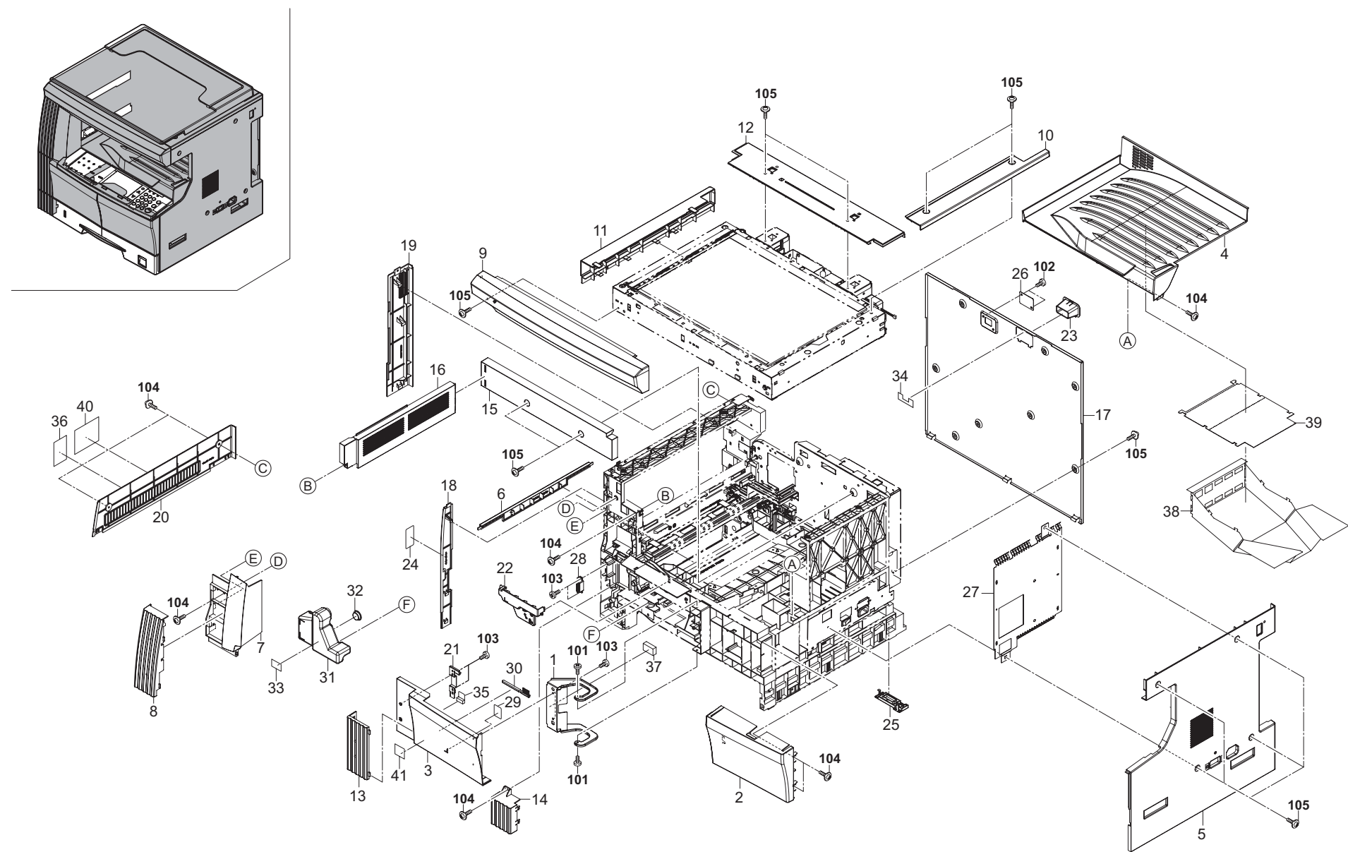
FIG. 1 Covers
