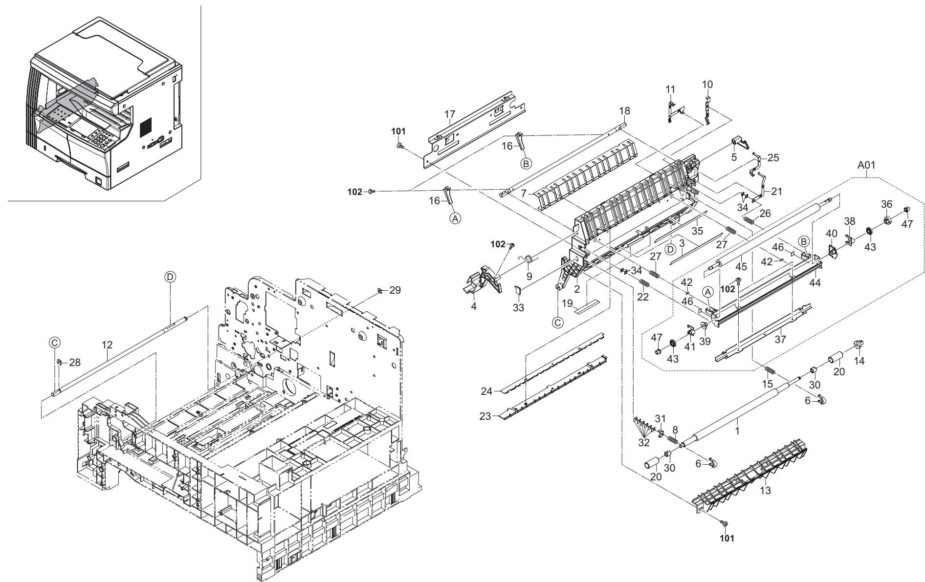
FIG. 4 Conveying
