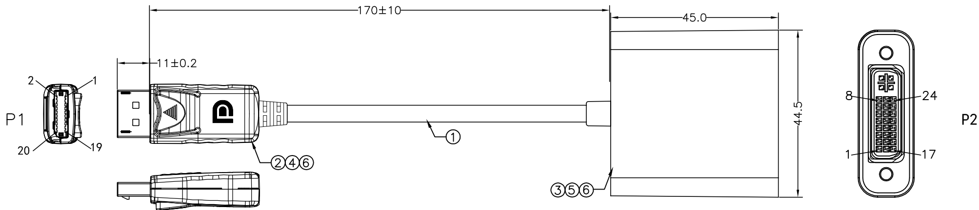
Pin Assignment
