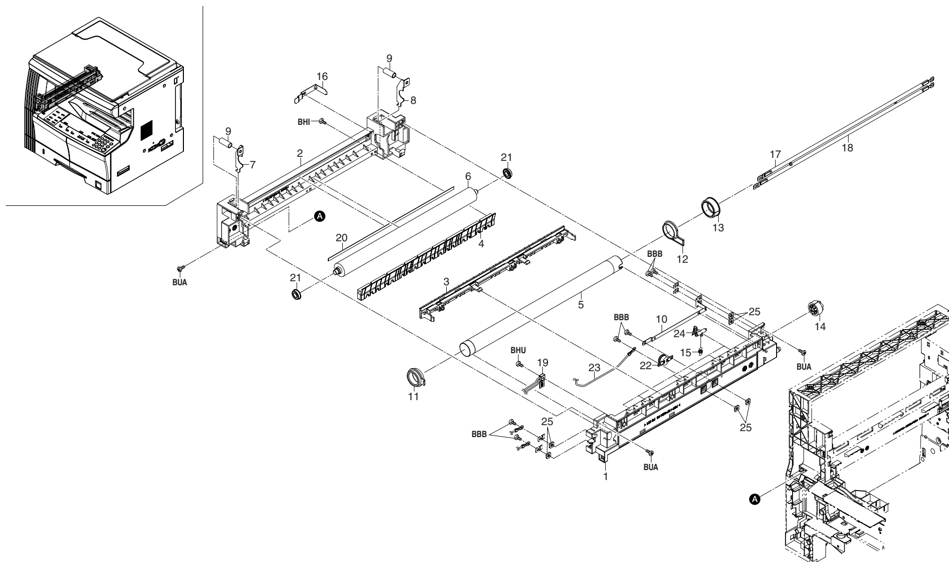
FIG. 10 FUSER UNIT
