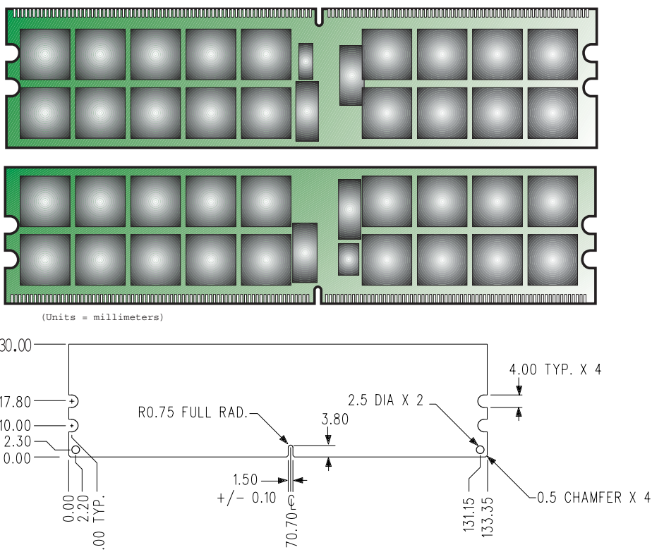
Figure 1: KVR667D2D4P5/4GI 240-Pin DIMM
