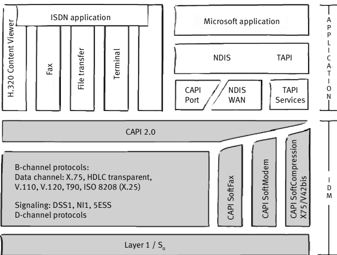
ISDN driver model (IDM)
