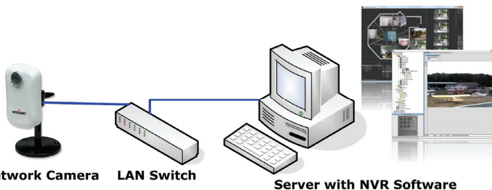
Server with NVR Software
