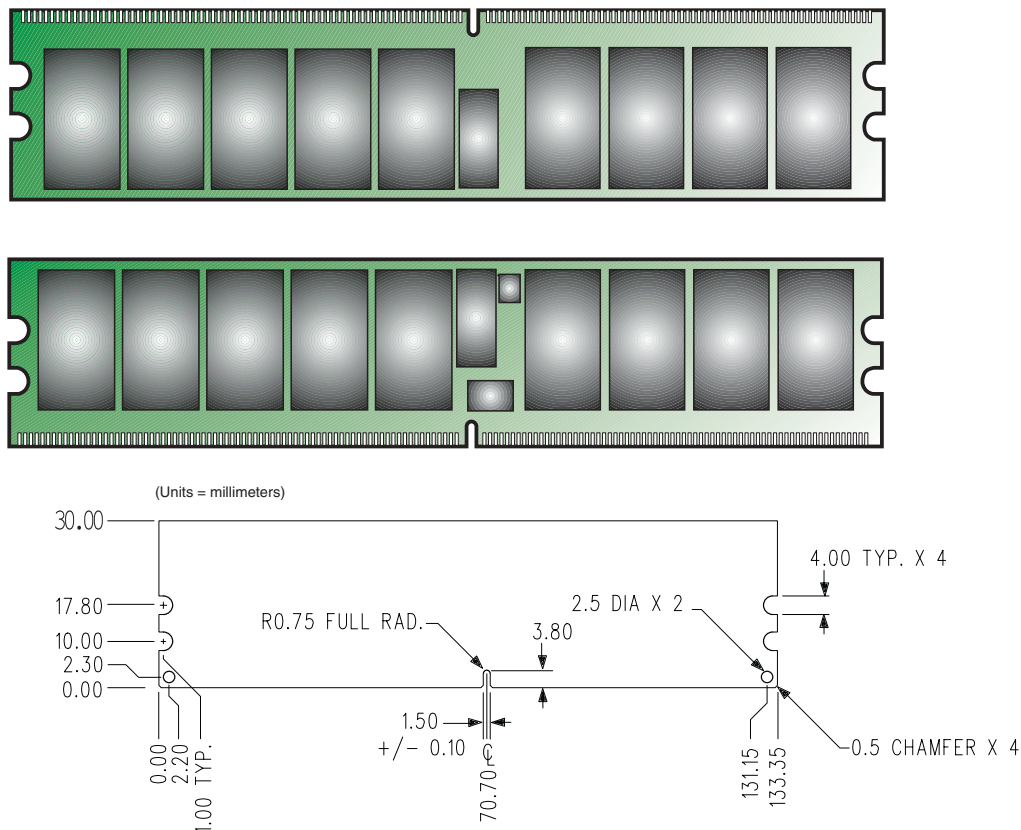
Figure 1: KVR800D2D8P6/4G 240-Pin DIMM
