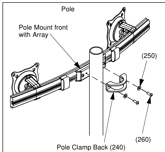
Figure 5: Assemble Array Rail to Pole
