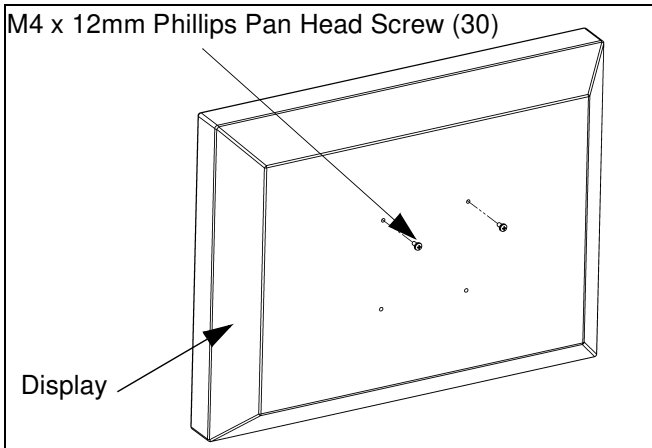
Figure 6: Prepare Display
