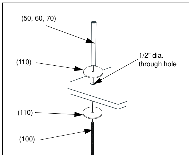
Figure 2: Grommet installation
