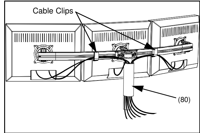
Figure 16: Cable Management
