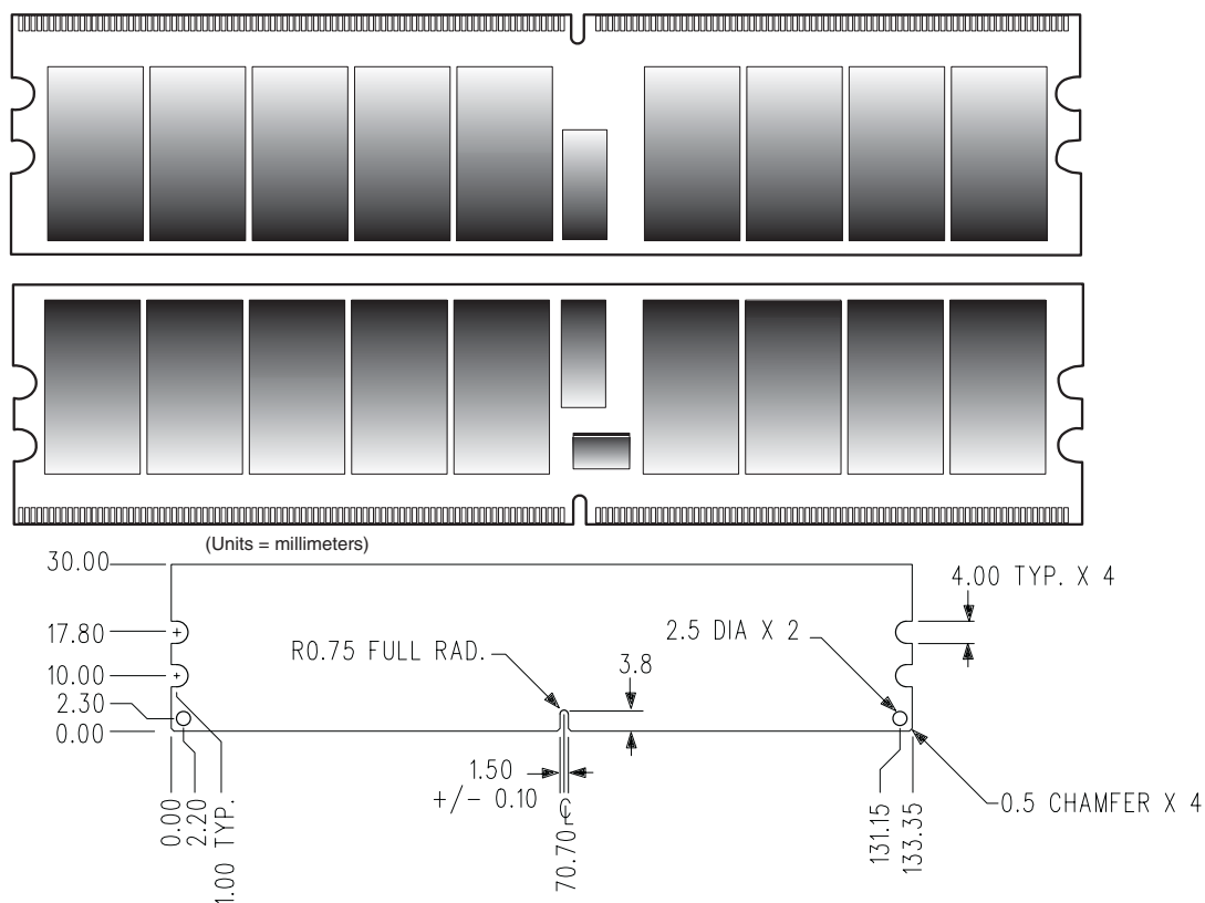
Figure 1: KVR400D2S4R3/2GEF 240-Pin DIMM
