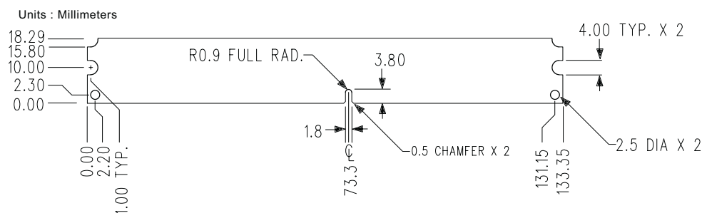
Figure 1: KVR333S4R25L/1G 184-Pin DIMM
