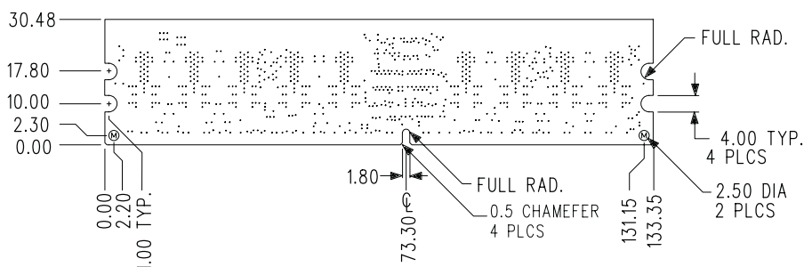
Figure 1: KVR333S4R25/512I 184-Pin DIMM
