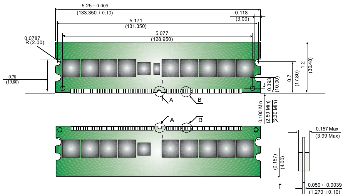
Figure 1: KVR333S4R25/1GI 184-Pin DIMM
