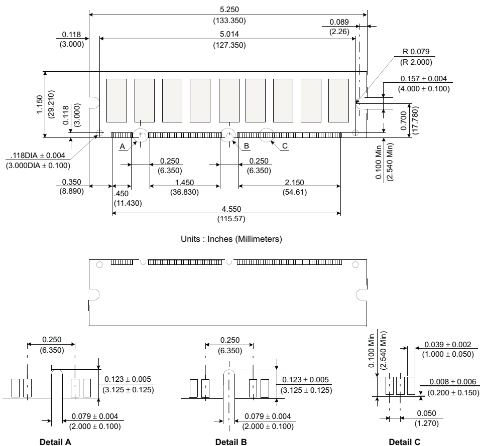
Figure 1: KVR133X72C3/128 168-Pin SDRAM Module
