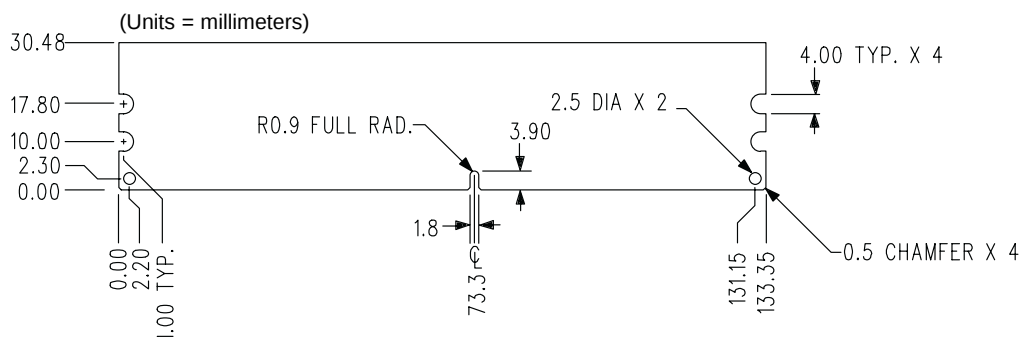
Figure 1: KVR400D4R3A/2G 184-Pin DIMM
