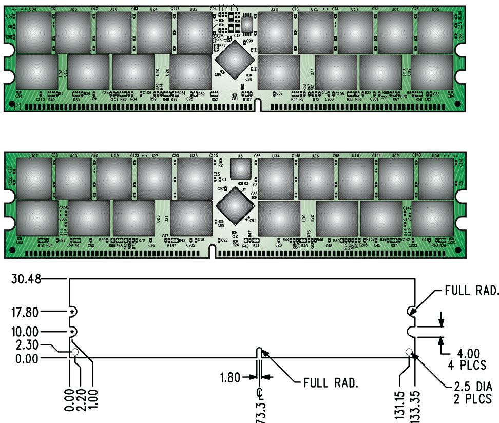
Figure 1: KVR333X72BRC25/2G 184-Pin DIMM
