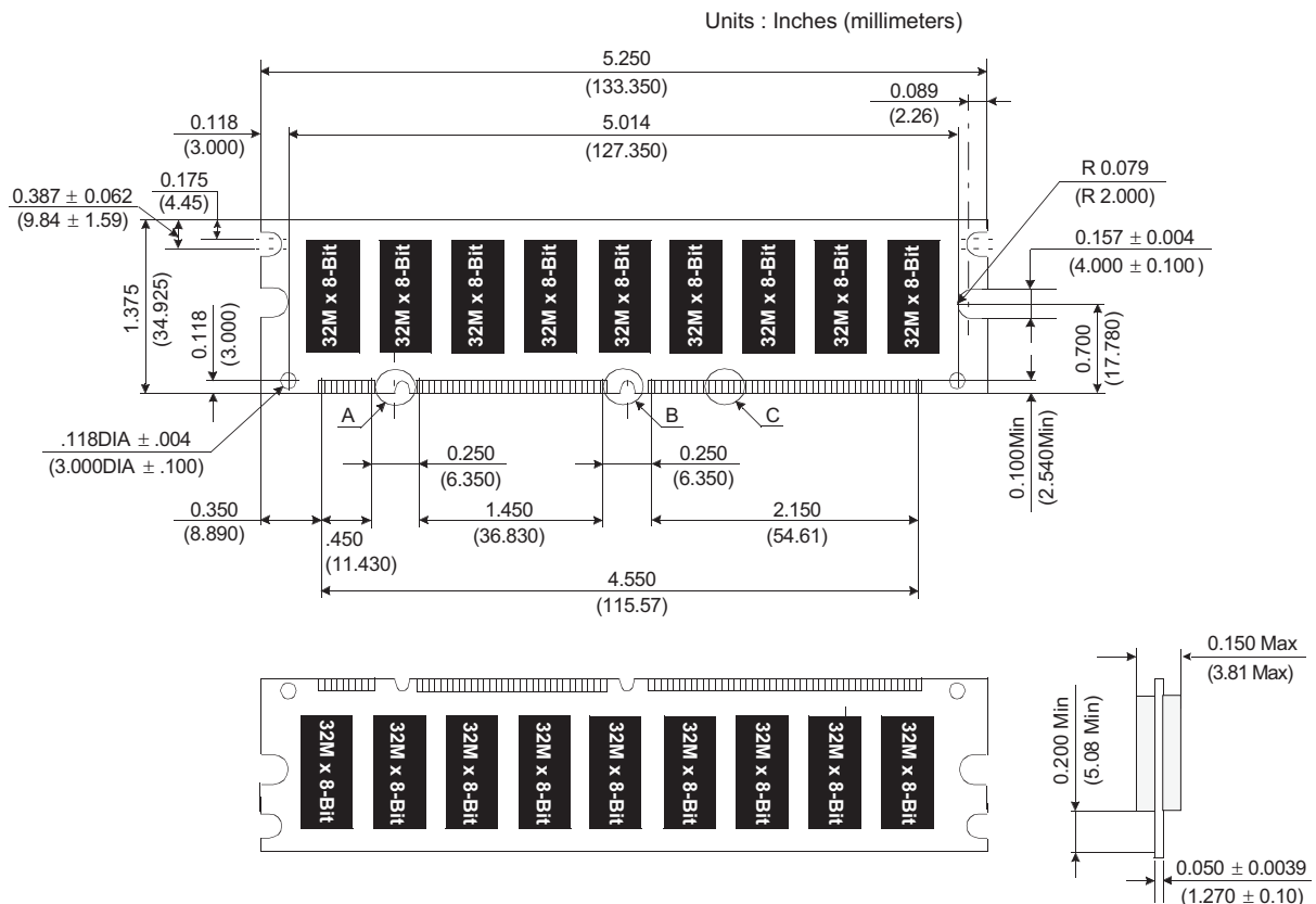
Figure 1: KVR133X72C3/512 168-Pin SDRAM Module
