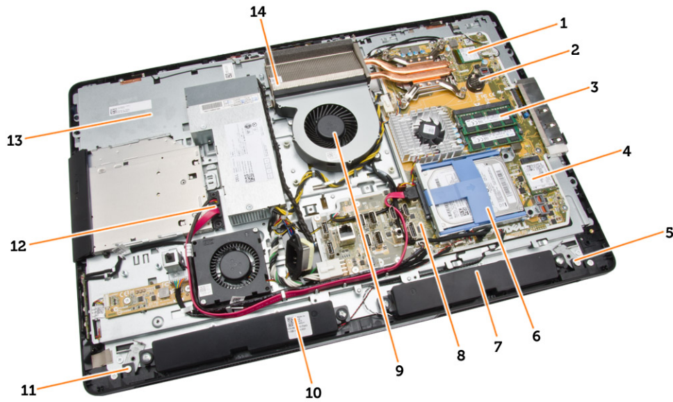
Figure 2. Inside View – 2
