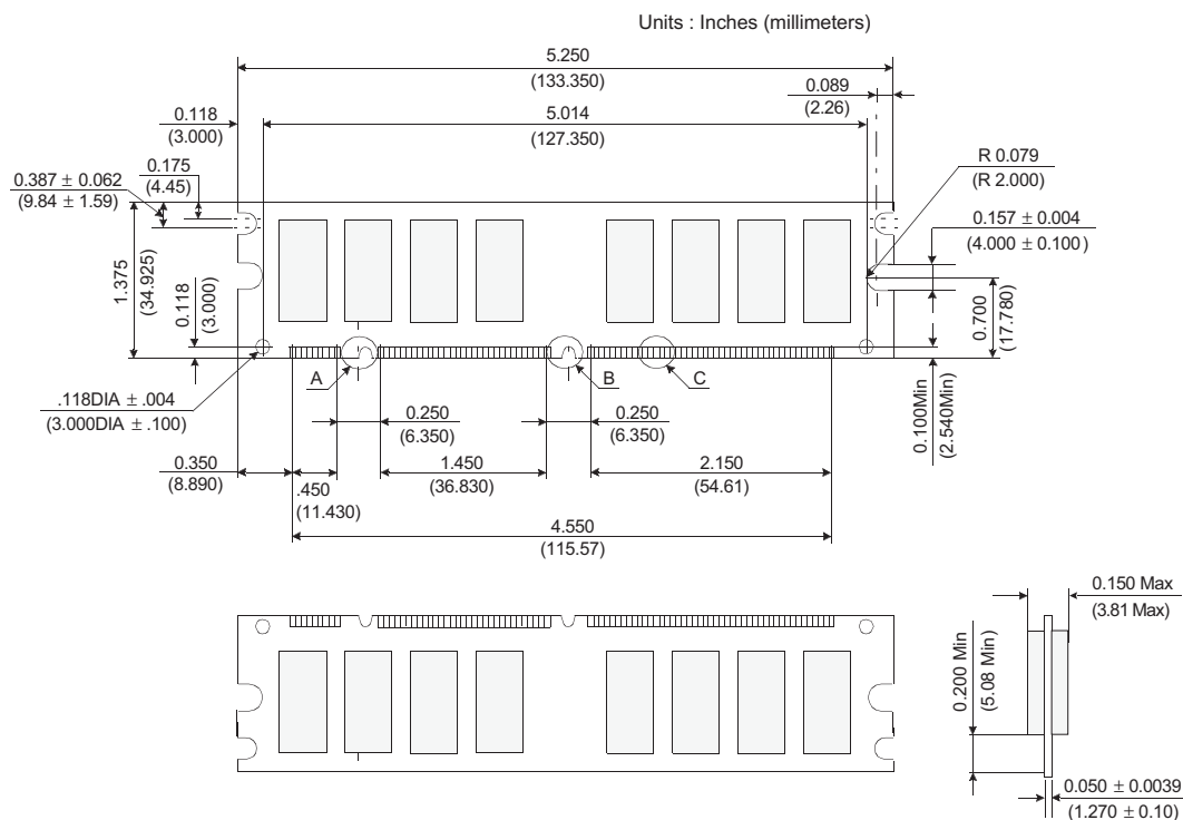
Figure 1: KVR100X64C2/128 168-Pin SDRAM Module
