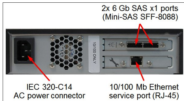
Figure 5. Rear view of the TS2270, TS2260, and TS2250
