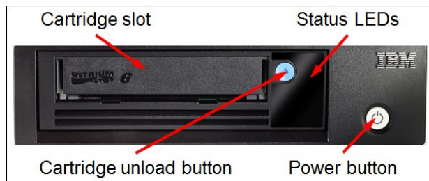
Figure 4. Front view of the TS2260
