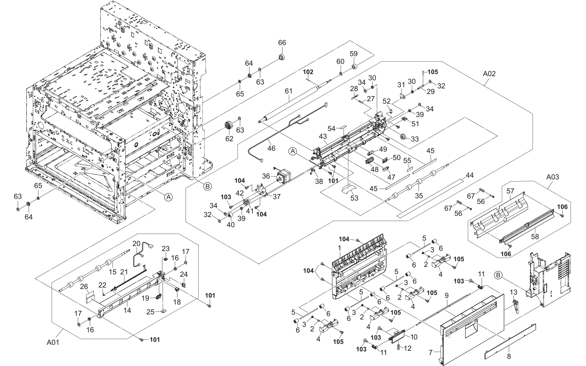
FIG. 7 Paper Feed Section 2
