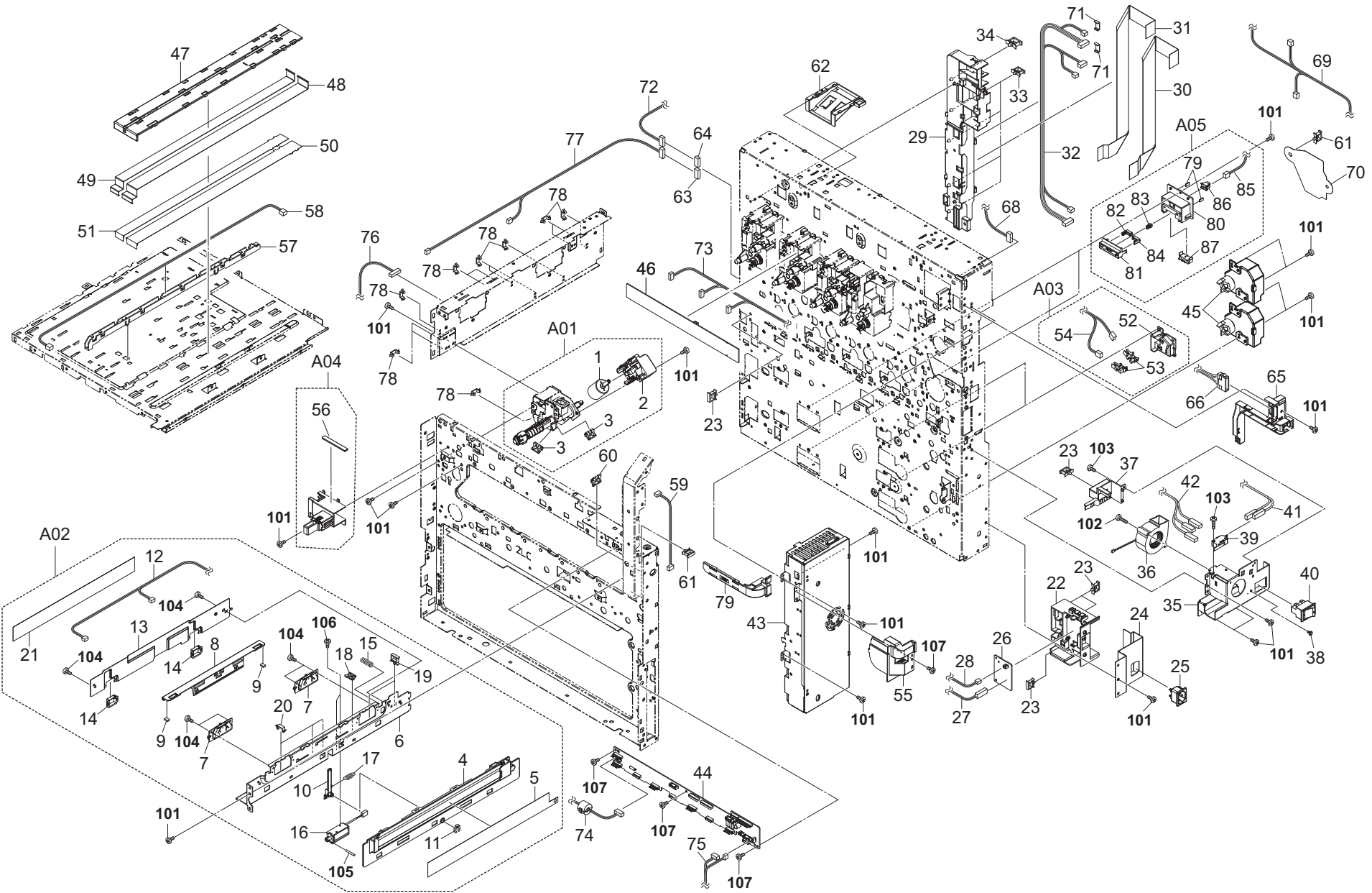
FIG. 21 Electrical Components 1
