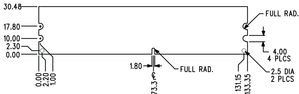
Figure 1: KVR266D4R25/1GI 184-Pin DIMM
