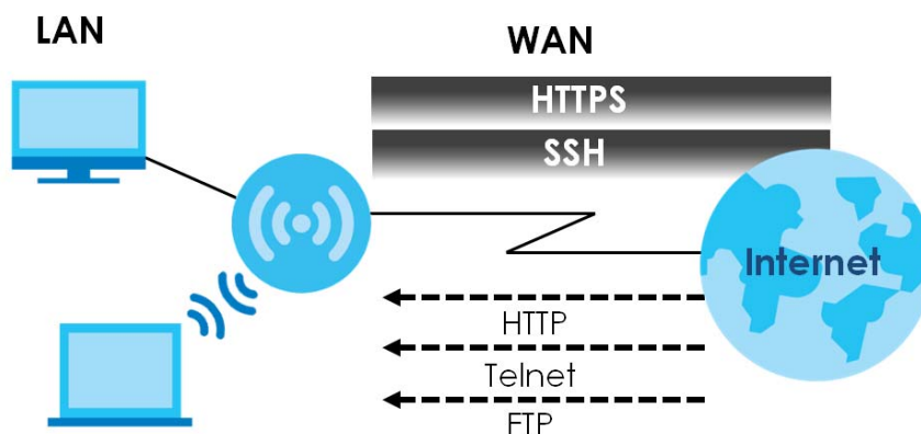
Figure 110 Secure and Insecure Service Access From the WAN
