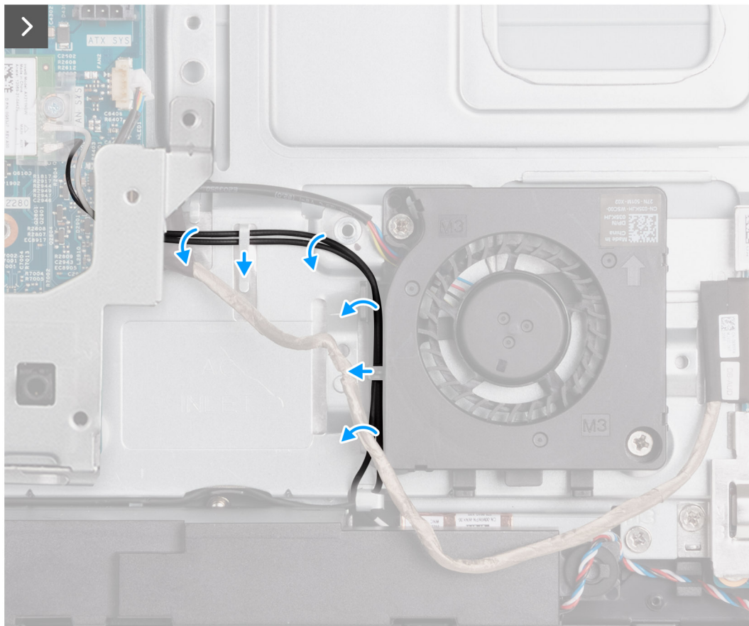
Figure 52. Removing the power-supply fan
