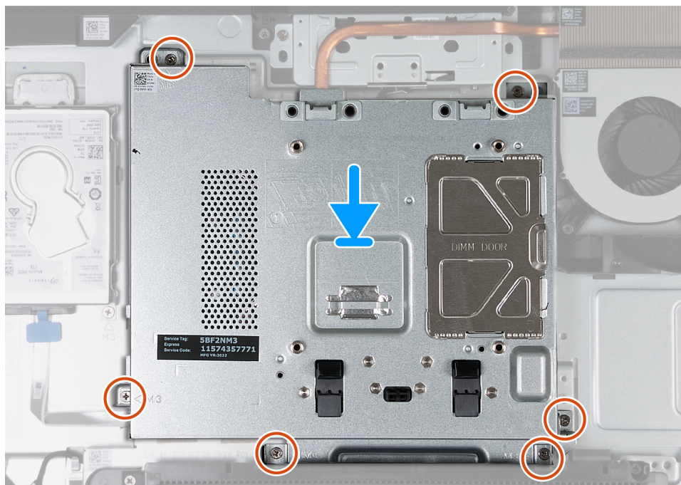
Figure 26. Installing the system-board shield
