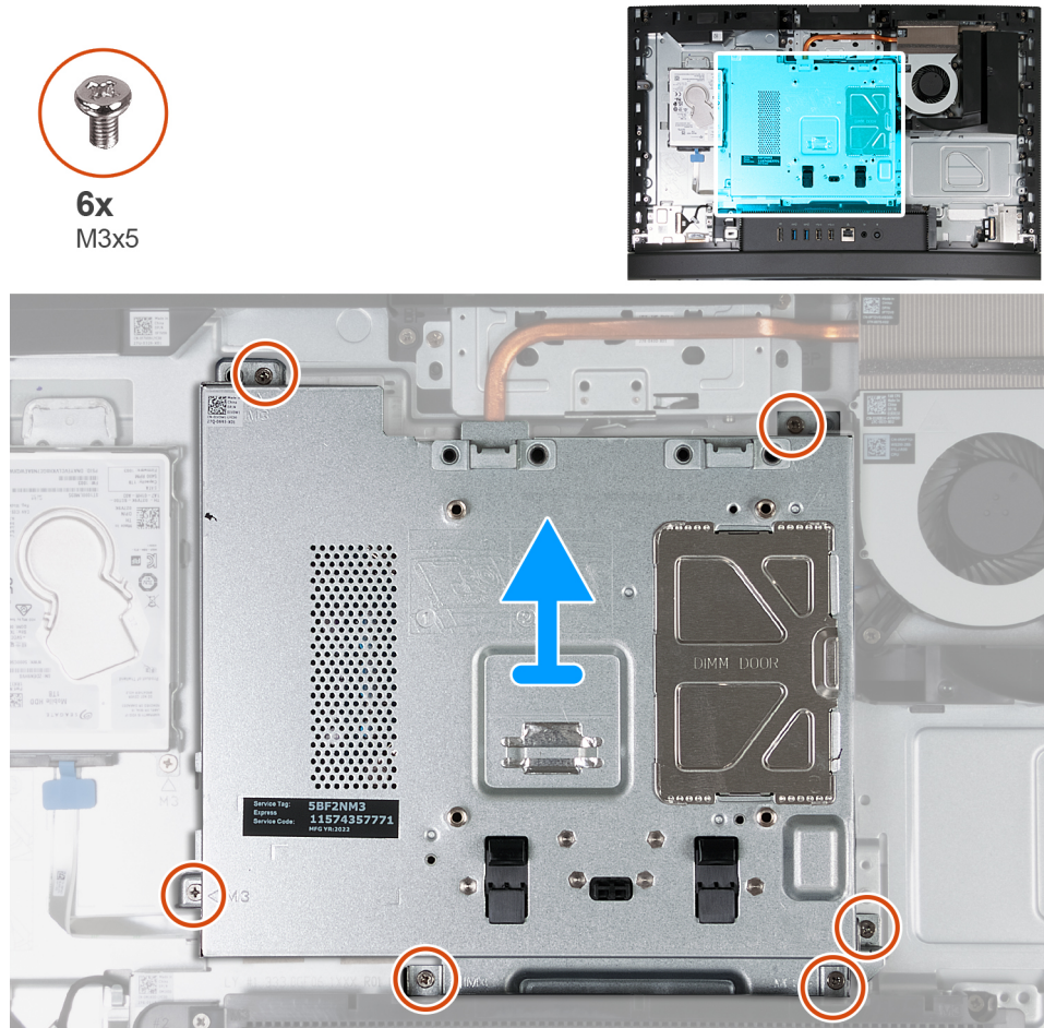
Figure 25. Removing the system-board shield
