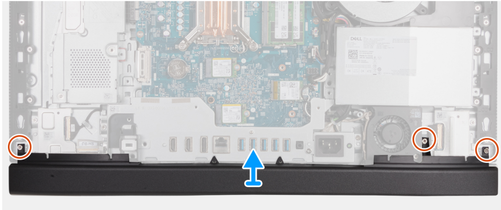
Figure 43. Removing the bottom cover
