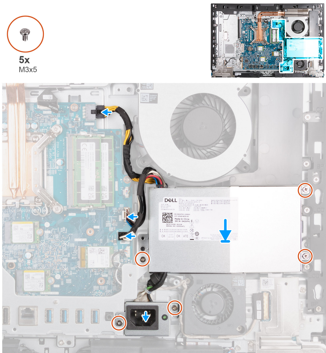
Figure 50. Installing the power-supply unit
