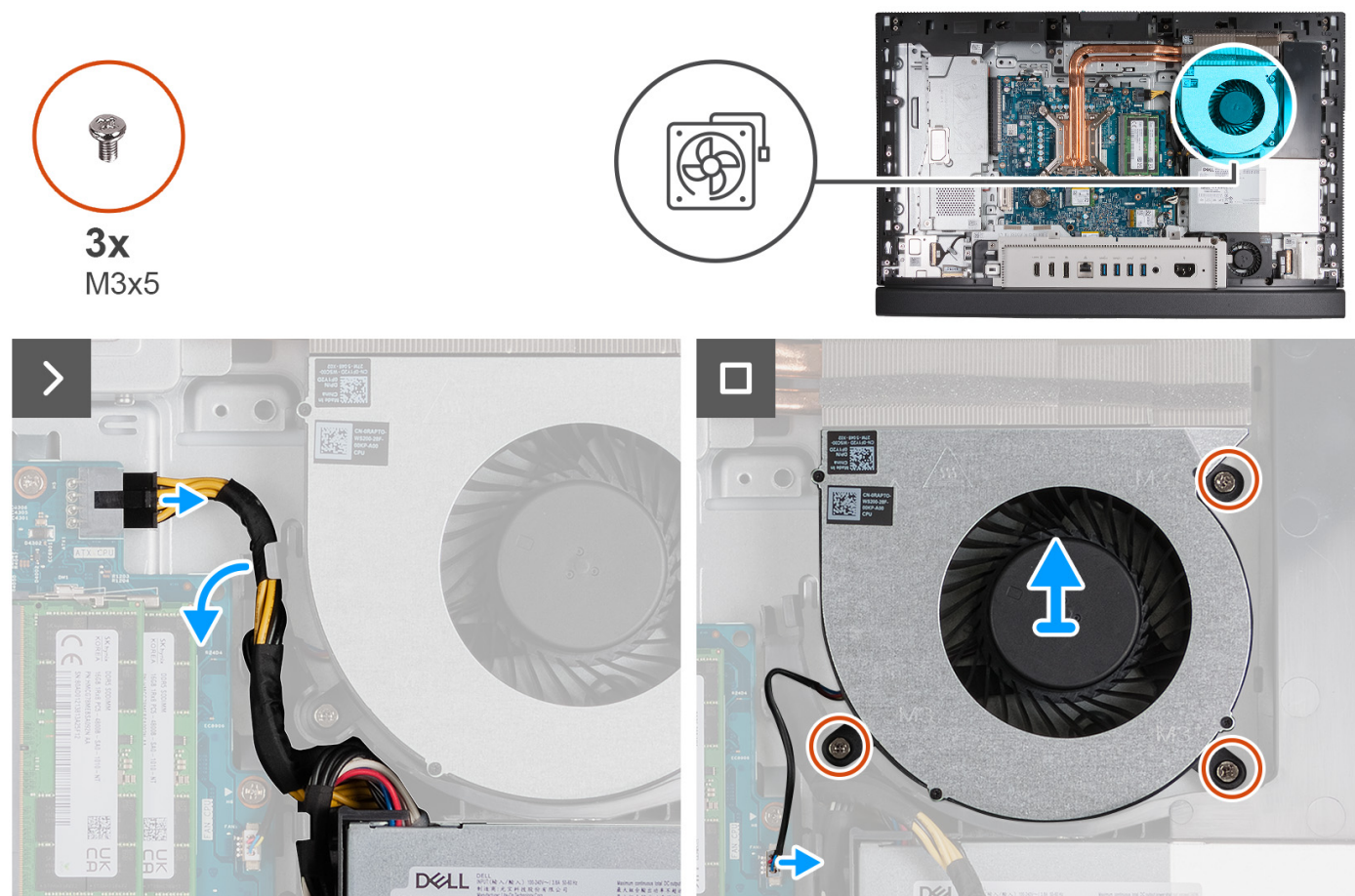
Figure 47. Removing the fan
