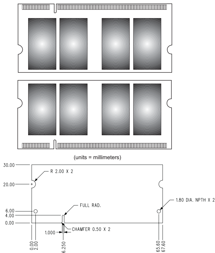
Figure 1: KVR400D2S3/256 200-Pin SODIMM
